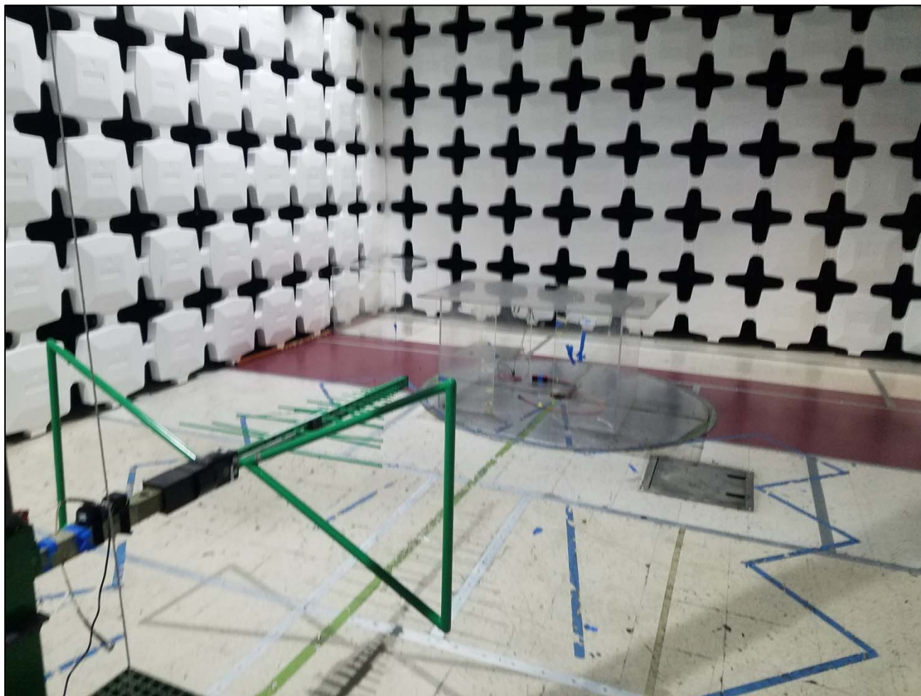
REE 30MHz - 1GHz Setup
