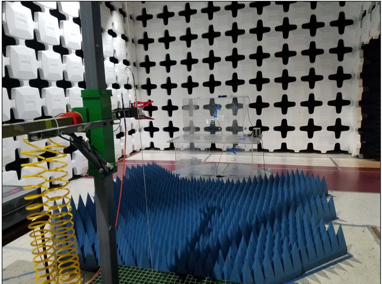
RSE Above 1GHz Setup
