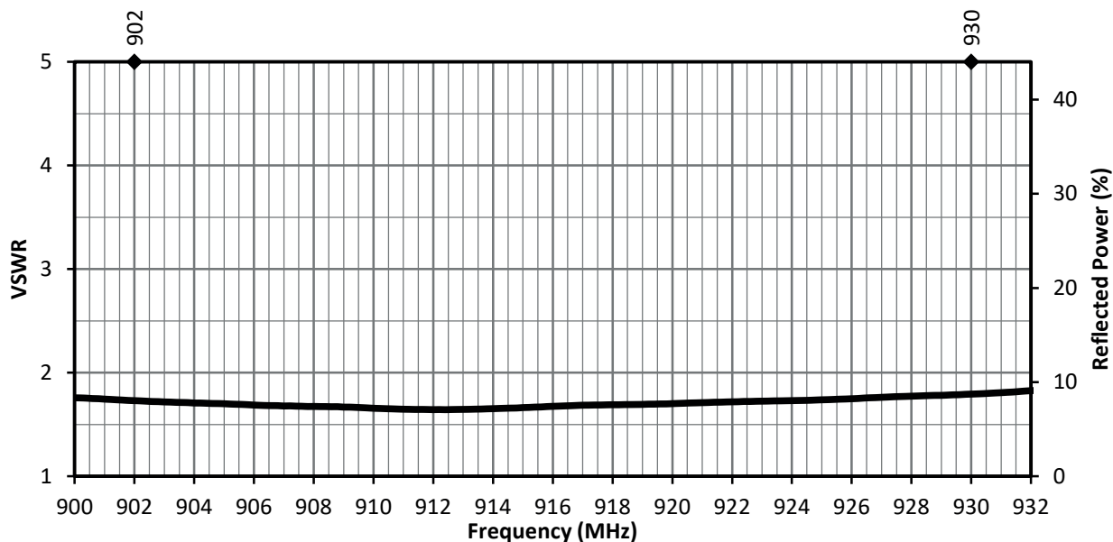
Figure 3. ANT-916-CW-RCL VSWR
