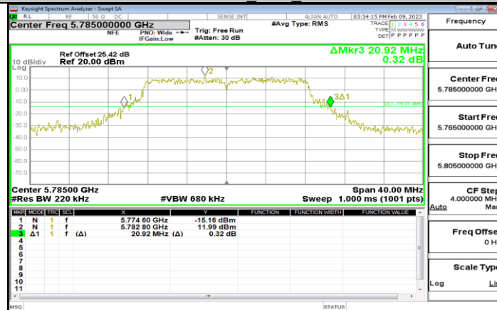
11A-CDD Ant1 5785
