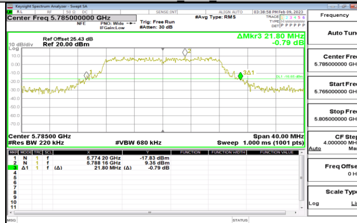
11A-CDD Ant3 5785
