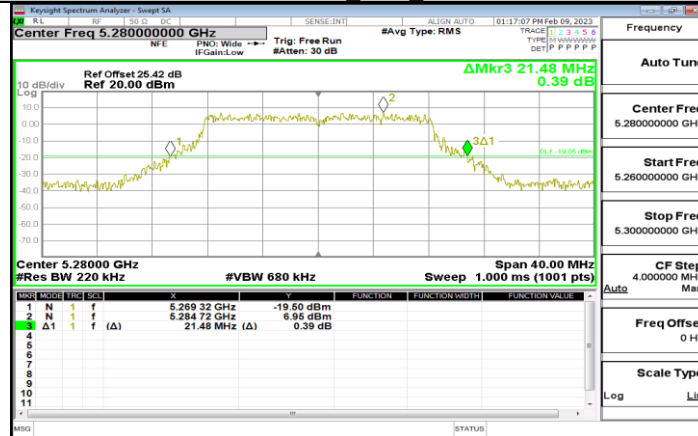
11A-CDD Ant1 5280
