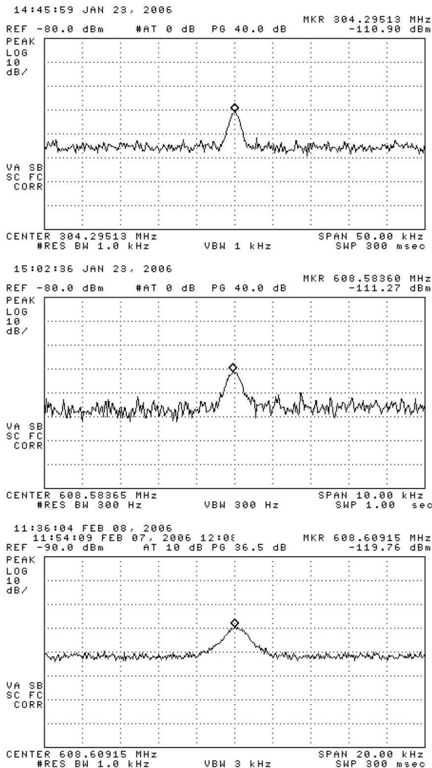
Figure 6.1. Relative receiver emissions, Radiated and Conducted. (top) radiated, (middle) radiated, (bottom) conducted
