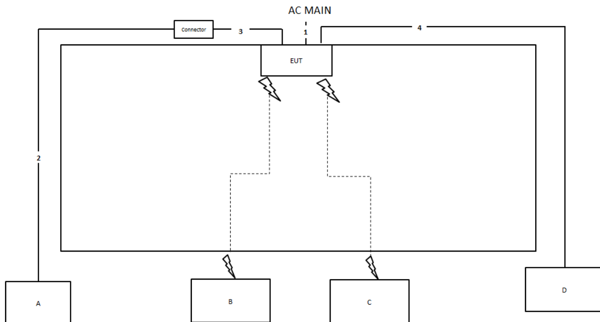
Test Setup Diagram - Radiated Test < 1GHz / Mode 4
