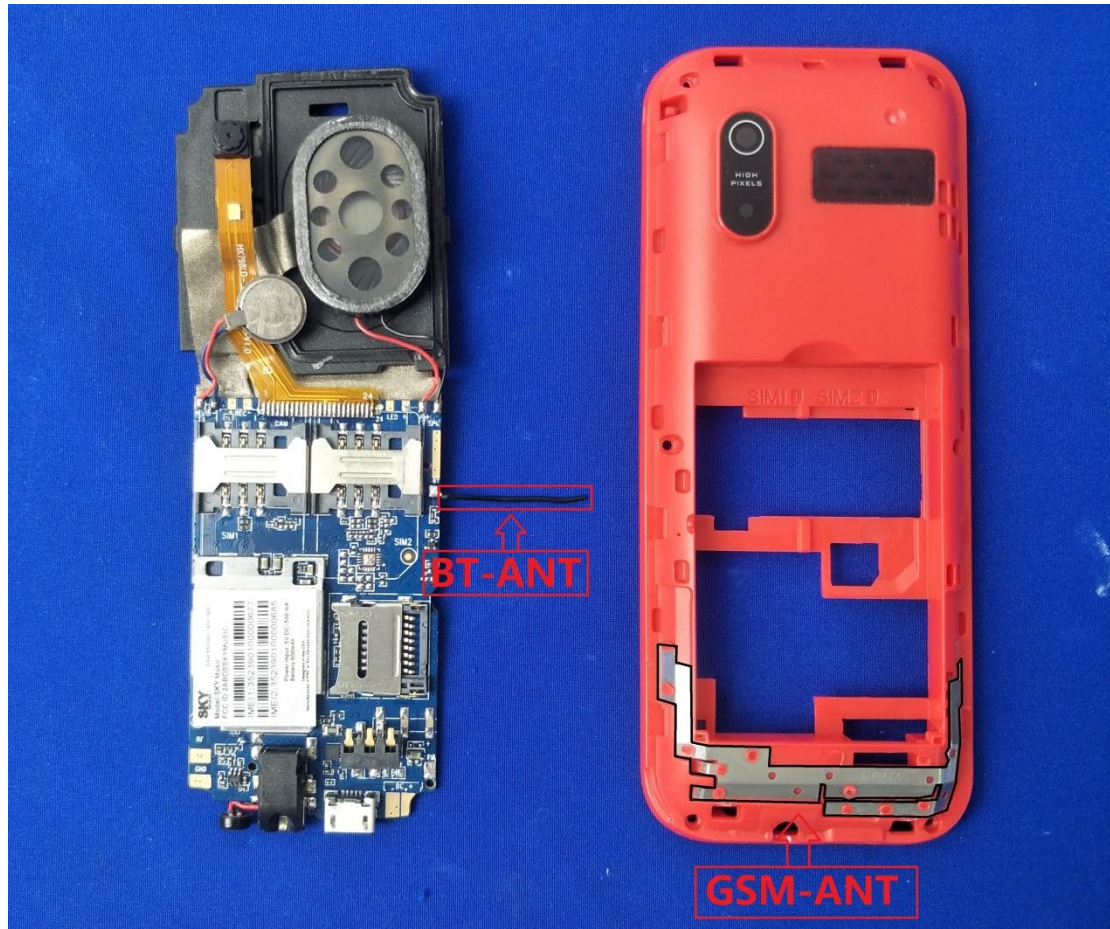
Fig.1 EUT Antenna Locations
