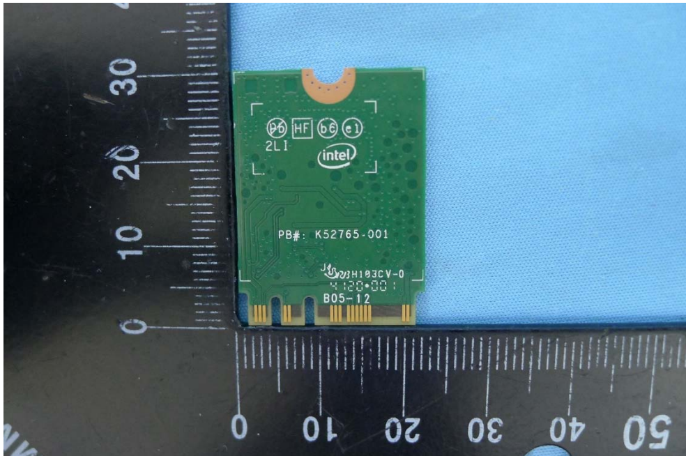
(51) EUT Photo
