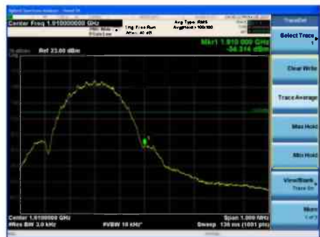
LTE Band 2 1.4MHz QPSK 1RB CH-High
