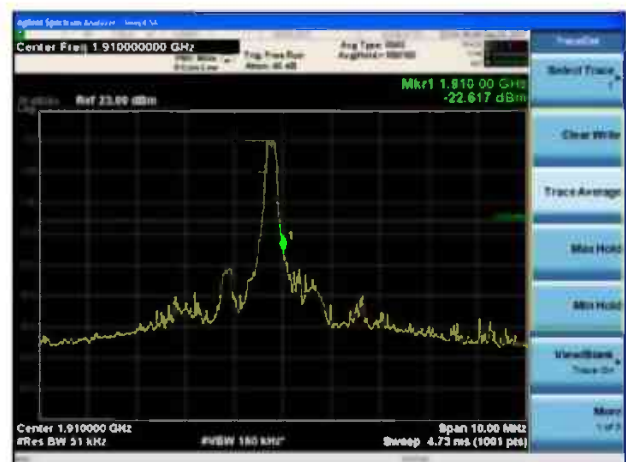
LTE Band 2 1.4MHz QPSK 1RB CH-High
