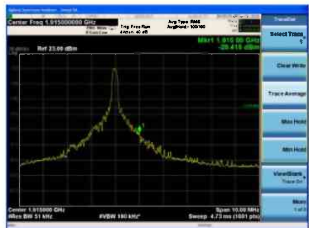
LTE Band 25 15MHz QPSK 1RB CH-High
