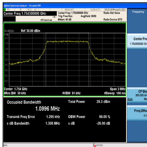
Band4-1.4MHz-QPSK-20393-6RB#0-1.0996
