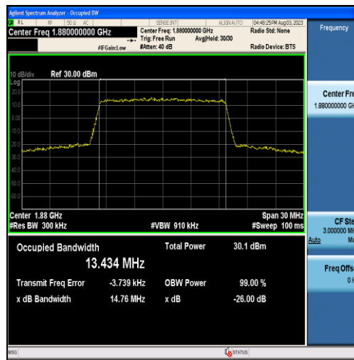
Band2-15MHz-QPSK-18900-75RB#0-13.434
