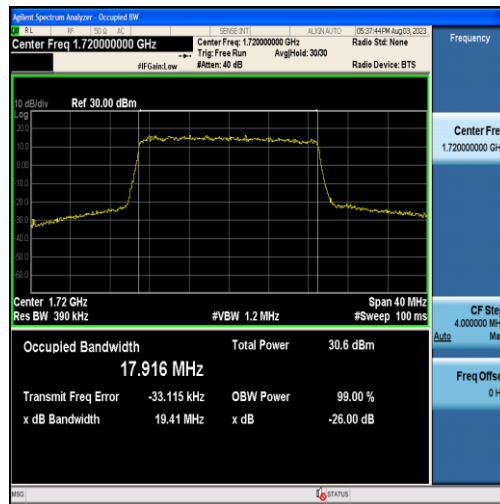
Band4-20MHz-QPSK-20050-100RB#0-17.916
