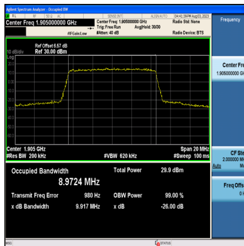
Band2-10MHz-QPSK-19150-50RB#0-8.9724
