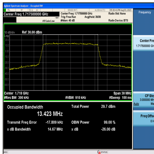
Band4-15MHz-16QAM-20025-75RB#0-13.423
