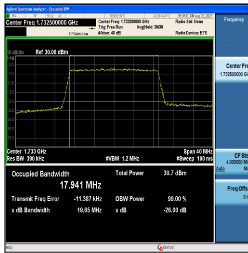
Band4-20MHz-QPSK-20175-100RB#0-17.941
