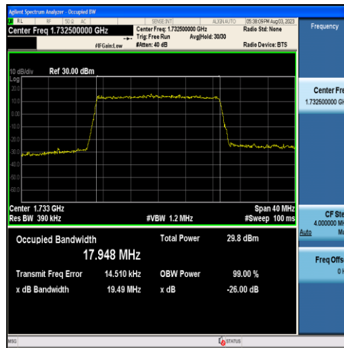
Band4-20MHz-16QAM-20175-100RB#0-17.948
