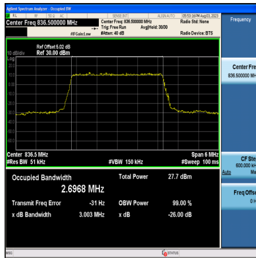
Band5-3MHz-16QAM-20525-15RB#0-2.6968
