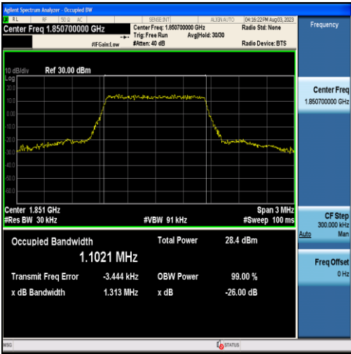
Band2-1.4MHz-16QAM-18607-6RB#0-1.1021
