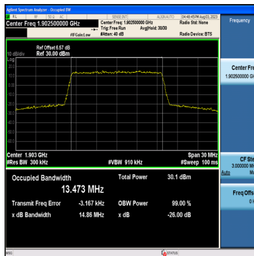
Band2-15MHz-QPSK-19125-75RB#0-13.473
