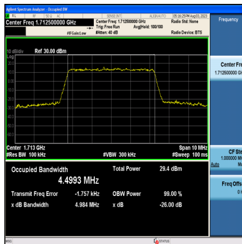
Band4-5MHz-16QAM-19975-25RB#0-4.4993
