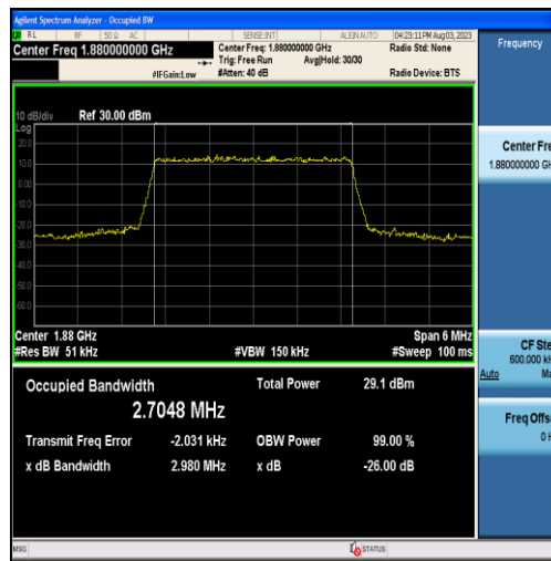
Band2-3MHz-QPSK-18900-15RB#0-2.7048
