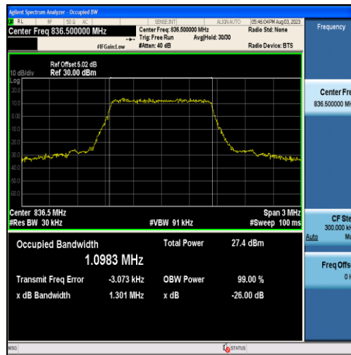
Band5-1.4MHz-16QAM-20525-6RB#0-1.0983
