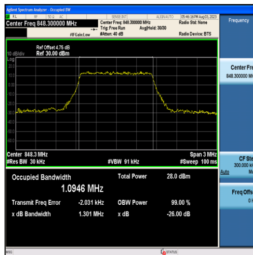
Band5-1.4MHz-QPSK-20643-6RB#0-1.0946
