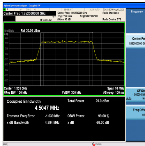
Band2-5MHz-16QAM-18625-25RB#0-4.5047
