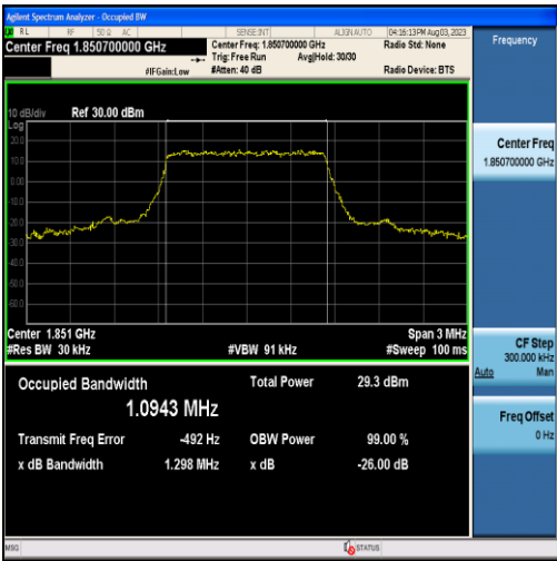
Band2-1.4MHz-QPSK-18607-6RB#0-1.0943
