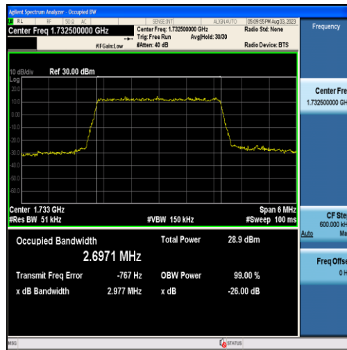
Band4-3MHz-16QAM-20175-15RB#0-2.6971
