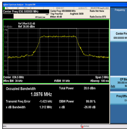
Band5-1.4MHz-QPSK-20525-6RB#0-1.0976
