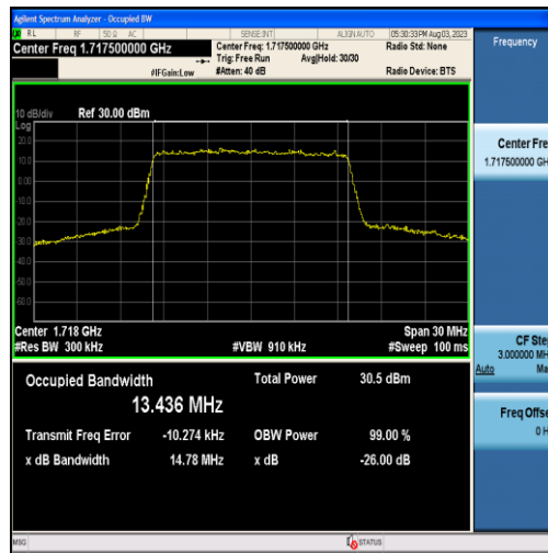
Band4-15MHz-QPSK-20025-75RB#0-13.436
