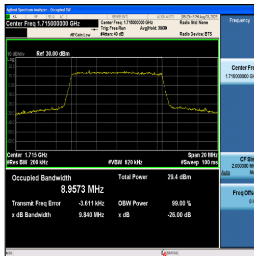
Band4-10MHz-16QAM-20000-50RB#0-8.9573
