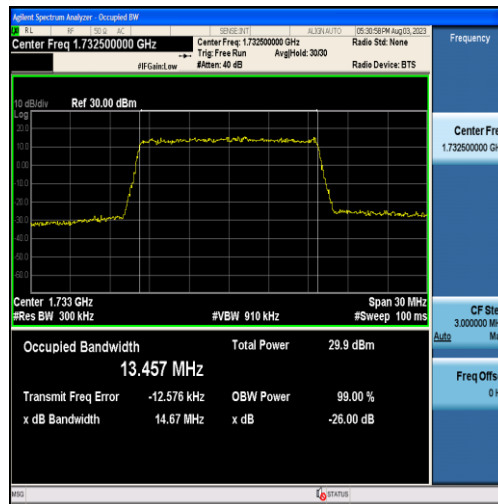
Band4-15MHz-16QAM-20175-75RB#0-13.457
