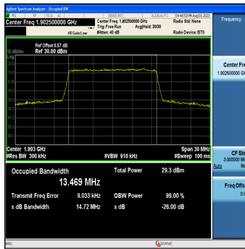
Band2-15MHz-16QAM-19125-75RB#0-13.469
