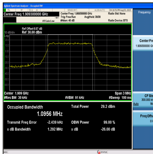
Band2-1.4MHz-QPSK-19193-6RB#0-1.0956
