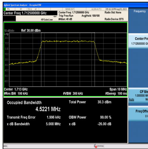
Band4-5MHz-QPSK-19975-25RB#0-4.5221
