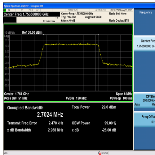
Band4-3MHz-QPSK-20385-15RB#0-2.7024
