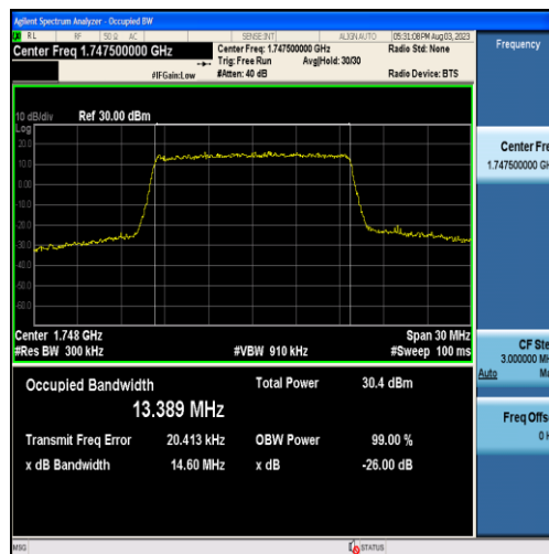
Band4-15MHz-QPSK-20325-75RB#0-13.389
