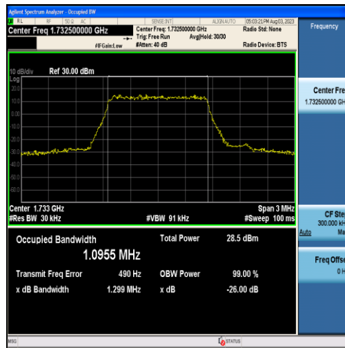
Band4-1.4MHz-16QAM-20175-6RB#0-1.0955
