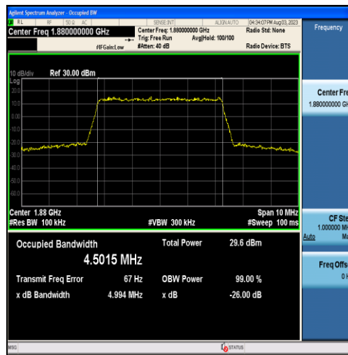
Band2-5MHz-QPSK-18900-25RB#0-4.5015
