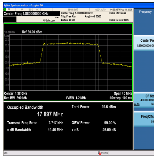
Band2-20MHz-16QAM-18900-100RB#0-17.897
