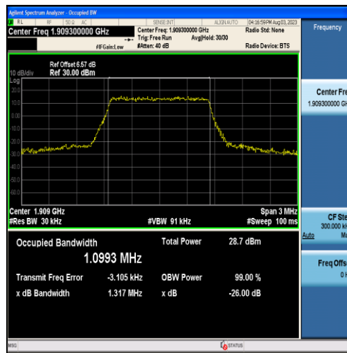
Band2-1.4MHz-16QAM-19193-6RB#0-1.0993
