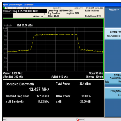
Band2-15MHz-16QAM-18675-75RB#0-13.437
