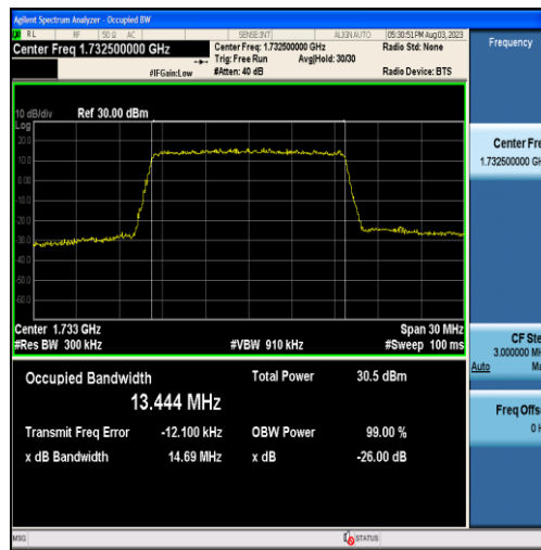
Band4-15MHz-QPSK-20175-75RB#0-13.444
