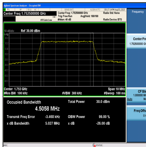
Band4-5MHz-QPSK-20375-25RB#0-4.5058
