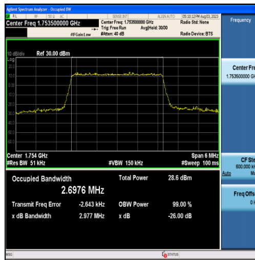
Band4-3MHz-16QAM-20385-15RB#0-2.6976
