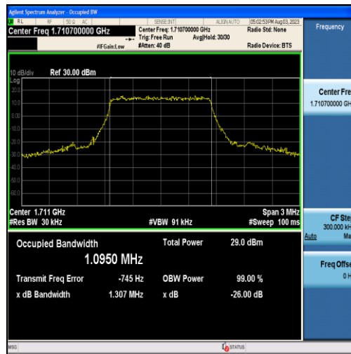
Band4-1.4MHz-QPSK-19957-6RB#0-1.0950
