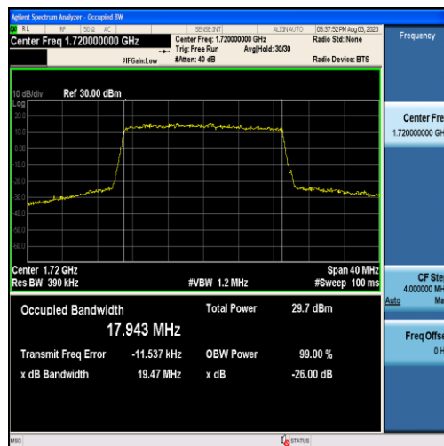
Band4-20MHz-16QAM-20050-100RB#0-17.943
