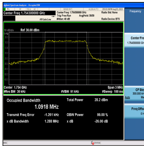
Band4-1.4MHz-16QAM-20393-6RB#0-1.0918
