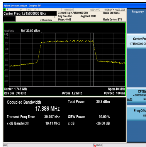
Band4-20MHz-QPSK-20300-100RB#0-17.886
