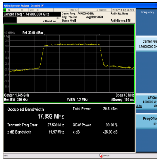
Band4-20MHz-16QAM-20300-100RB#0-17.892
