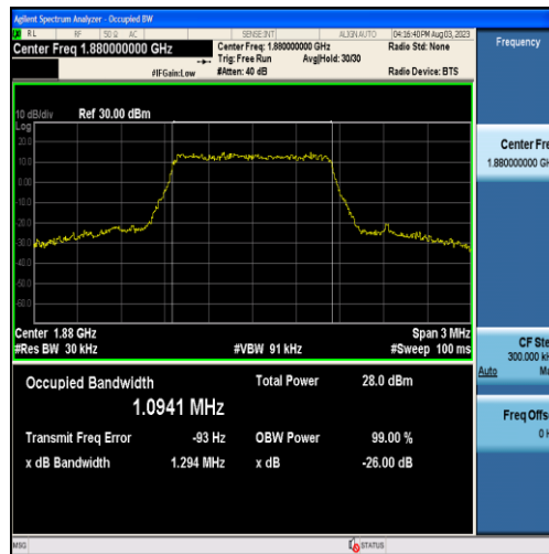
Band2-1.4MHz-16QAM-18900-6RB#0-1.0941
