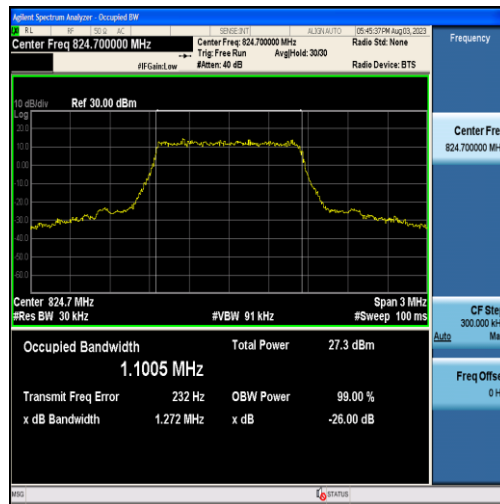
Band5-1.4MHz-QPSK-20407-6RB#0-1.1005
