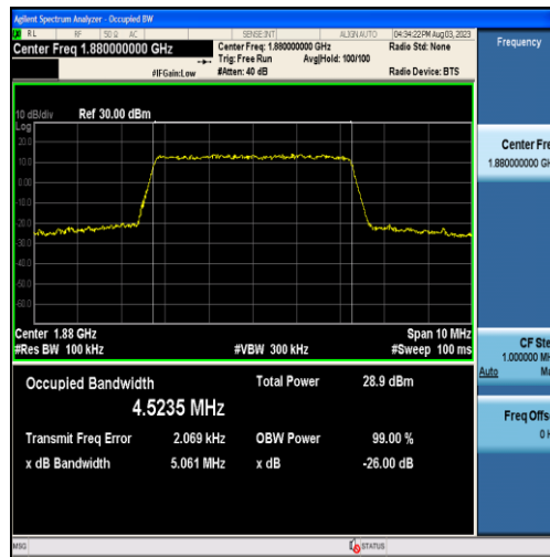
Band2-5MHz-16QAM-18900-25RB#0-4.5235
