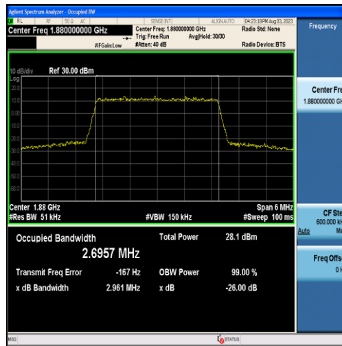
Band2-3MHz-16QAM-18900-15RB#0-2.6957
