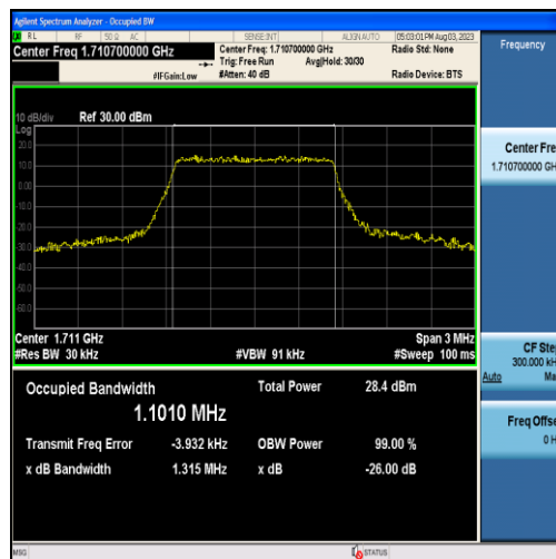
Band4-1.4MHz-16QAM-19957-6RB#0-1.1010
