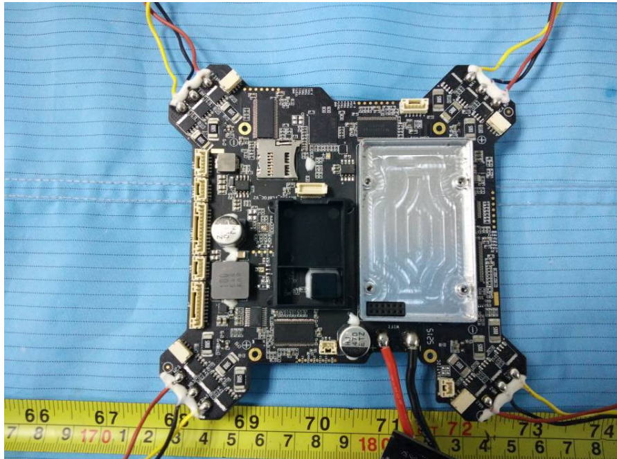
EUT – Main Board 1 Top Shielding off View 4
