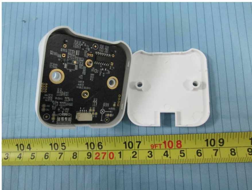
EUT – Camera Cover off View
