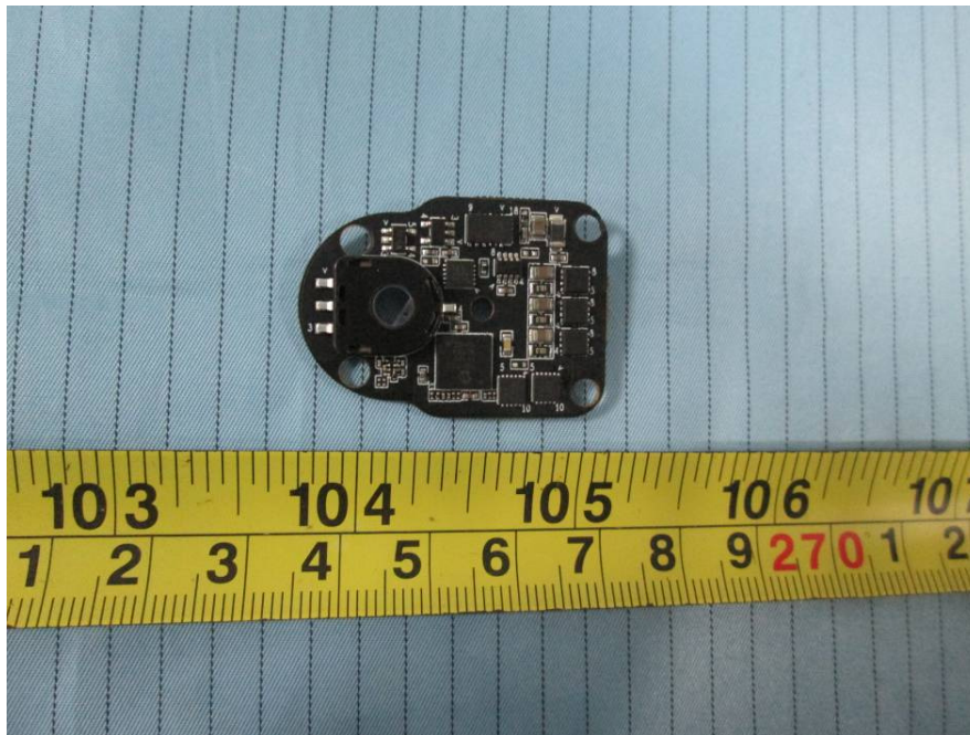
EUT – Vidicon Main Board 3 Bottom View
