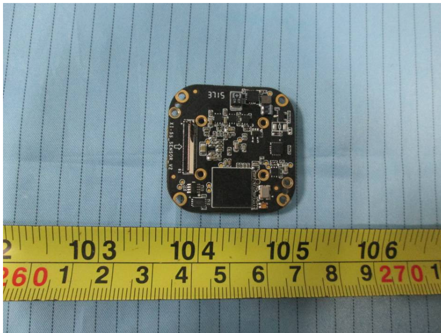
EUT – Vidicon Main Board 2 Top View
