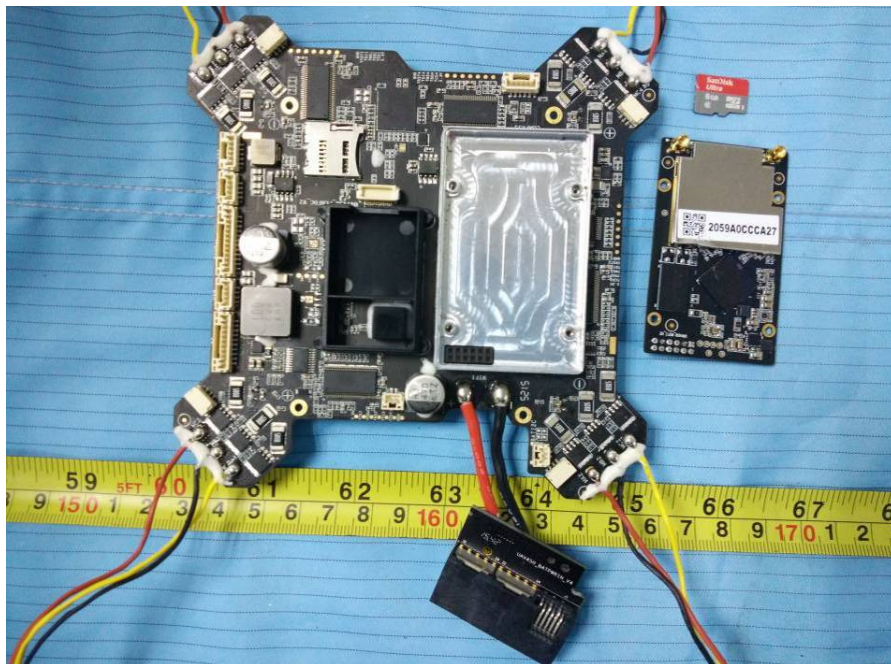
EUT – Main Board 1 Top Shielding off View 3
