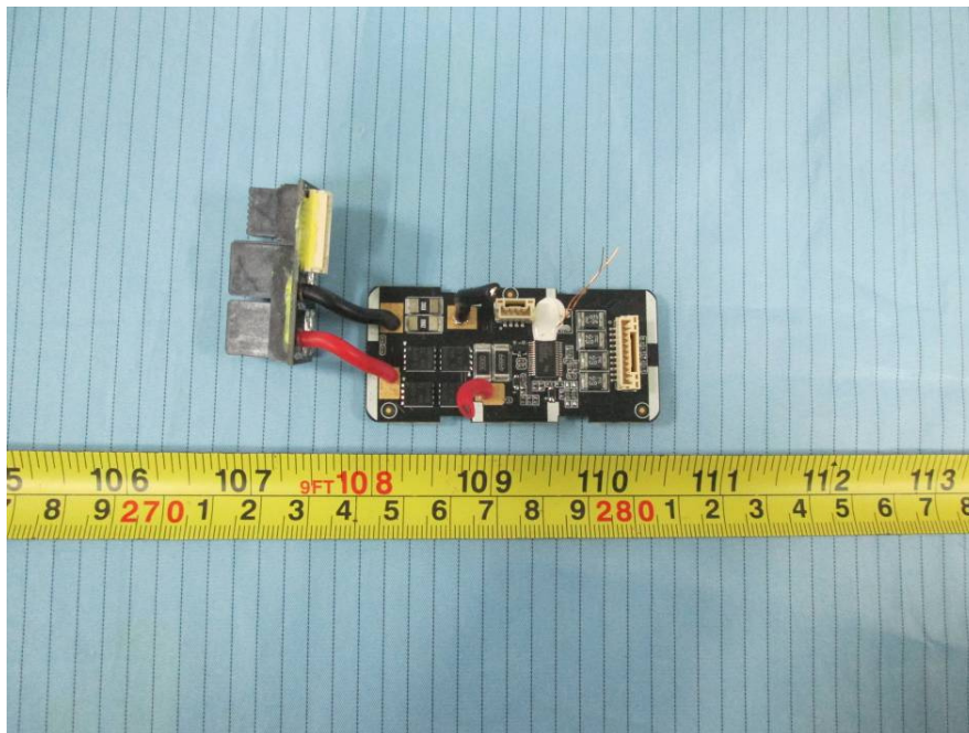
EUT – Battery Main Board 1 Bottom View
