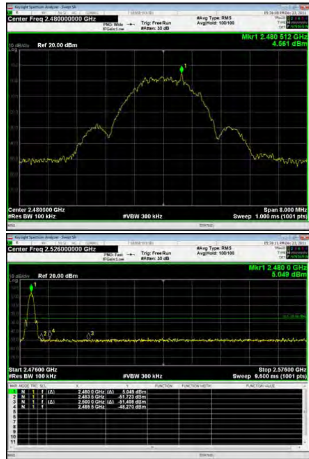
Bluetooth LE (2M), Channel No.: 39
