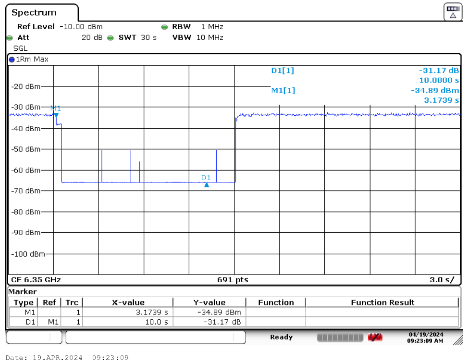
Plot 7-389. Contention Based Protocol Timing Plot (320MHz (UNII Band 6) – Ch. 95 Low)
