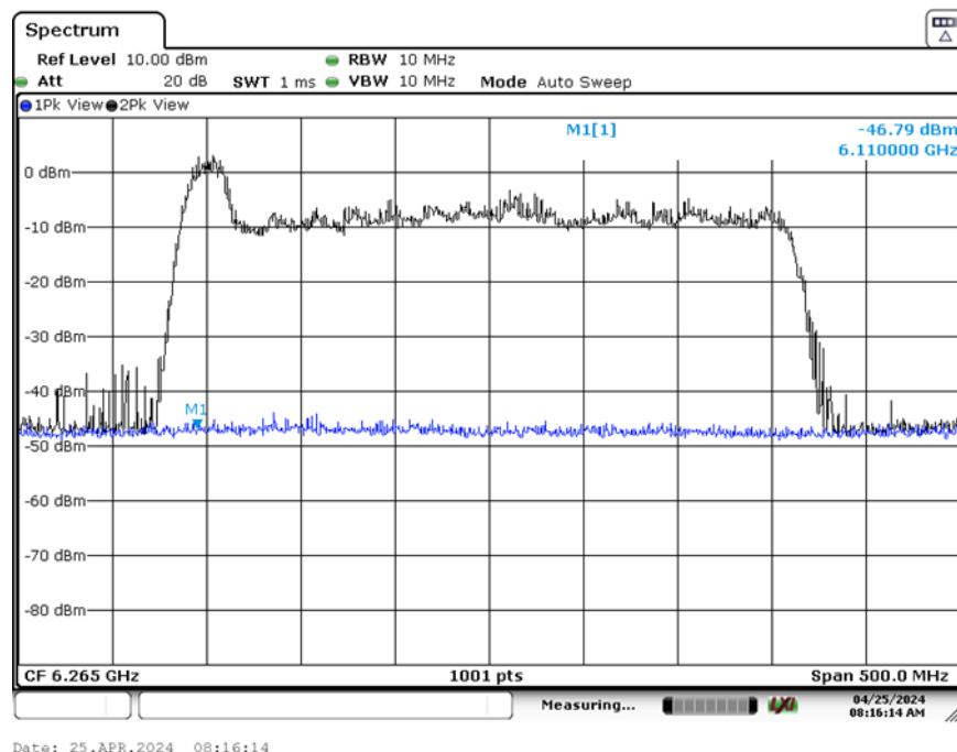
Plot 7-399. CBP 320MHz Channel - Injection Lower Edge – [6110 MHz]
