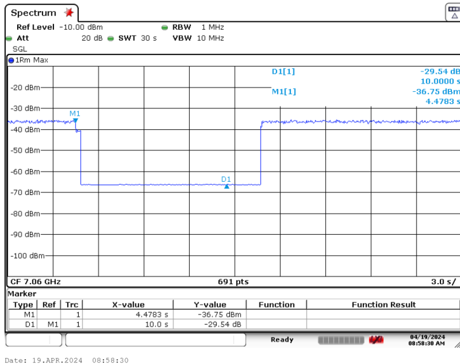
Plot 7 397. Contention Based Protocol Timing Plot (320MHz (UNII Band 8) – Ch. 191 High)
