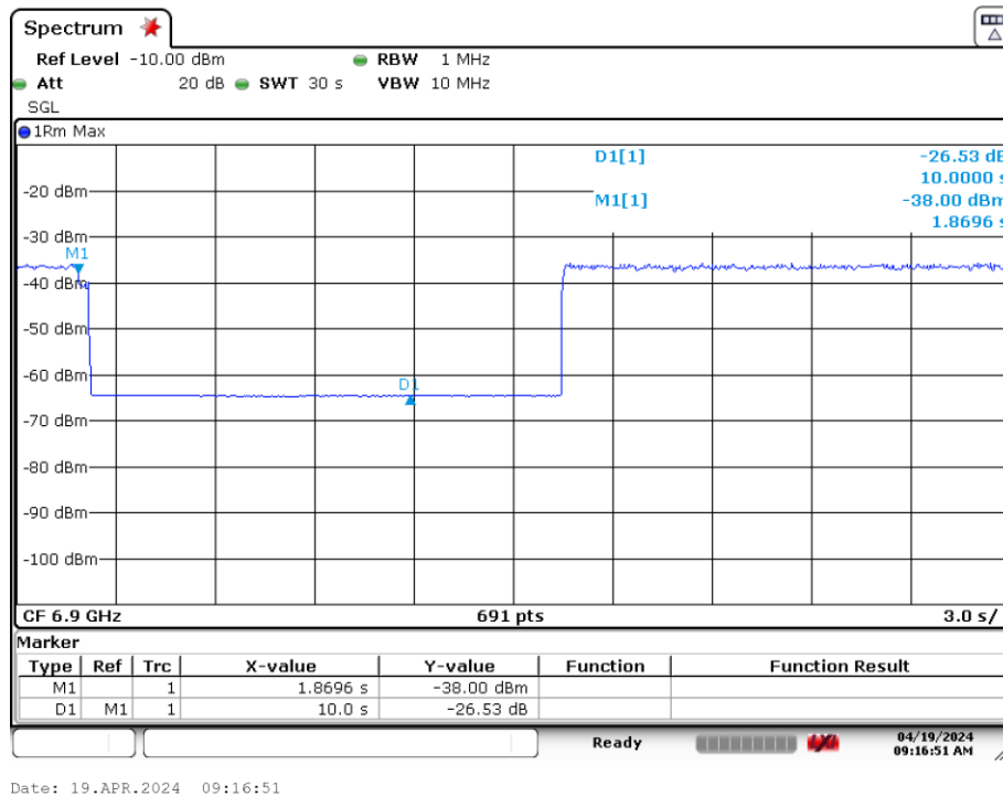
Plot 7-395. Contention Based Protocol Timing Plot (320MHz (UNII Band 7) – Ch. 159 High)
