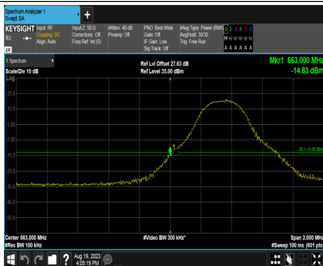
Band71-5MHz-16QAM-133147-1RB#24
