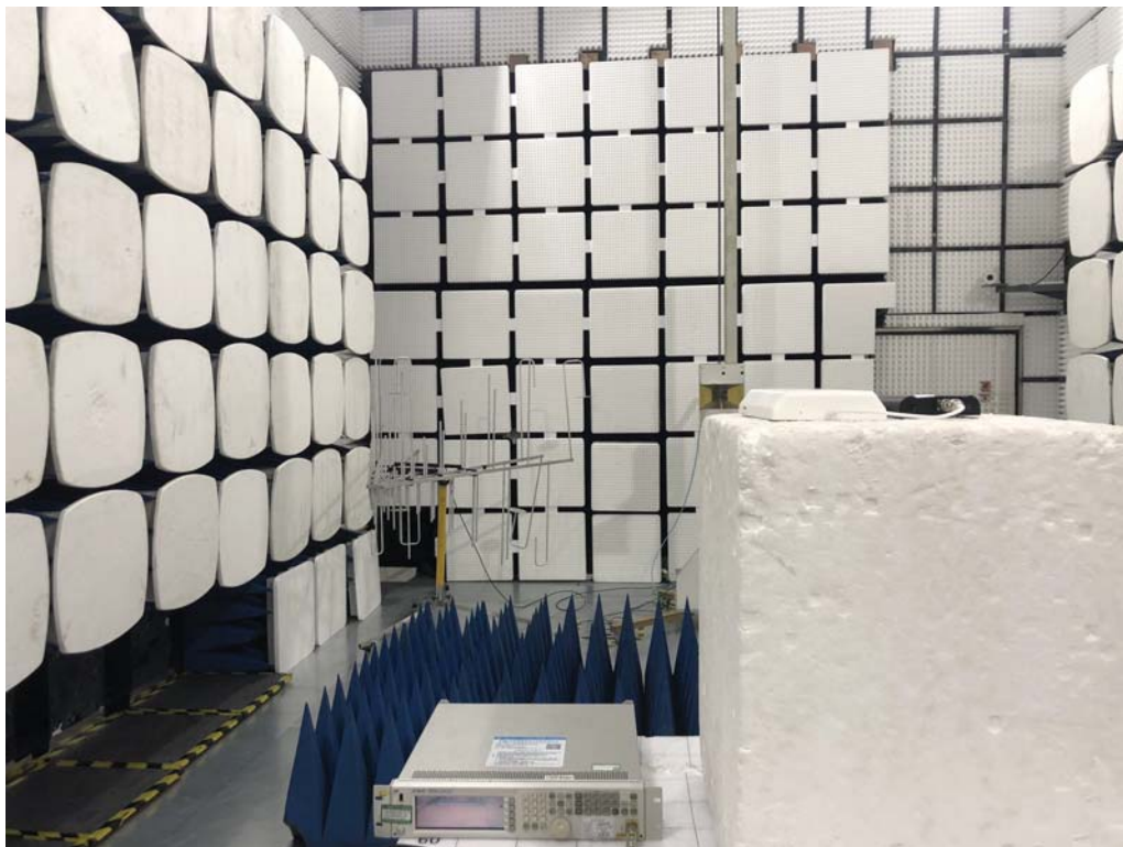
Fig. 6 (Above 1GHz)-SYN-OPA-8D
