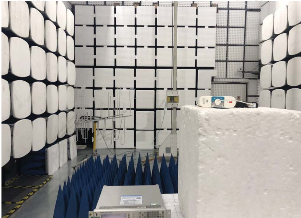
Fig. 5 (Above 1GHz)-SYN-BY-9D
