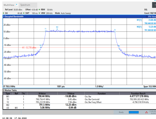
Band14-5MHz-QPSK-23330-25RB#0
