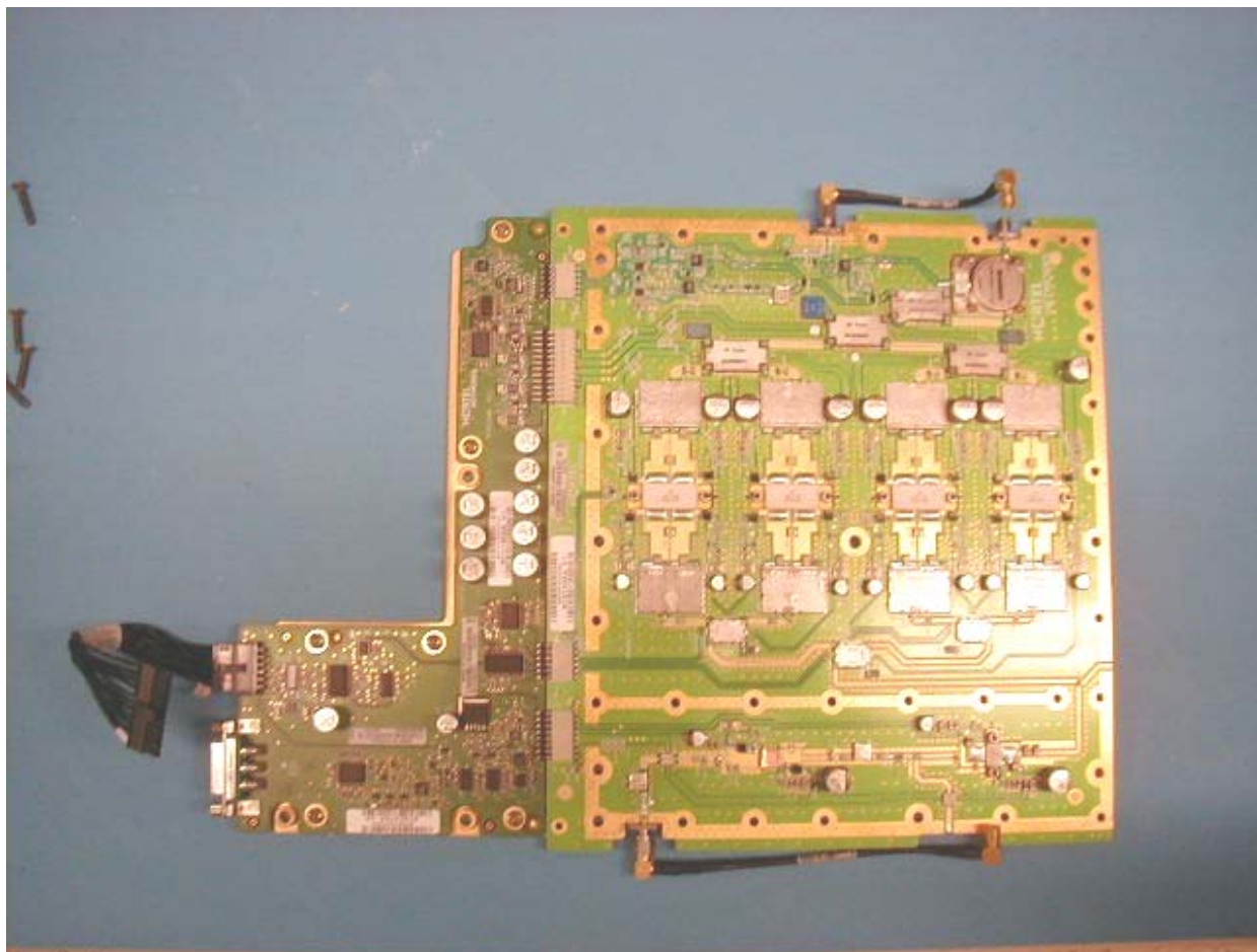
Nortel Networks 800MHz MFRM2 PA Board NTGY33EA Top View
