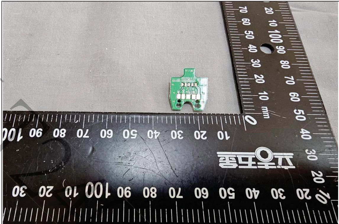
< PCB1-R >
