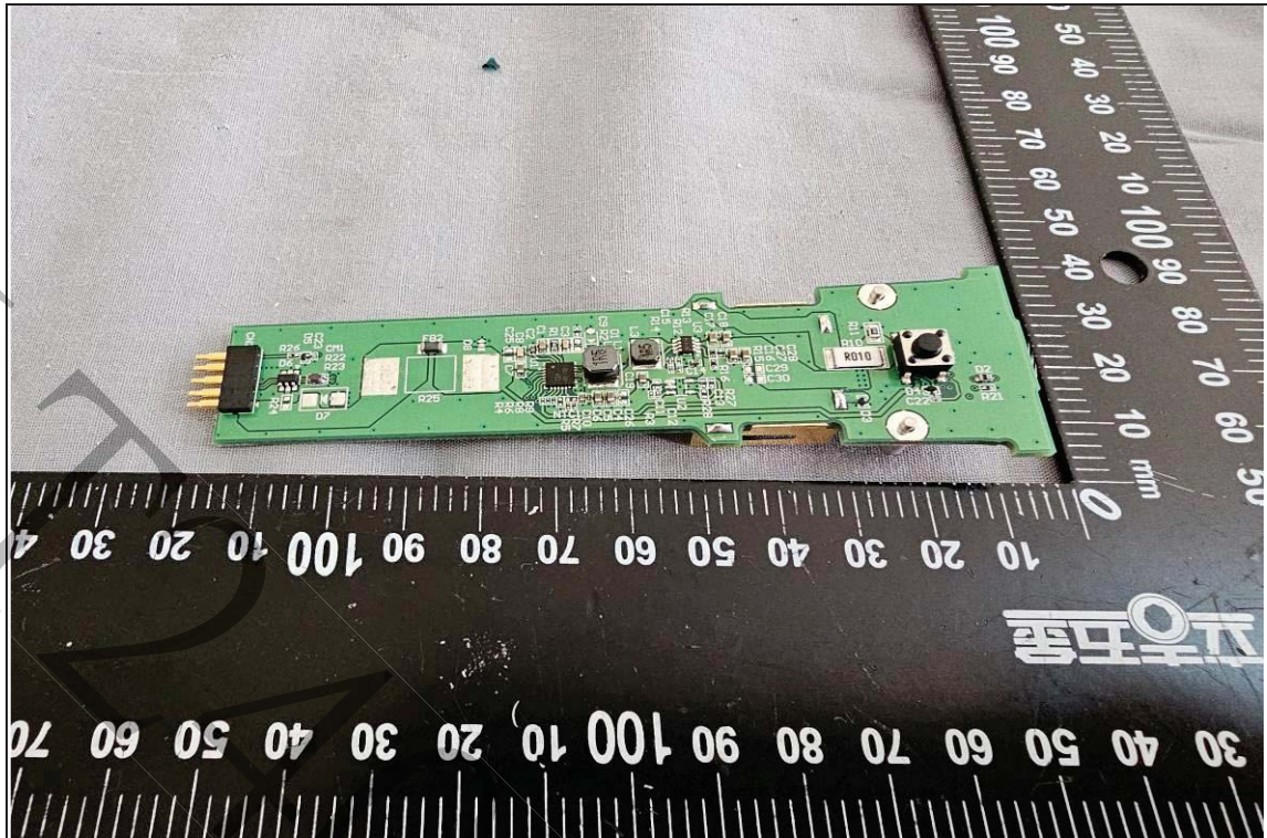
< PCB2-R >
