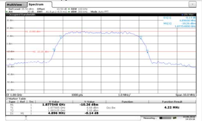
Channel 9400
