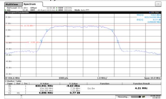
Channel 4183
