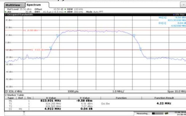
Channel 4132
