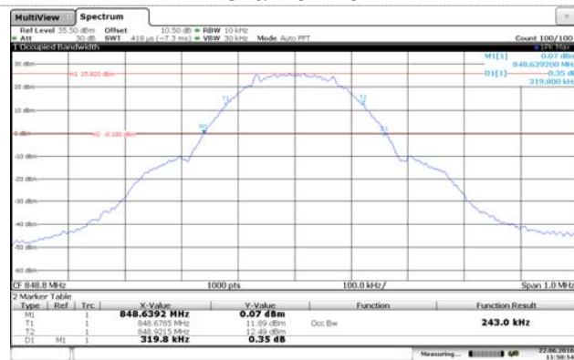
Channel 251
