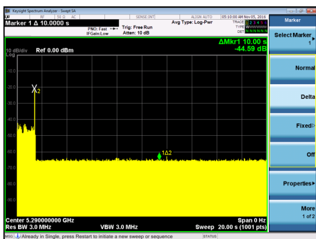
Channel Move Time - 802.11ac-5290MHz (Type0)
