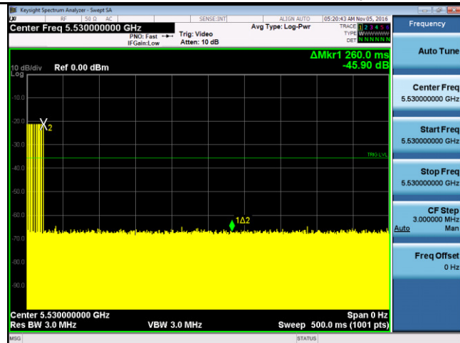
Channel Closing Time - 802.11ac-5530MHz (Type0)
