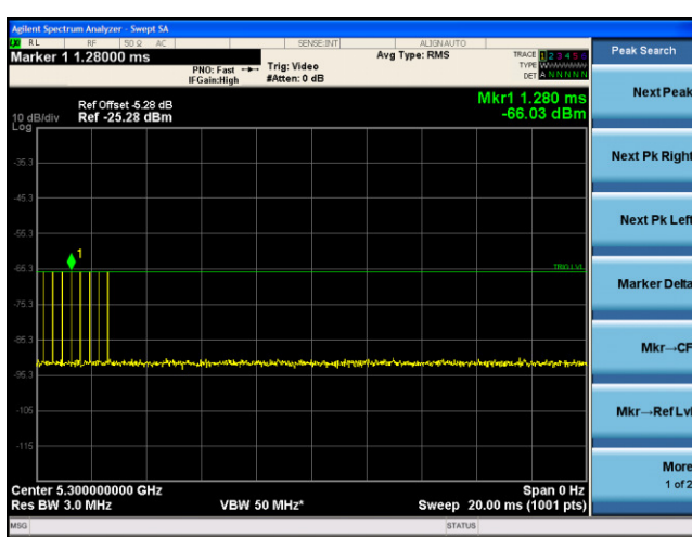
Radar Calibration - Type 6
