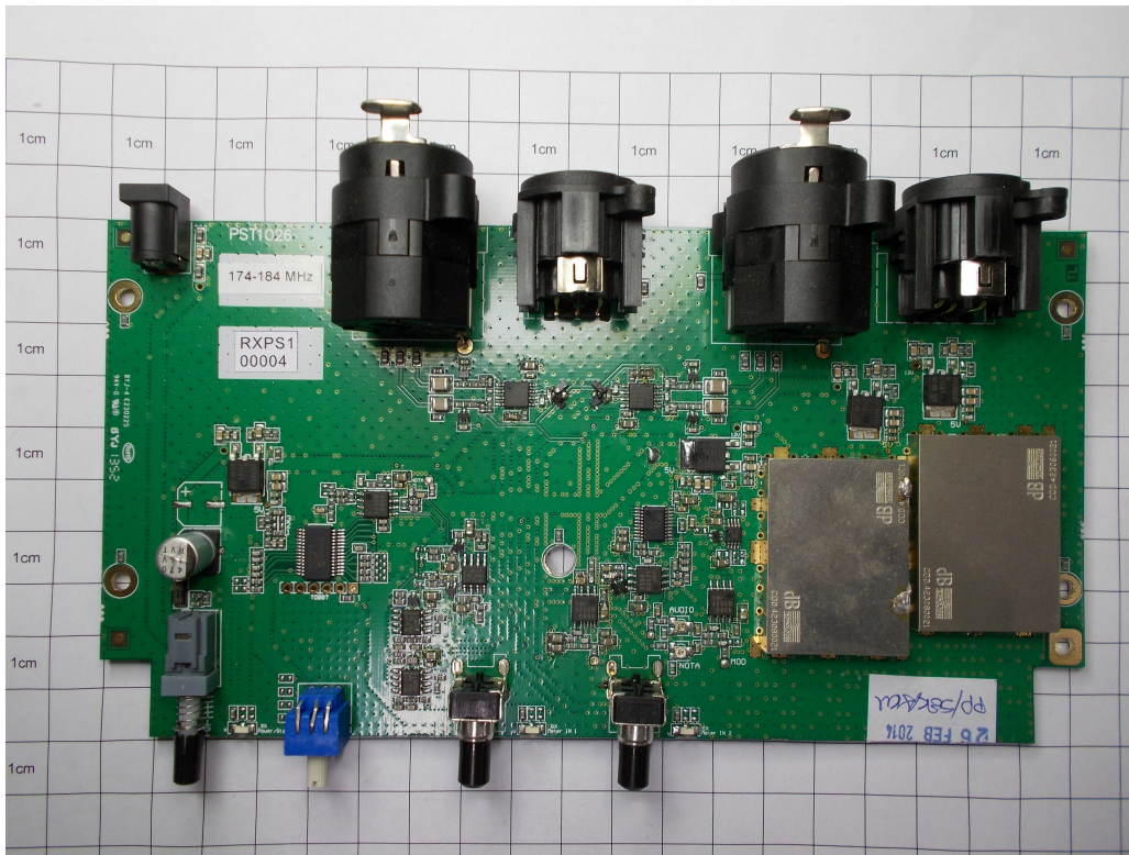
Fig. 1 - FRONT with complete shields
