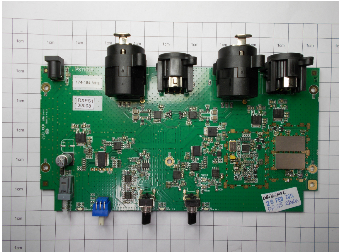
Fig. 3 - FRONT without firsts shields
