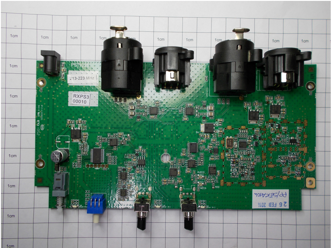
Fig. 5 - FRONT without all shields
