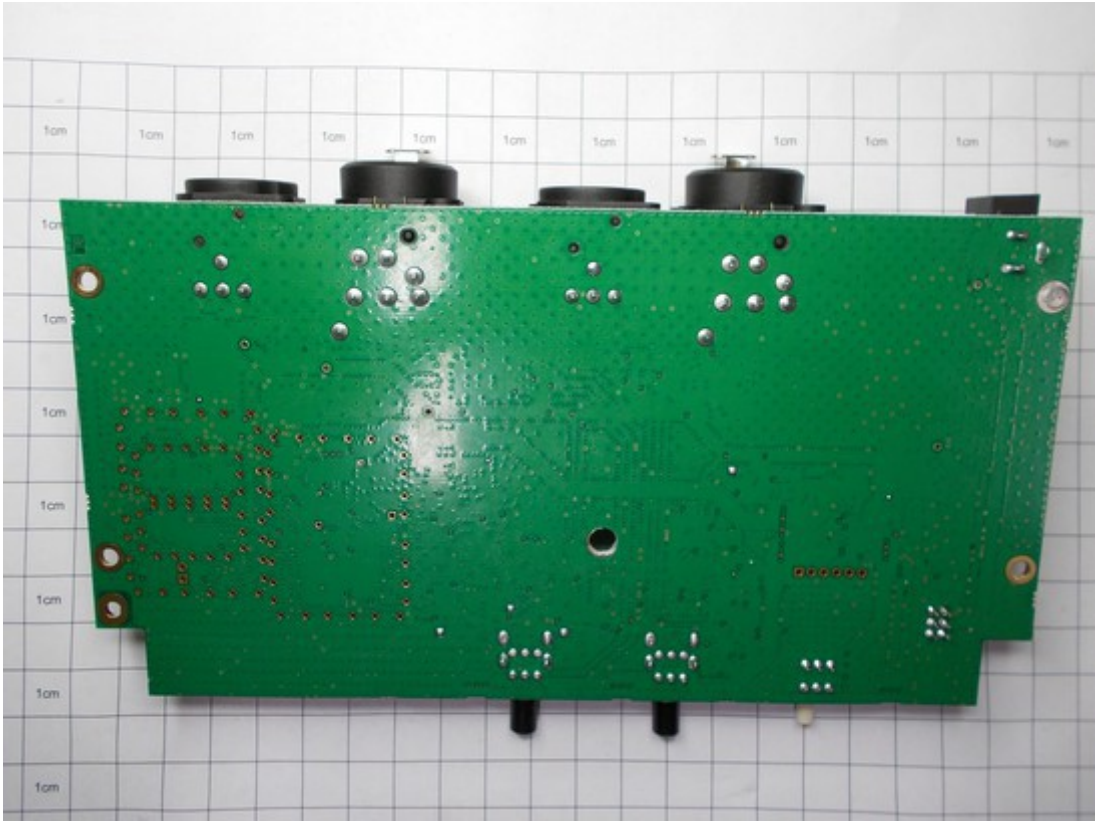
Fig.6 - REAR of fig. 5
