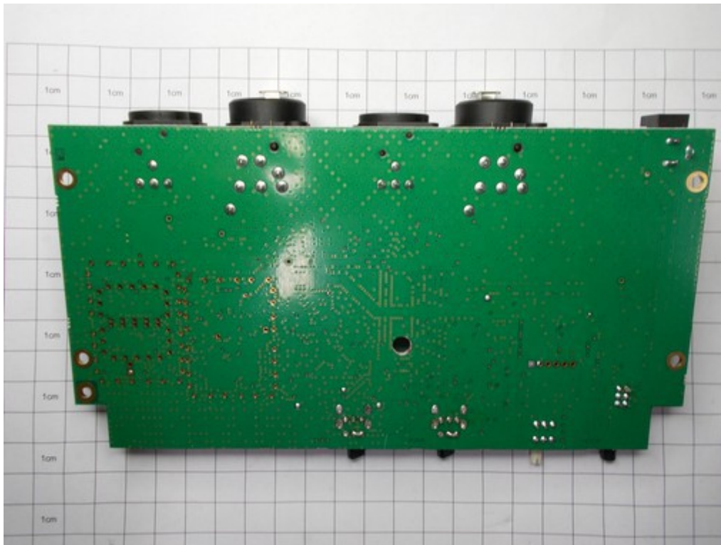
Fig.2 - REAR of fig. 1
