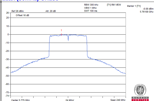
11ax (80MHz) CH155
