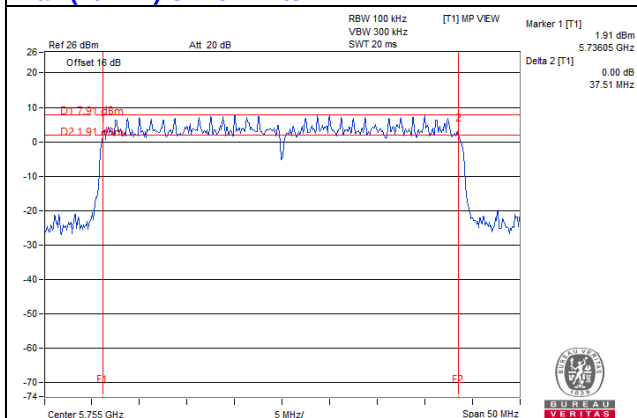
11ax (40MHz) CH151 Ant4
