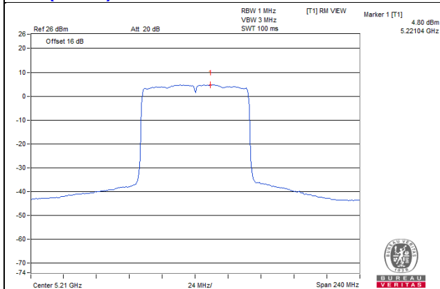
11ax (80MHz) CH42
