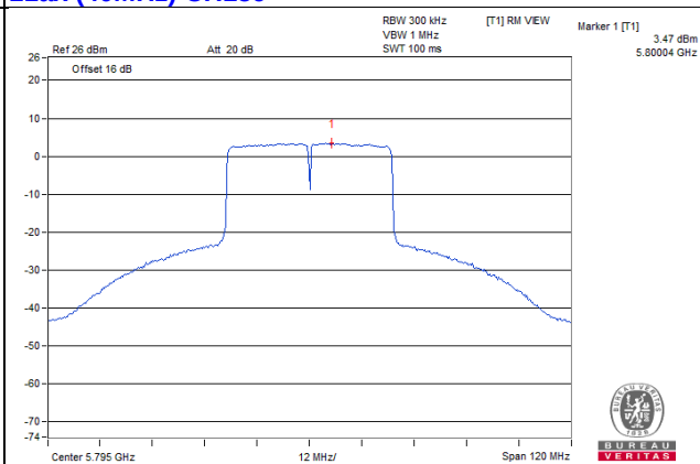
11ax (40MHz) CH159
