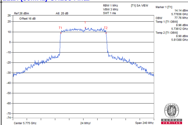
11ax (80MHz) CH155 Ant2
