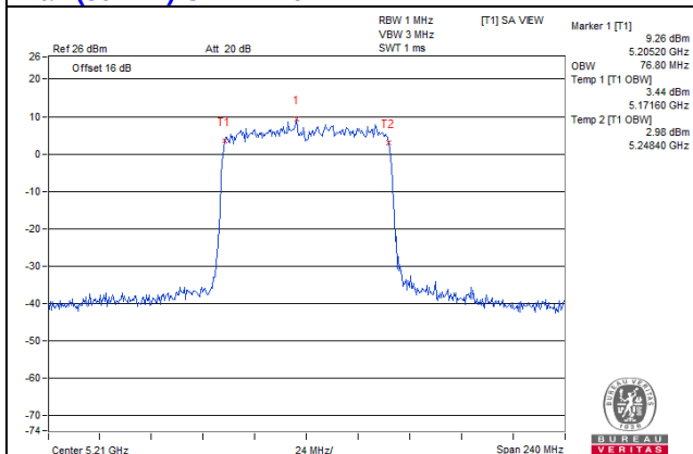
11ax (80MHz) CH42 Ant1
