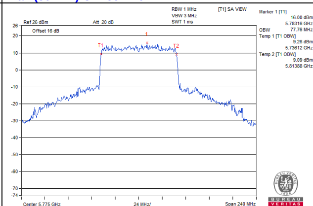
11ax (80MHz) CH155 Ant1
