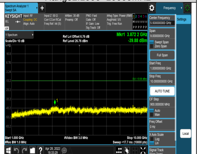
Band17-10MHz-16QAM-23780-1RB#0-
