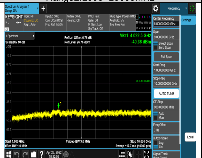
Band17-10MHz-QPSK-23800-1RB#0- Range2:1000~10000MHz
