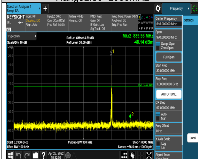
Band17-10MHz-QPSK-23800-1RB#0- Range1:30~1000MHz
