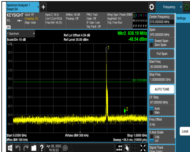
Band17-10MHz-QPSK-23790-1RB#0- Range1:30~1000MHz
