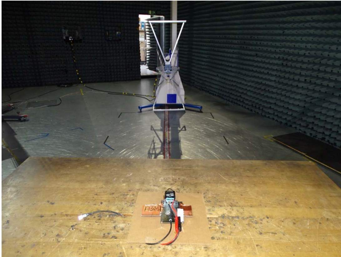
Photo 1: Test setup for radiated measurements (Enclosure, semi-anechoic chamber, 30 MHz to 1 GHz, intentional radiator §15, ANSI C63.10)
