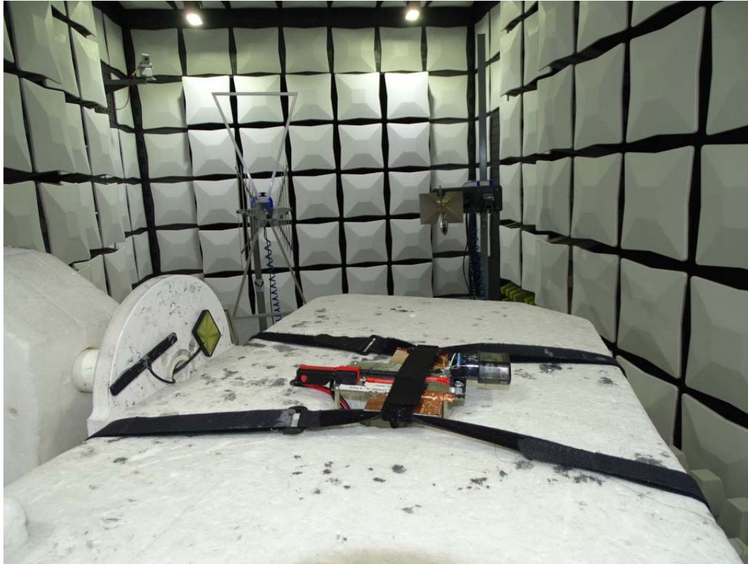
Photo 2: Test setup for radiated measurements (Enclosure, fully-anechoic chamber, 1-26 GHz intentional radiator §15, ANSI C63.10 and 30 MHz – 10/20 GHz, §22/24/27)
