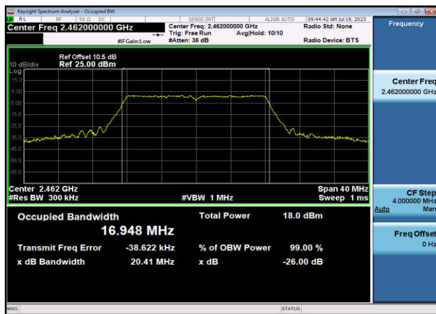
99% Bandwidth-802.11g,2462MHz,Ant1
