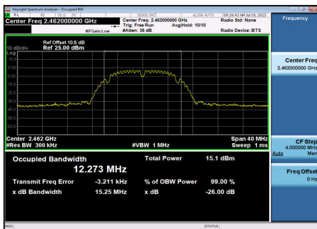
99% Bandwidth-802.11b,2462MHz,Ant1
