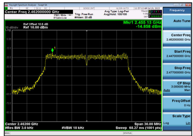
Power spectral density-802.11g ,2462MHz,Ant2
