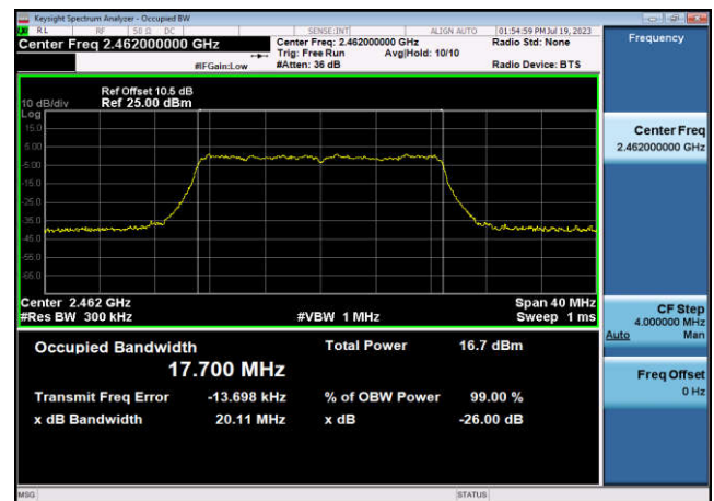
99% Bandwidth-802.11n(HT20),2462MHz ,Ant2
