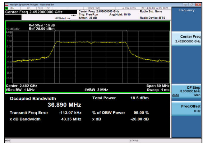
99% Bandwidth-802.11n(HT40),2452MHz ,Ant2
