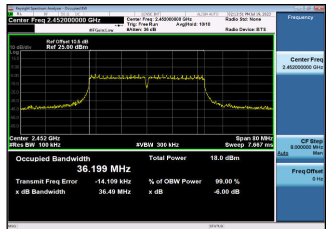
6dB Bandwidth-802.11n(HT40),2452MHz ,Ant2
