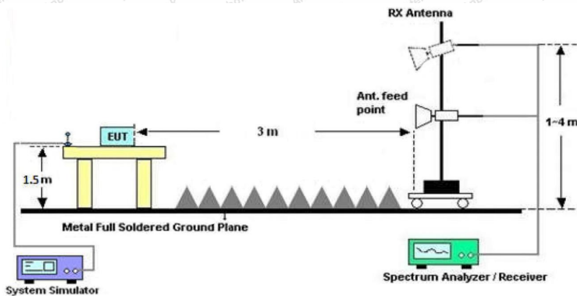
Figure 3. Above 1 GHz
