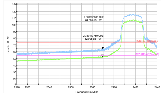
802.11n HT20-Channel 2 Peak+ Average
