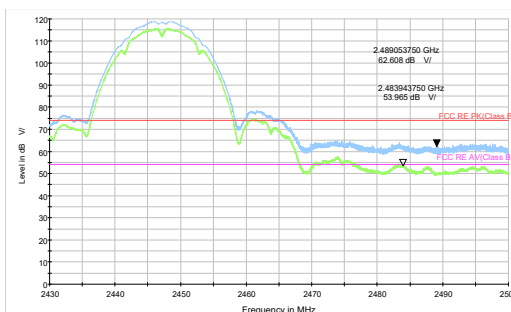
802.11b-Channel 8 Peak+ Average
