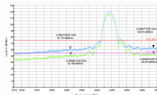
802.11b-Channel 6 Peak+ Average
