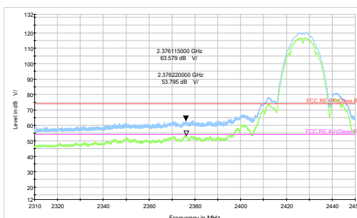
802.11b-Channel 4 Peak+ Average
