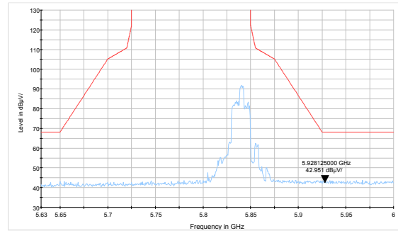
Frequency 5840MHz
