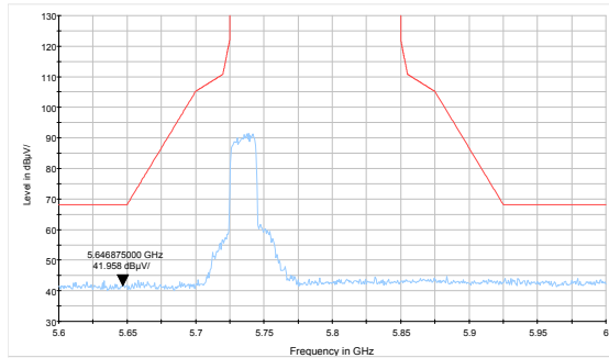
Frequency 5735MHz
