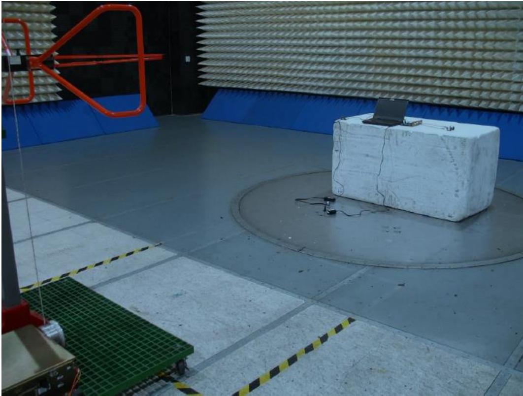
Test Setup Photos; White and Black Antennas
