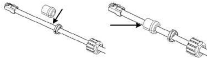
Figure 31: Insert Rubber Gland on Cable
