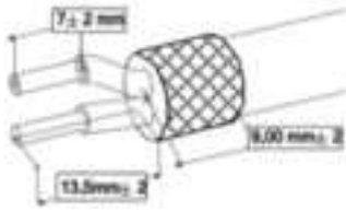
Figure 40: Stripping Dimensions (DC Cable)
