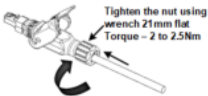
Figure 38: Tighten Gland Nut
