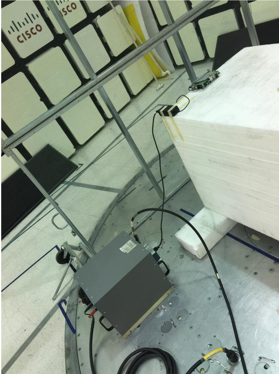
AIR-AP1810W-x-K9 AC Mains Conducted Emissions setup
