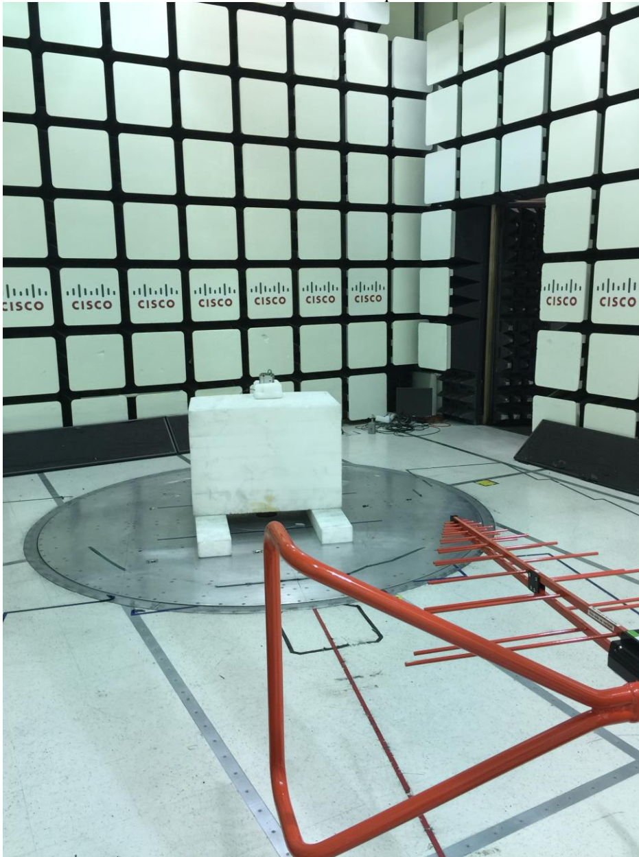
AIR-AP1810W-x-K9 Radiated Emissions setup 30MHz – 1GHz
