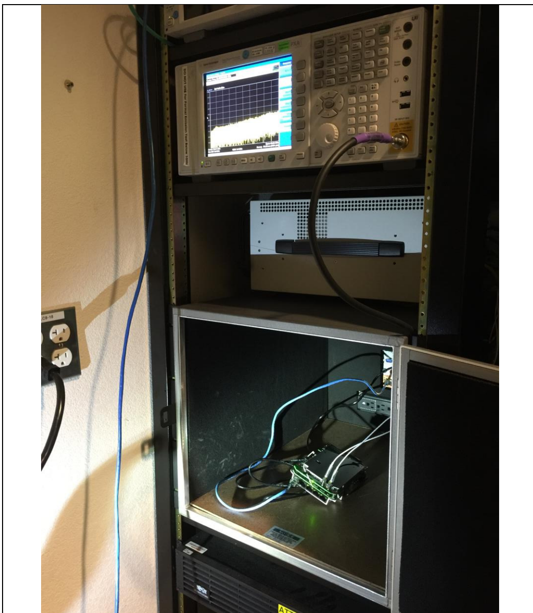
Title: Conducted Test Setup
