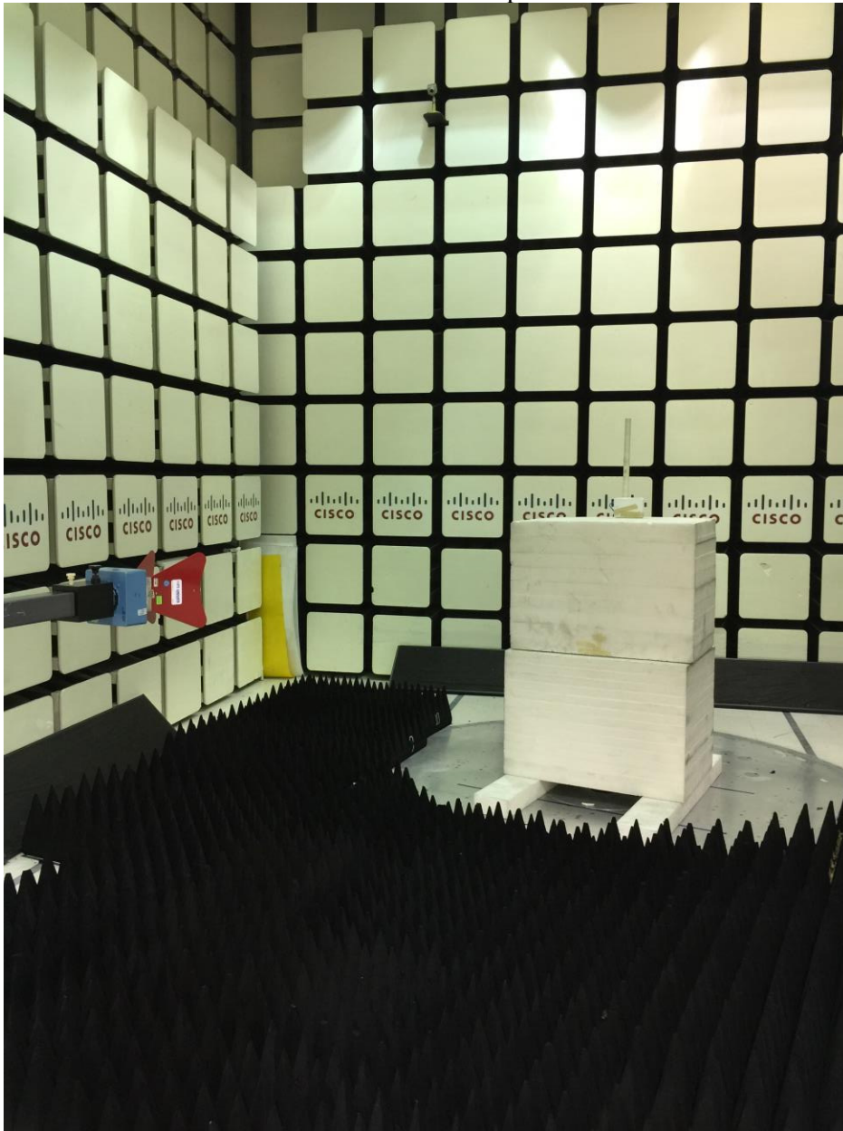
AIR-AP1810W-x-K9 Radiated Emissions setup above 1GHz
