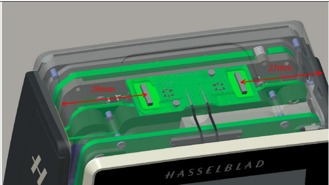
Antenna board in top of camera.
