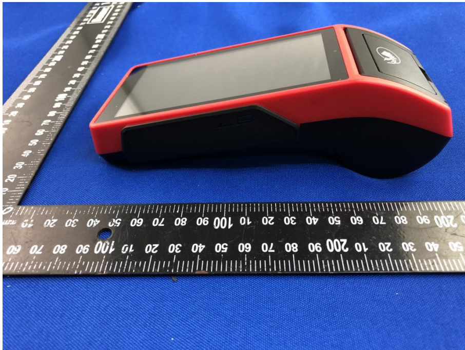
RIGHT SIDE VIEW OF EUT
