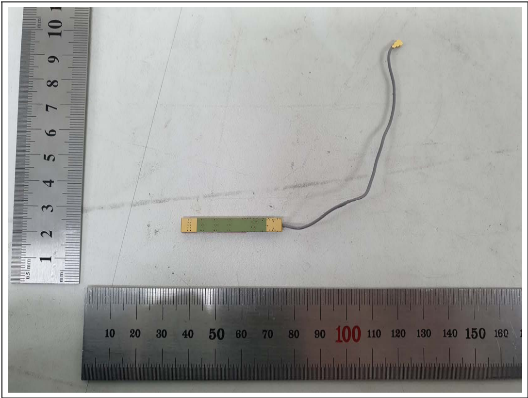
<WiFi Antenna>
