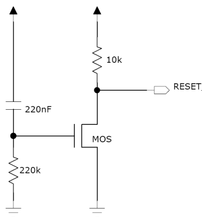
Figure 24: Example of a simple power on reset circuit.
