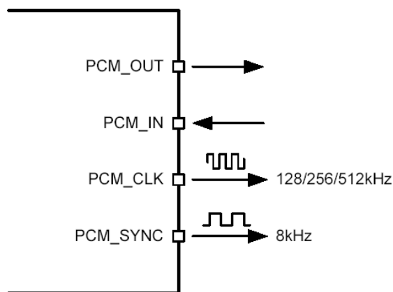
Figure 17: PCM Interface Master
