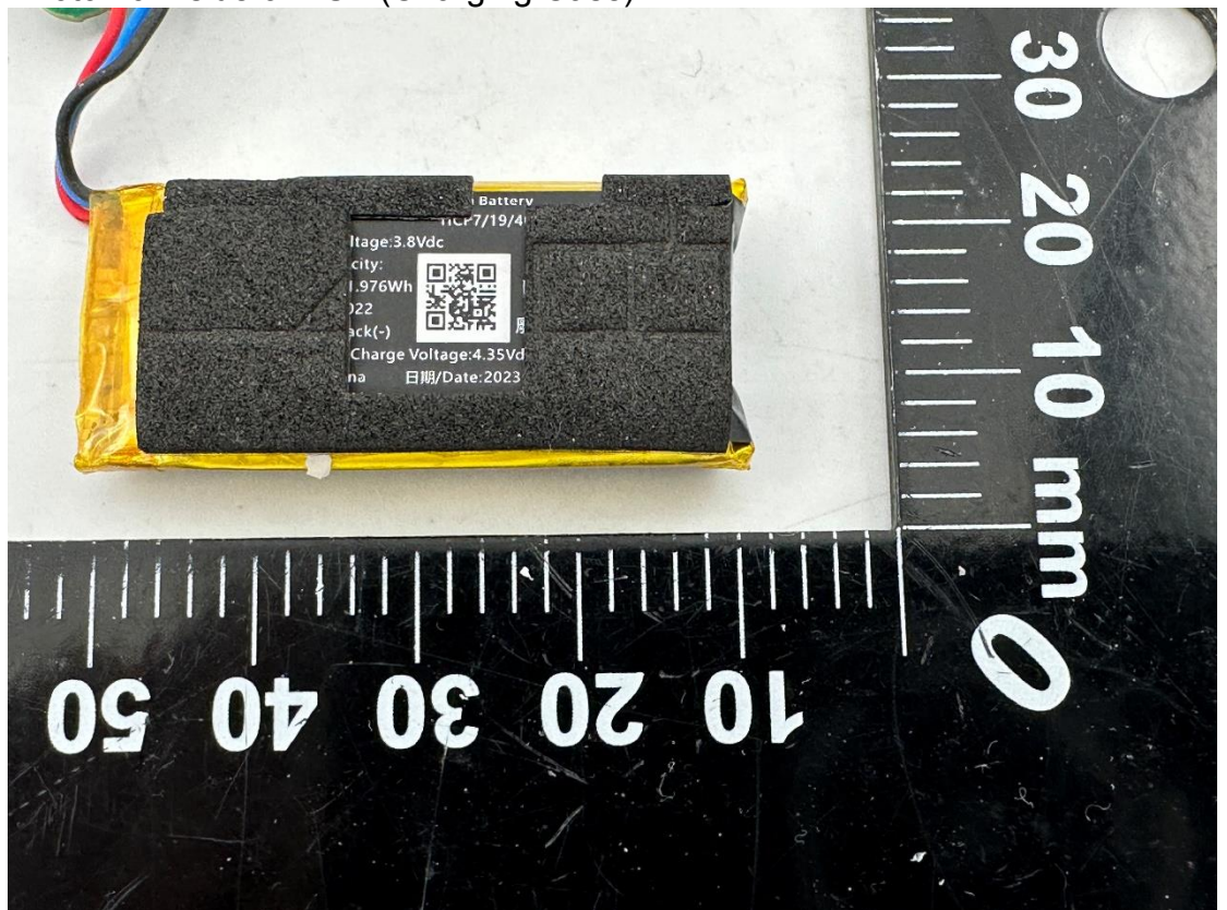
Photo 10 Inside of EUT (Charging Case)
