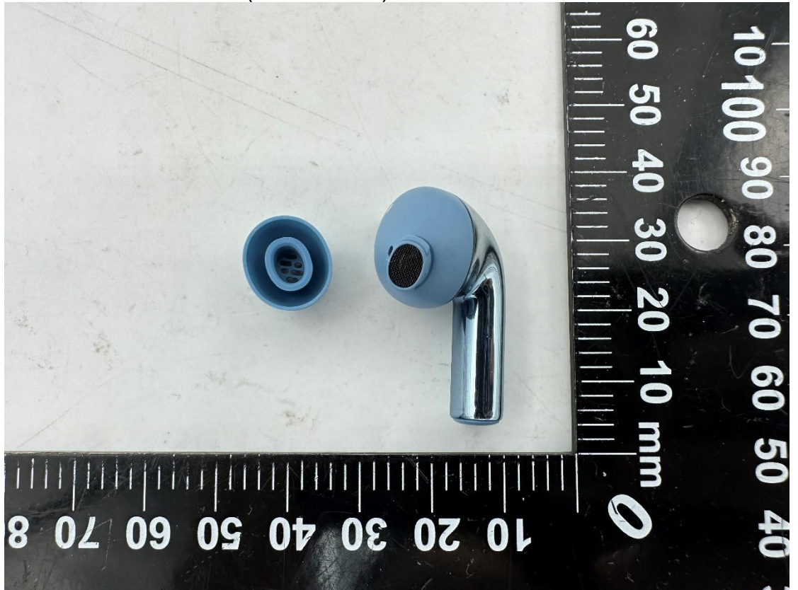
Photo 24 Inside of EUT (Left Earbuds)
