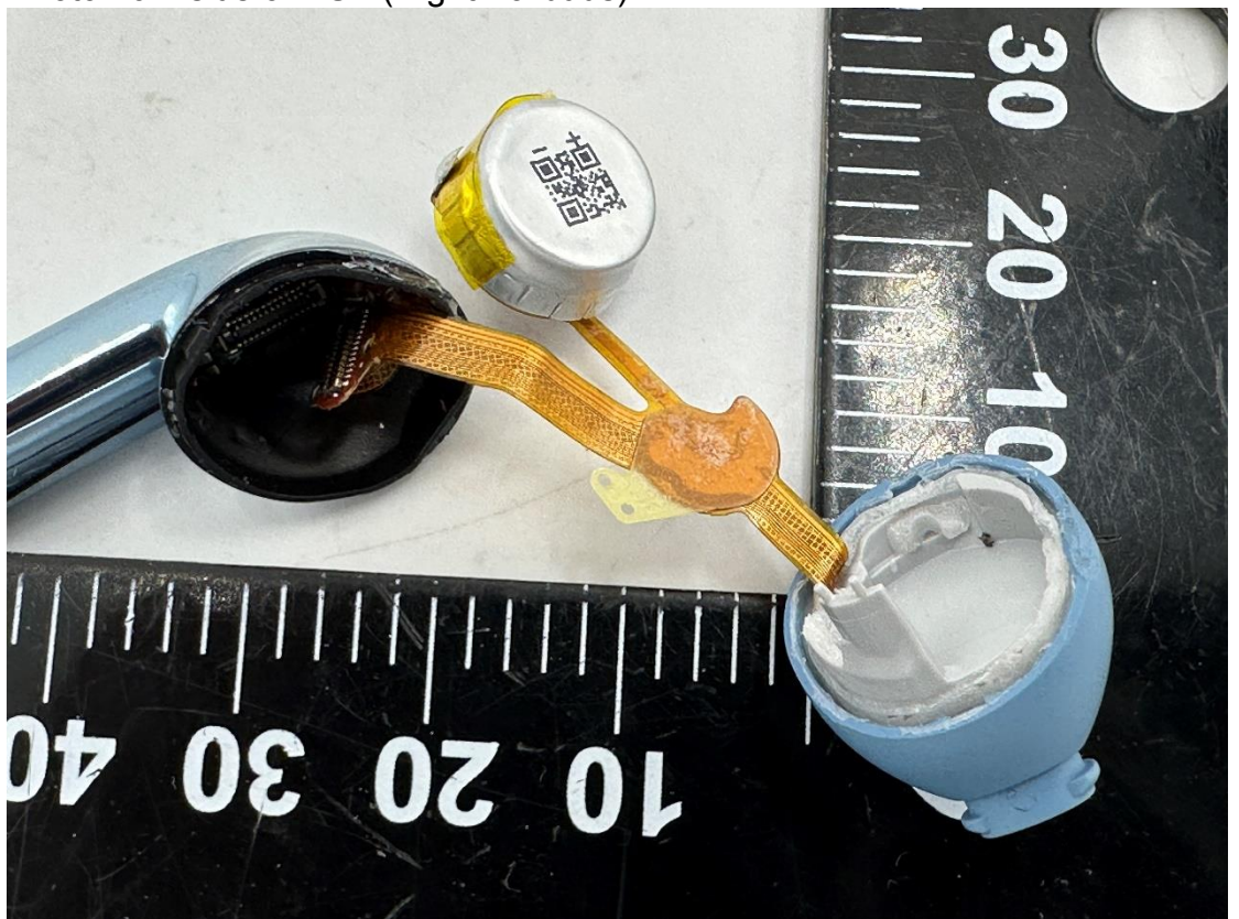
Photo 16 Inside of EUT (Right Earbuds)
