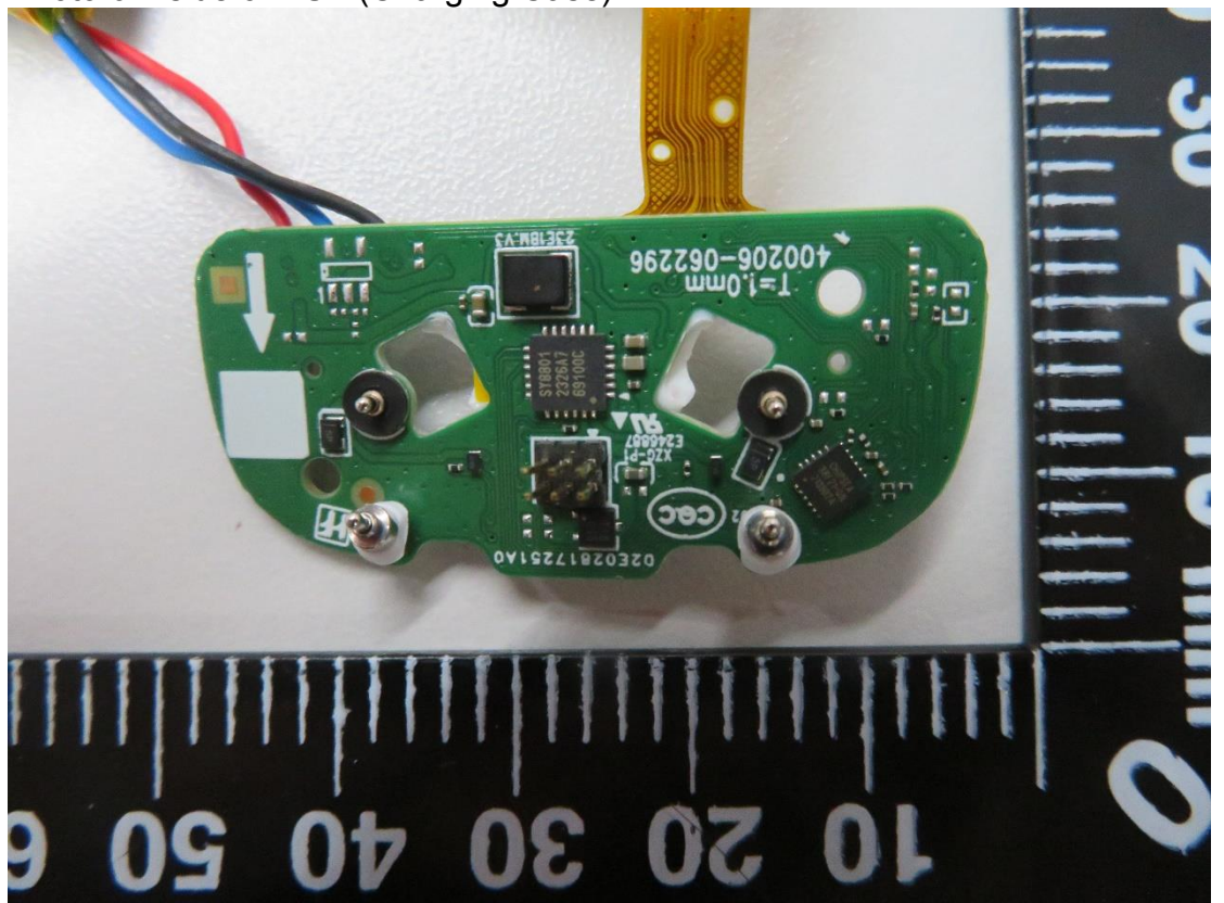
Photo 6 Inside of EUT (Charging Case)
