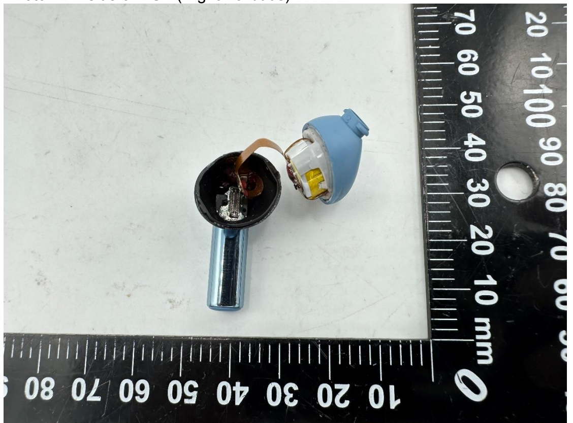
Photo 14 Inside of EUT (Right Earbuds)
