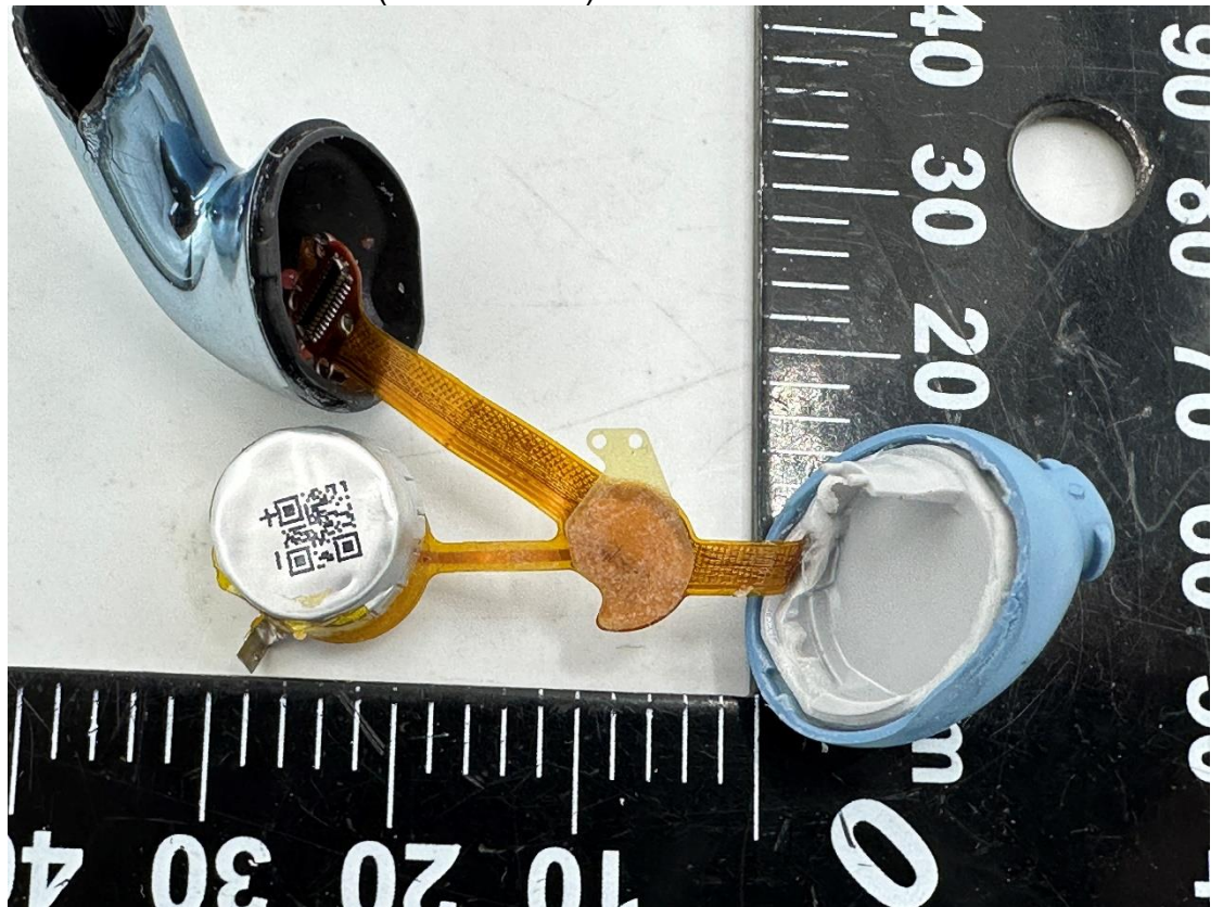
Photo 28 Inside of EUT (Left Earbuds)
