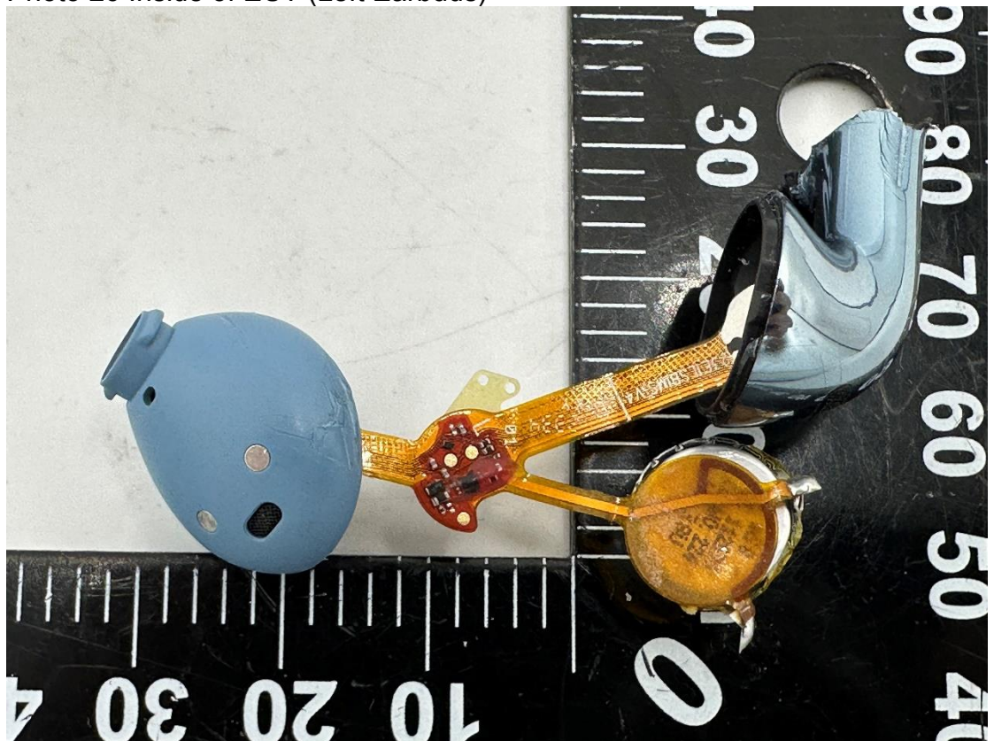
Photo 26 Inside of EUT (Left Earbuds)
