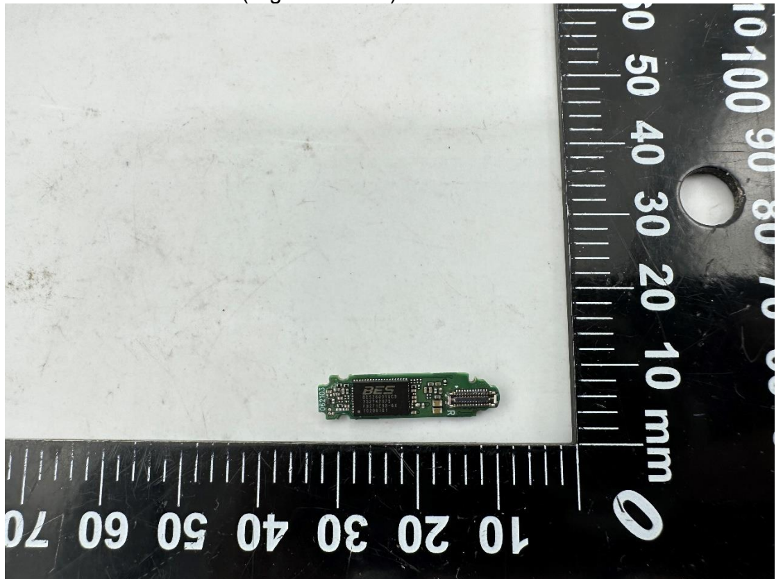
Photo 22 Inside of EUT (Right Earbuds)
