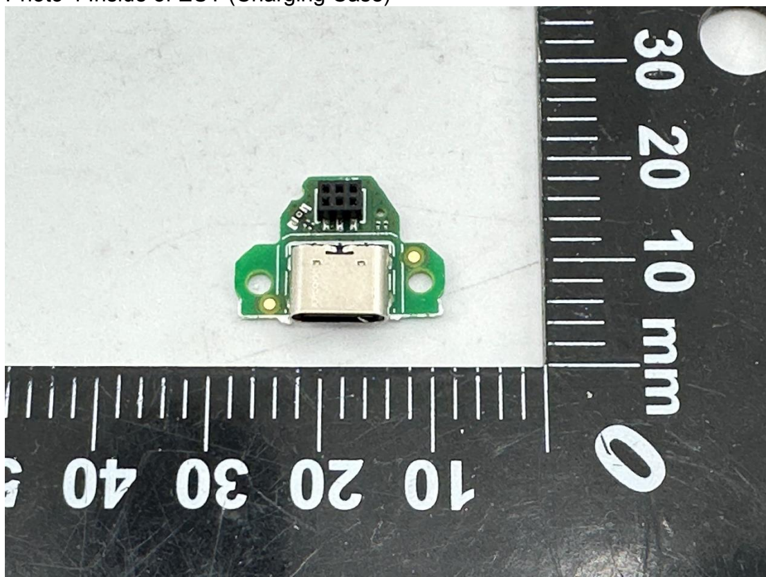
Photo 4 Inside of EUT (Charging Case)
