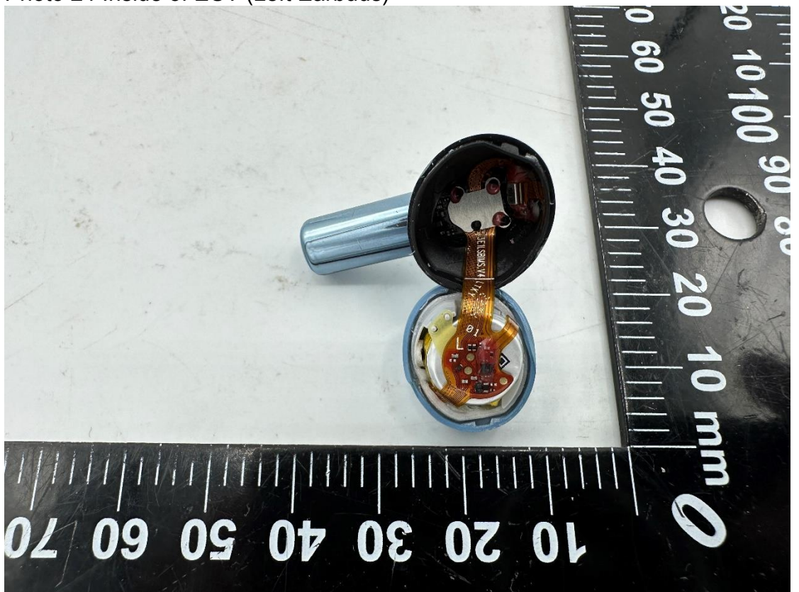
Photo 24 Inside of EUT (Left Earbuds)
