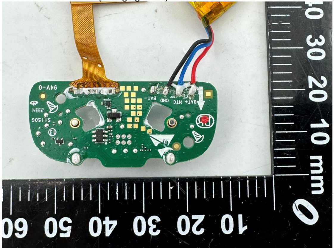
Photo 7 Inside of EUT (Charging Case)
