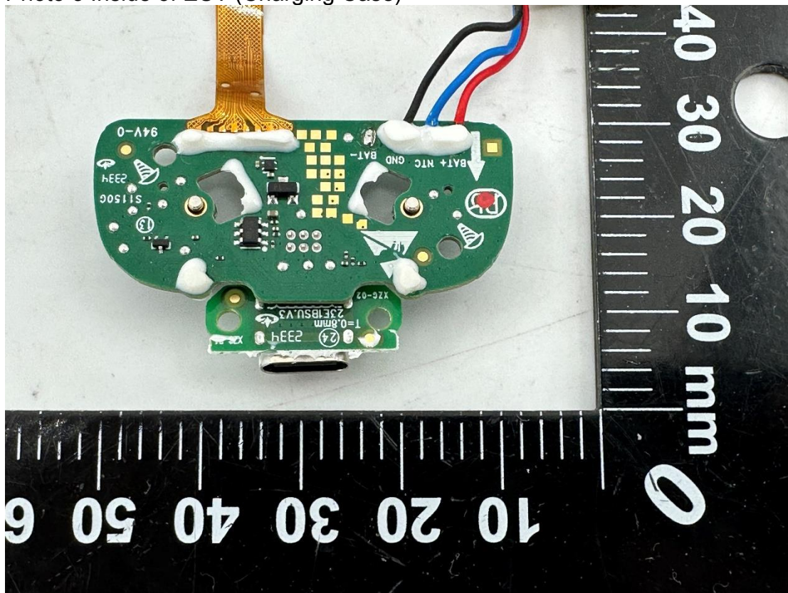
Photo 3 Inside of EUT (Charging Case)
