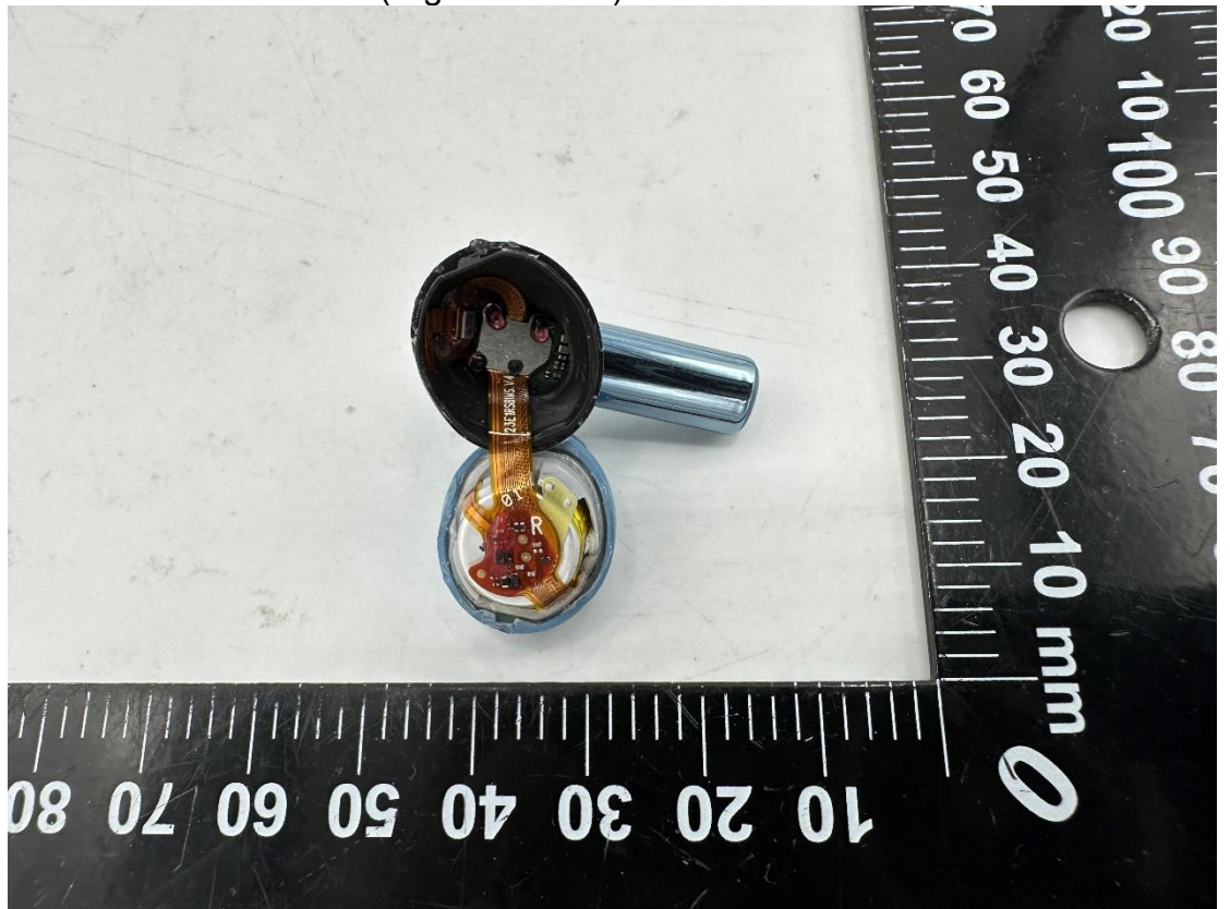
Photo 13 Inside of EUT (Right Earbuds)
