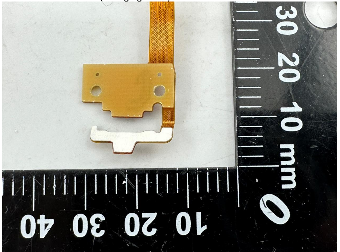
Photo 9 Inside of EUT (Charging Case)
