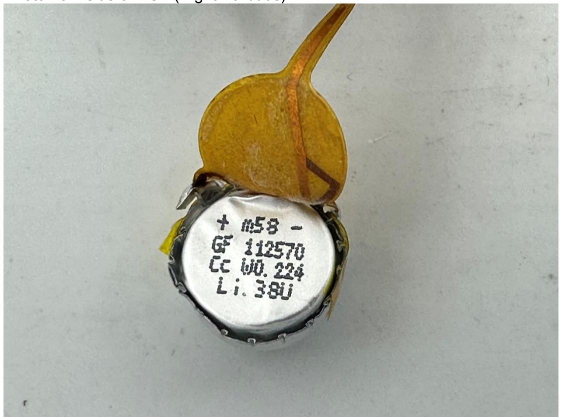
Photo 18 Inside of EUT (Right Earbuds)
