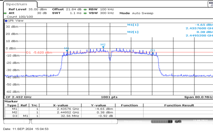
11N40SISO_Ant1_2452
