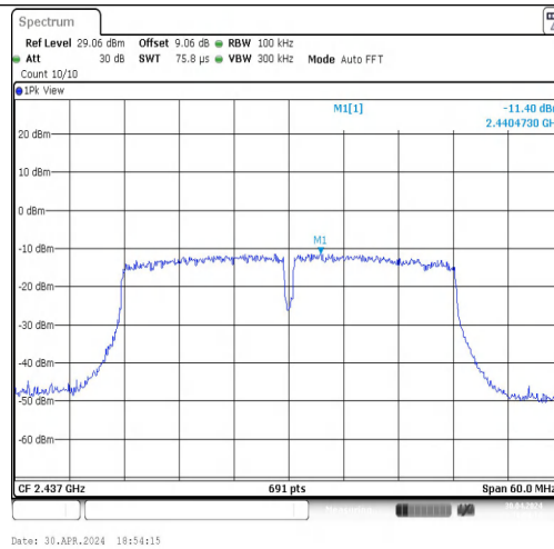
11N40MIMO-Ant1-2437-0~Reference-PASS
