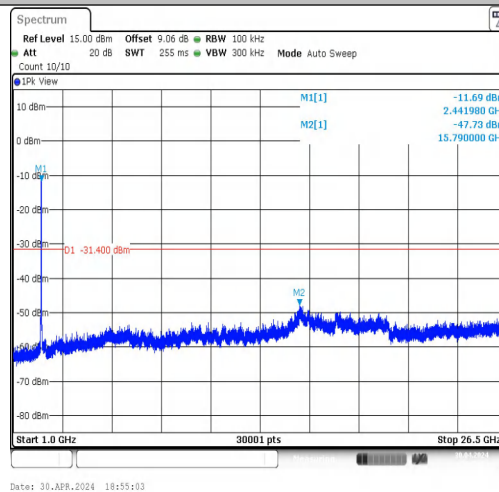
11N40MIMO-Ant1-2437-1000~26500-PASS
