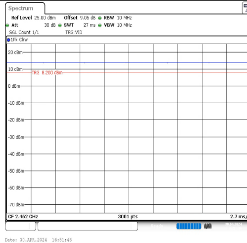
NTNV-11B-CDD-Ant1-2462
