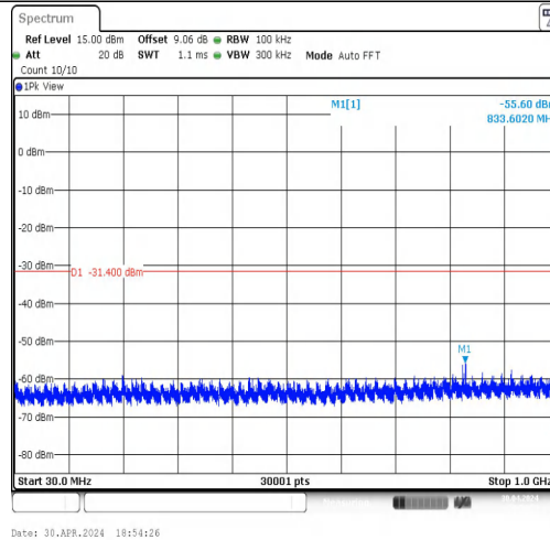
11N40MIMO-Ant1-2437-30~1000-PASS
