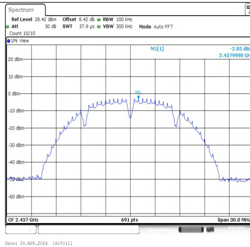
11B-CDD-Ant2-2437-0~Reference-PASS
