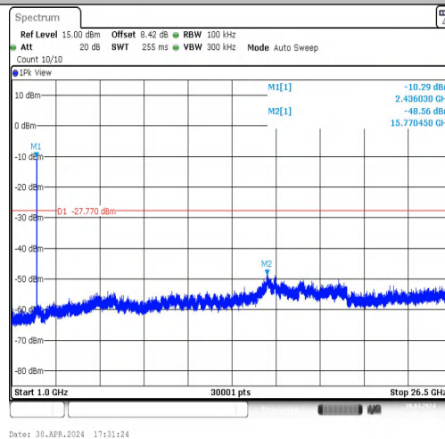
11G-CDD-Ant2-2437-1000~26500-PASS
