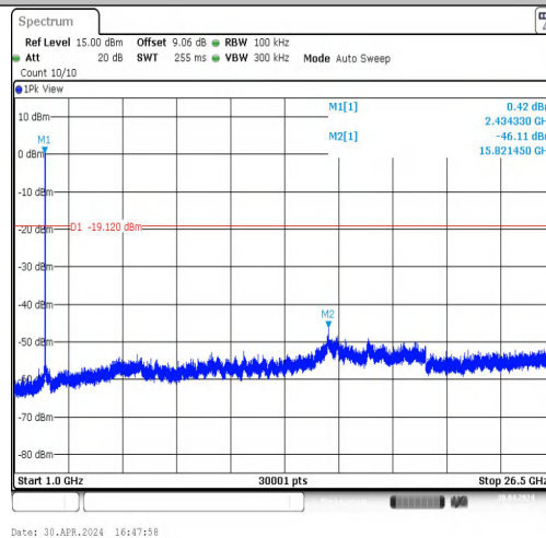
11B-CDD-Ant1-2437-1000~26500-PASS
