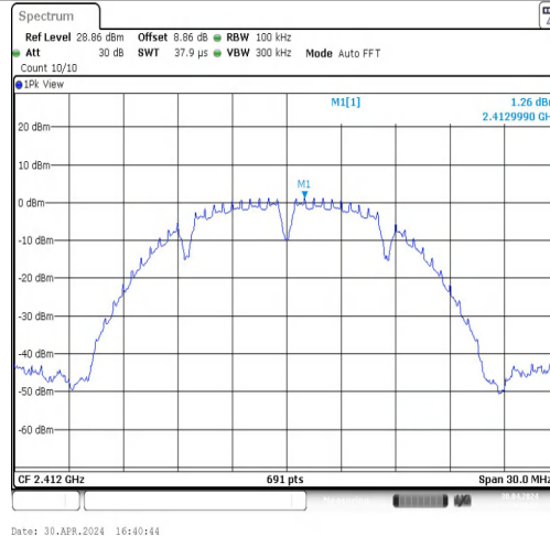
11B-CDD-Ant1-2412-0~Reference-PASS
