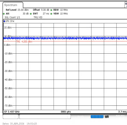
NTVN-11N40MIMO-Ant1-2437
