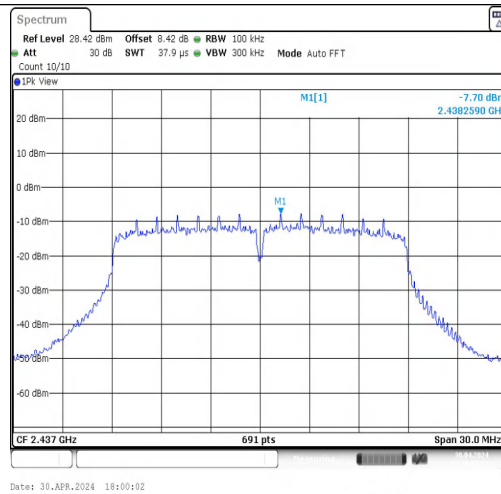
11N20MIMO-Ant2-2437-0~Reference-PASS
