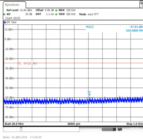
11G-CDD-Ant1-2462-30~1000-PASS
