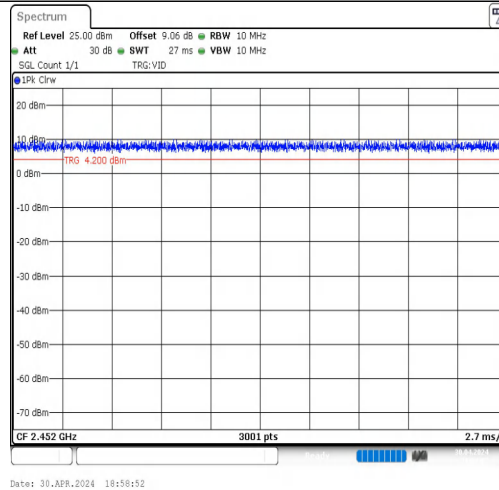
NTVN-11N40MIMO-Ant1-2452
