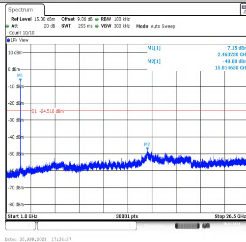
11G-CDD-Ant1-2462-1000~26500-PASS
