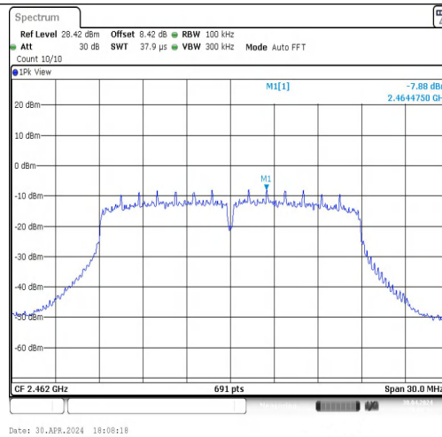
11N20MIMO-Ant2-2462-0~Reference-PASS
