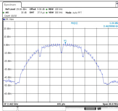
11B-CDD-Ant1-2462-0~Reference-PASS
