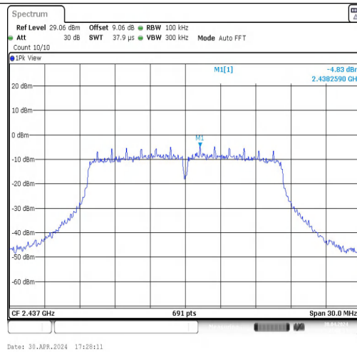
11G-CDD-Ant1-2437-0~Reference-PASS
