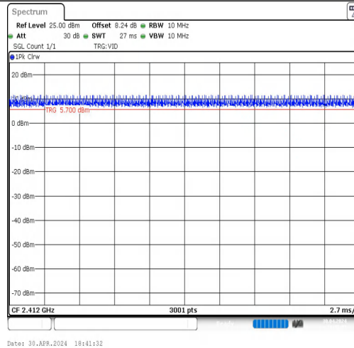
NTNV-11G-CDD-Ant2-2412
