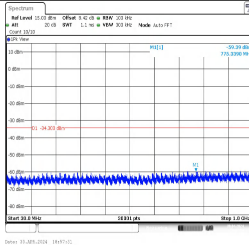
11N40MIMO-Ant2-2437-30~1000-PASS
