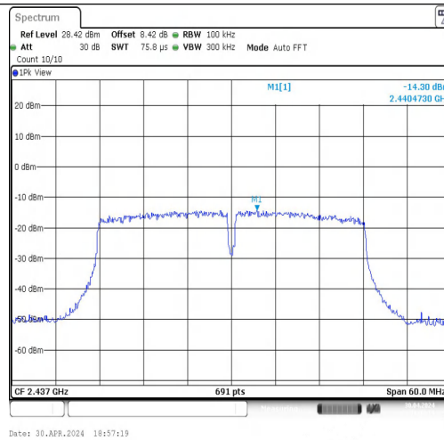
11N40MIMO-Ant2-2437-0~Reference-PASS
