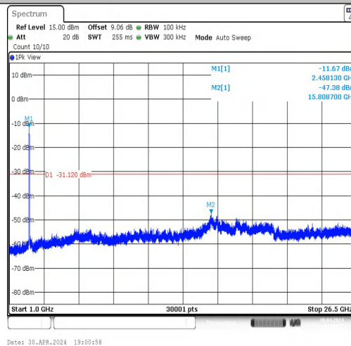
11N40MIMO-Ant1-2452-1000~26500-PASS
