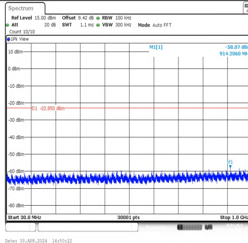
11B-CDD-Ant2-2437-30~1000-PASS
