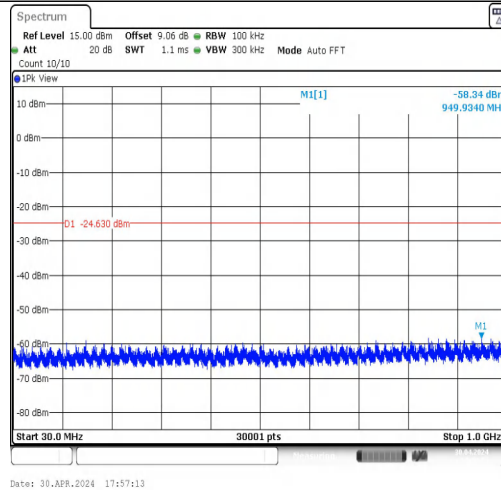
11N20MIMO-Ant1-2437-30~1000-PASS
