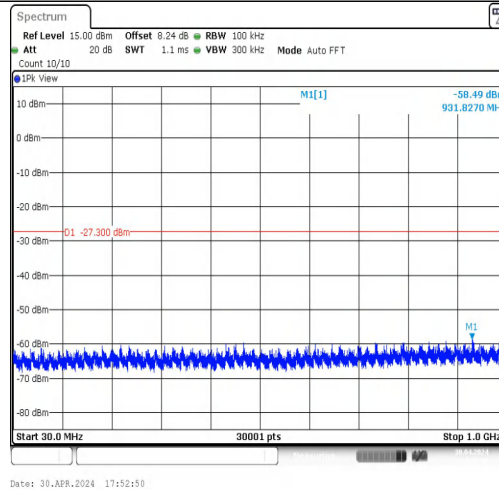
11N20MIMO-Ant2-2412-30~1000-PASS
