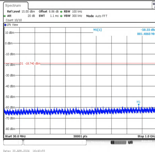
11B-CDD-Ant1-2412-30~1000-PASS
