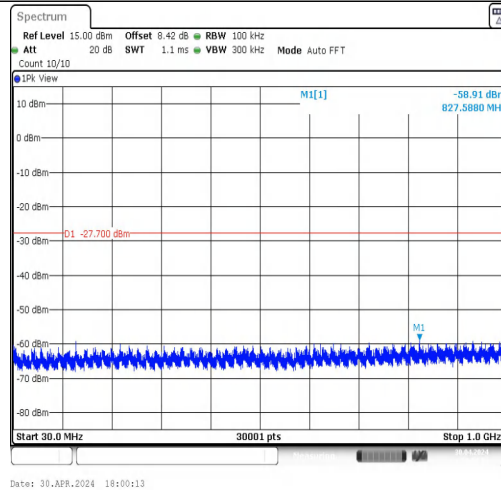
11N20MIMO-Ant2-2437-30~1000-PASS
