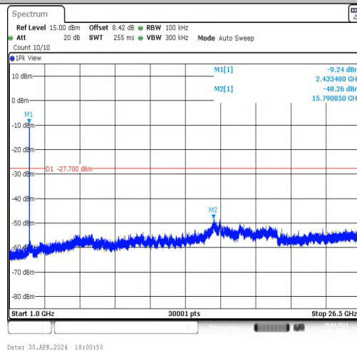
11N20MIMO-Ant2-2437-1000~26500-PASS
