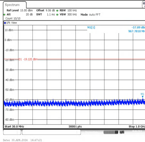
11B-CDD-Ant1-2437-30~1000-PASS
