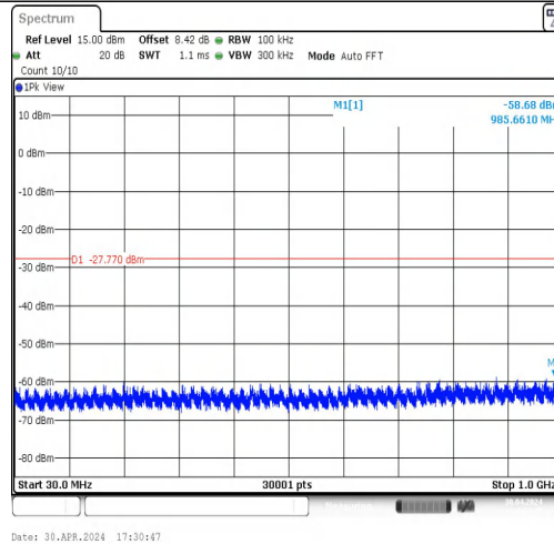
11G-CDD-Ant2-2437-30~1000-PASS
