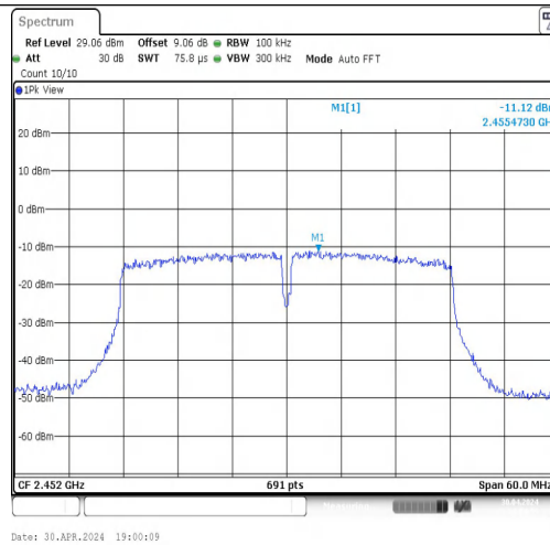
11N40MIMO-Ant1-2452-0~Reference-PASS
