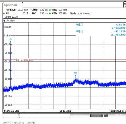
11N20MIMO-Ant2-2462-1000~26500-PASS
