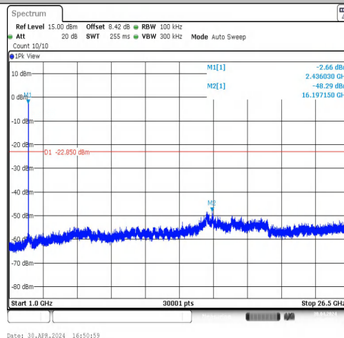
11B-CDD-Ant2-2437-1000~26500-PASS
