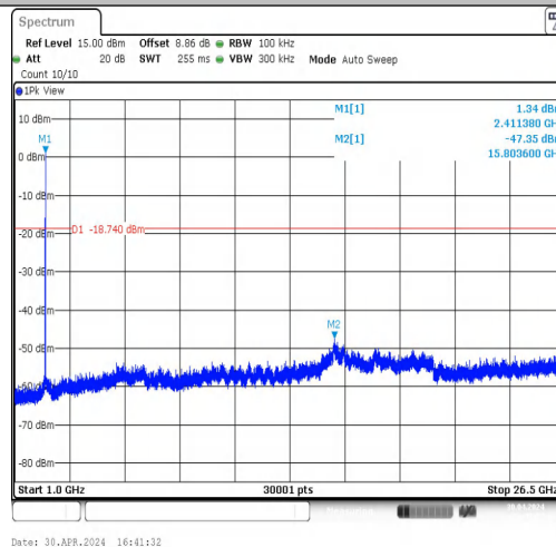
11B-CDD-Ant1-2412-1000~26500-PASS
