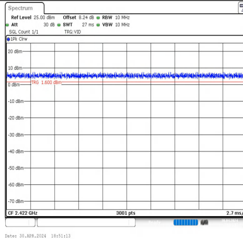
NTVN-11N40MIMO-Ant2-2422
