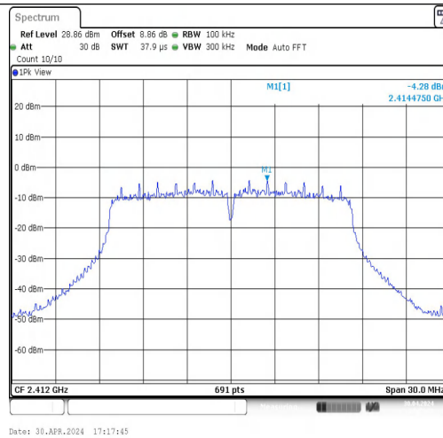
11G-CDD-Ant1-2412-0~Reference-PASS
