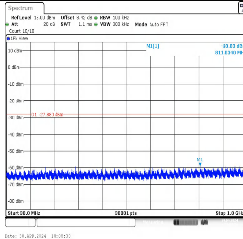
11N20MIMO-Ant2-2462-30~1000-PASS
