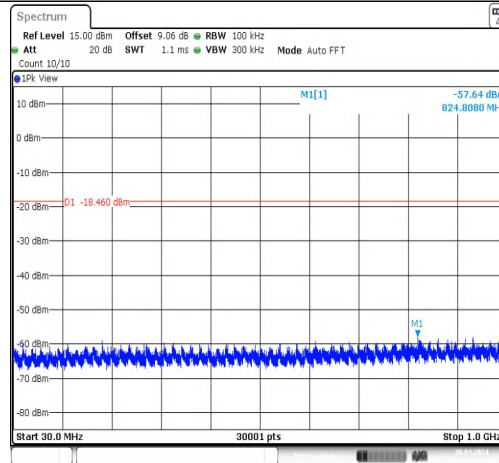
11B-CDD-Ant1-2462-0~Reference-PASS
