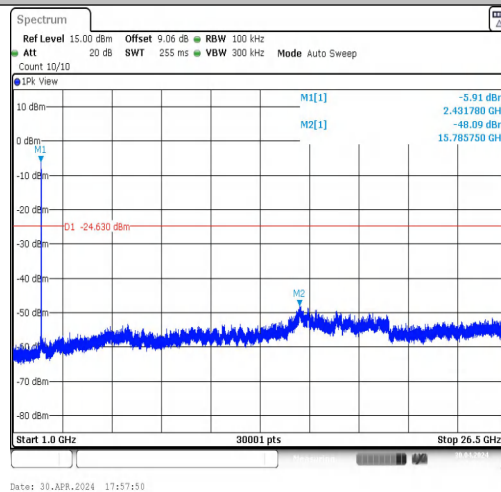
11N20MIMO-Ant1-2437-1000~26500-PASS
