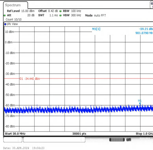
11N40MIMO-Ant2-2452-30~1000-PASS
