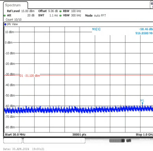
11N40MIMO-Ant1-2452-30~1000-PASS
