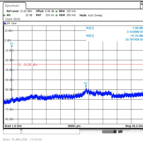
11G-CDD-Ant1-2412-1000~26500-PASS
