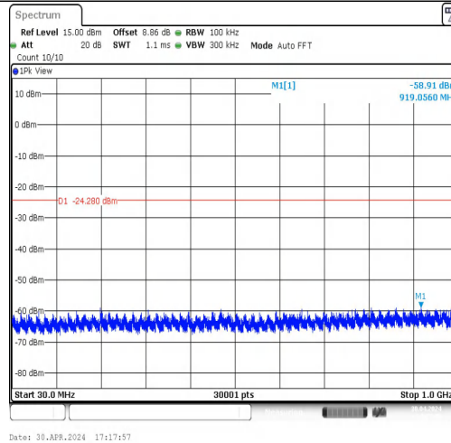
11G-CDD-Ant1-2412-30~1000-PASS
