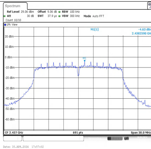
11N20MIMO-Ant1-2437-0~Reference-PASS
