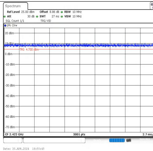
NTVN-11N40MIMO-Ant1-2422
