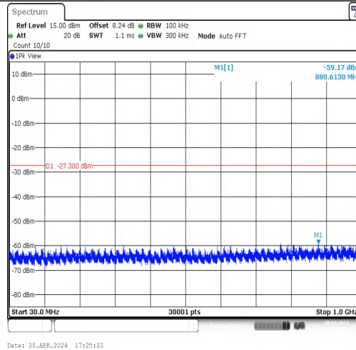
11G-CDD-Ant2-2412-30~1000-PASS
