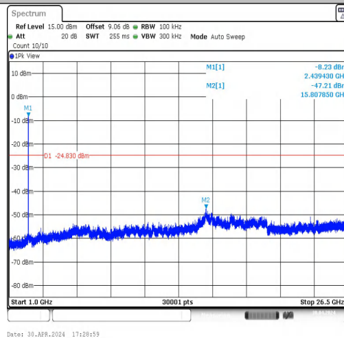
11G-CDD-Ant1-2437-1000~26500-PASS
