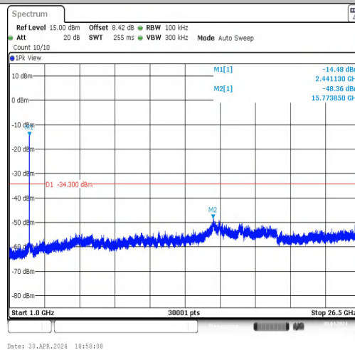
11N40MIMO-Ant2-2437-1000~26500-PASS
