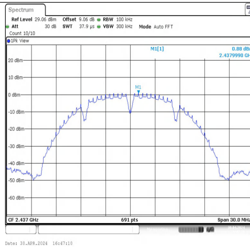
11B-CDD-Ant1-2437-0~Reference-PASS
