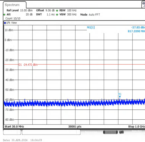
11N20MIMO-Ant1-2462-30~1000-PASS
