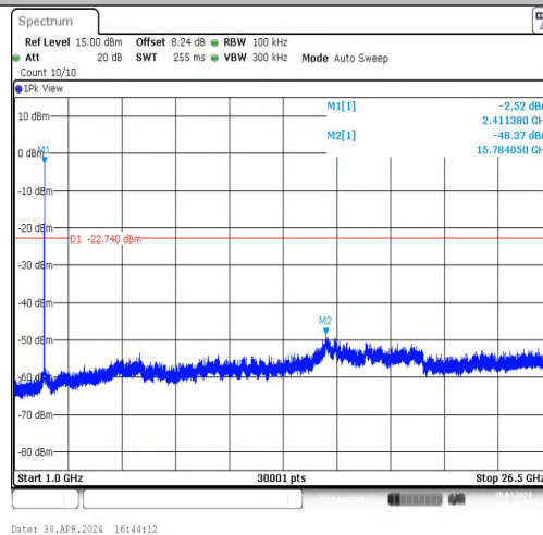
11B-CDD-Ant2-2412-1000~26500-PASS
