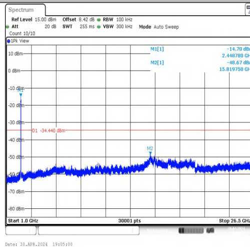
11N40MIMO-Ant2-2452-1000~26500-PASS
