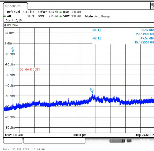
11N20MIMO-Ant1-2462-1000~26500-PASS
