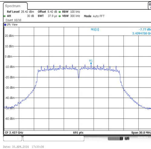
11G-CDD-Ant2-2437-0~Reference-PASS
