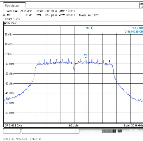
11G-CDD-Ant1-2462-0~Reference-PASS
