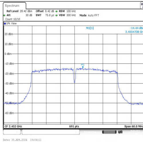
11N40MIMO-Ant2-2452-0~Reference-PASS
