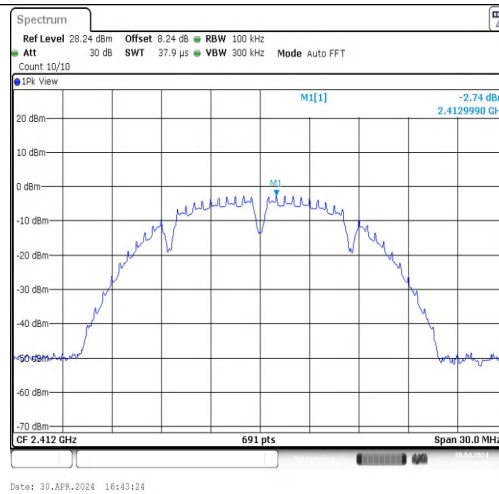
11B-CDD-Ant2-2412-0~Reference-PASS
