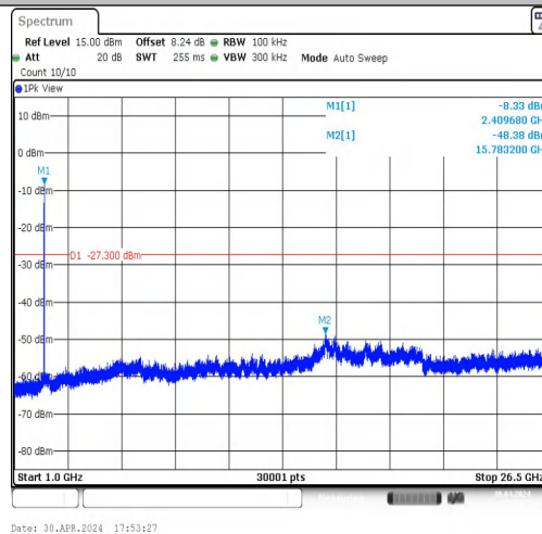
11N20MIMO-Ant2-2412-1000~26500-PASS
