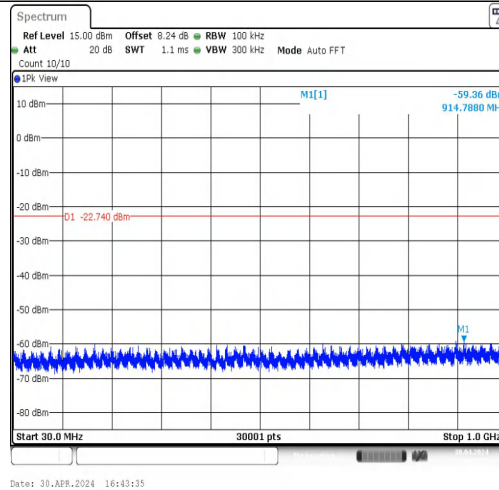
11B-CDD-Ant2-2412-30~1000-PASS
