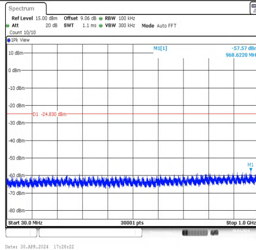
11G-CDD-Ant1-2437-30~1000-PASS
