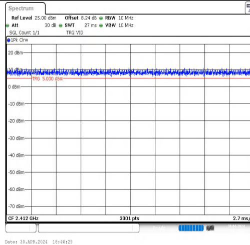
NTVN-11N20MIMO-Ant2-2412
