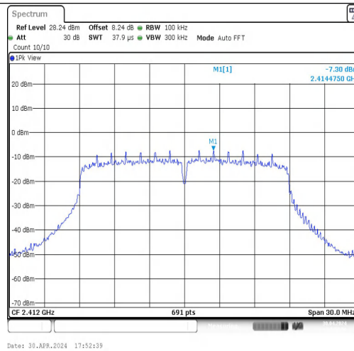
11N20MIMO-Ant2-2412-0~Reference-PASS
