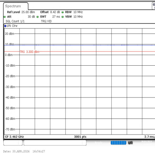
NTNV-11B-CDD-Ant2-2462
