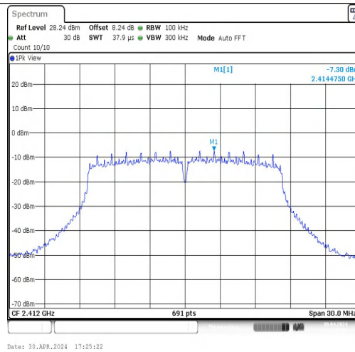
11G-CDD-Ant2-2412-0~Reference-PASS
