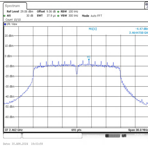
11N20MIMO-Ant1-2462-0~Reference-PASS
