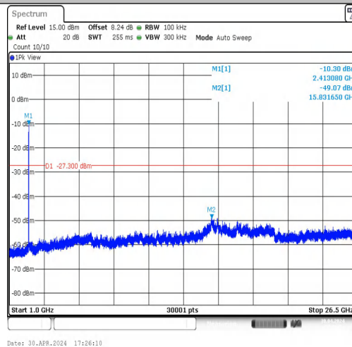
11G-CDD-Ant2-2412-1000~26500-PASS
