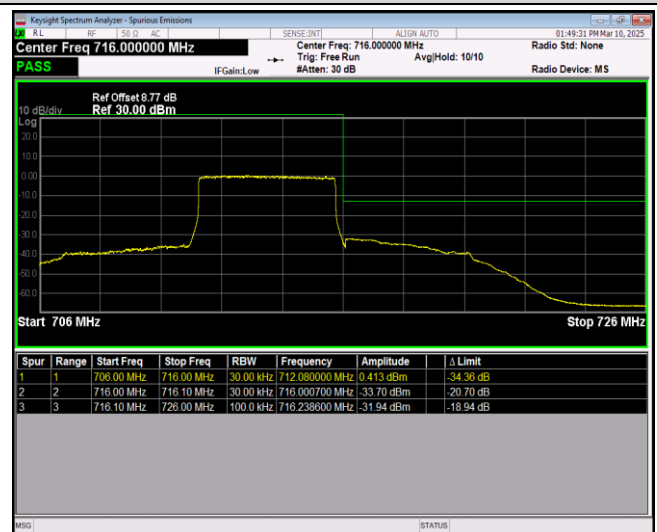
Band17-5MHz-16QAM-23755-1RB#24
