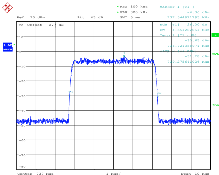
Input_DL_1S_M_AWGN_AGC+3dB_26dB Bandwidth
