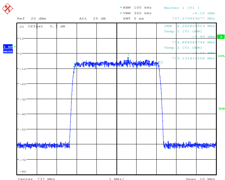
Input_DL_1S_M_AWGN_AGC+3dB_99% OBW
