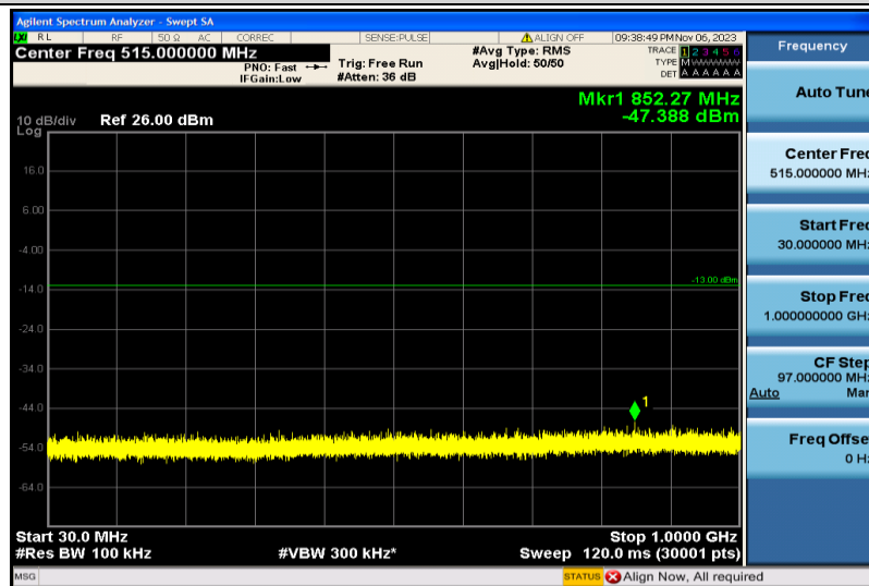
Band4-3MHz-16QAM-20385-1RB#0-30~1000MHz
