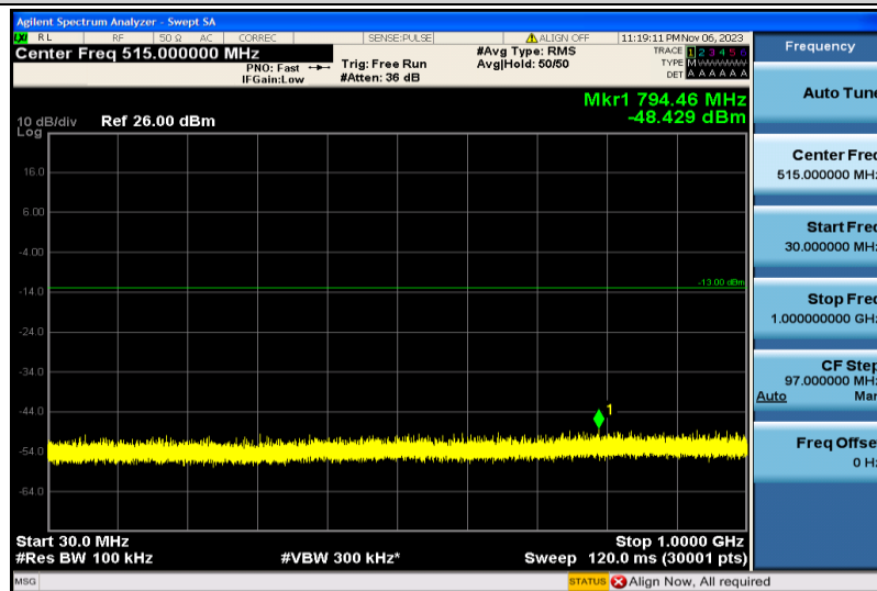
Band4-20MHz-16QAM-20300-1RB#0-30~1000MHz
