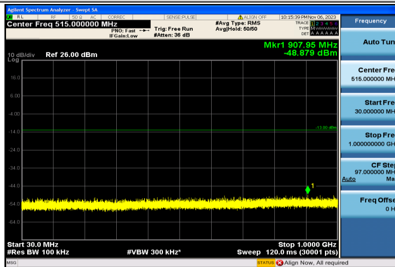
Band4-10MHz-16QAM-20350-1RB#0-30~1000MHz
