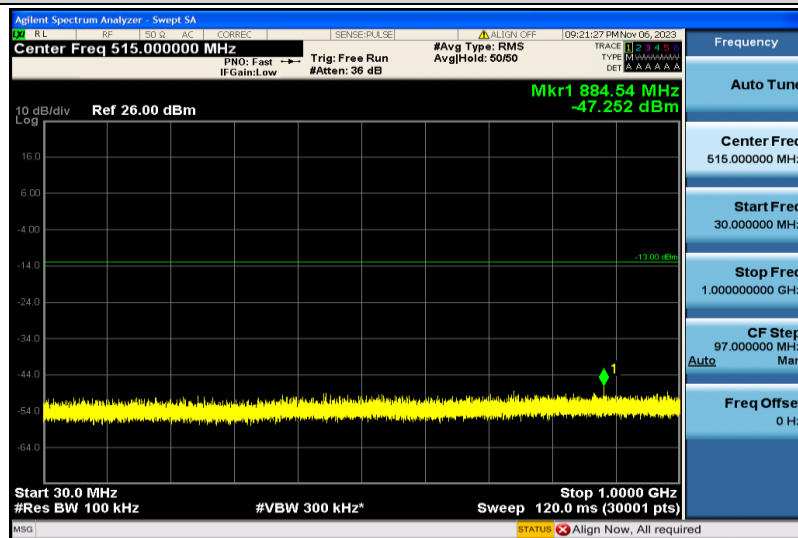
Band4-1.4MHz-16QAM-20393-1RB#0-30~1000MHz
