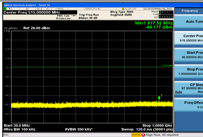
Band4-10MHz-QPSK-20350-1RB#0-30~1000MHz
