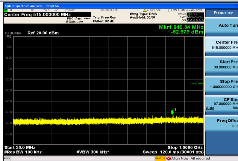
Band7-5MHz-QPSK-21425-1RB#0-30~1000MHz
