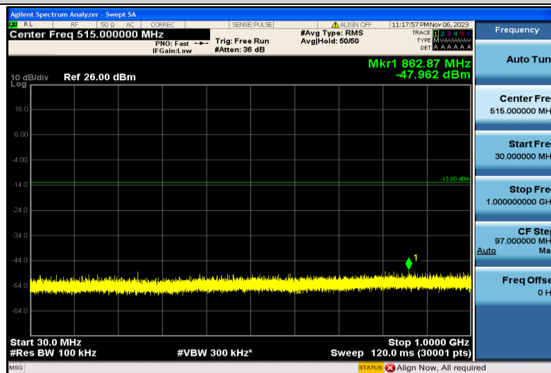
Band4-20MHz-16QAM-20175-1RB#0-30~1000MHz
