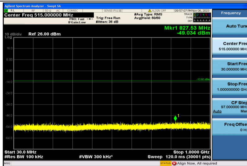
Band4-5MHz-16QAM-20375-1RB#0-30~1000MHz
