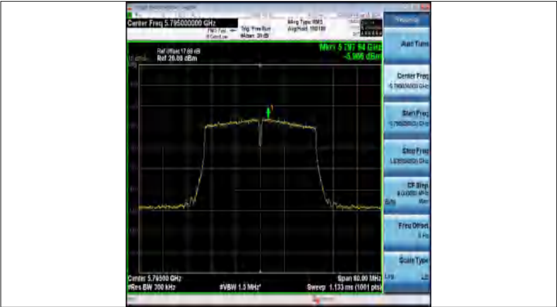
11N40SISO-Ant2-5795-PASS
