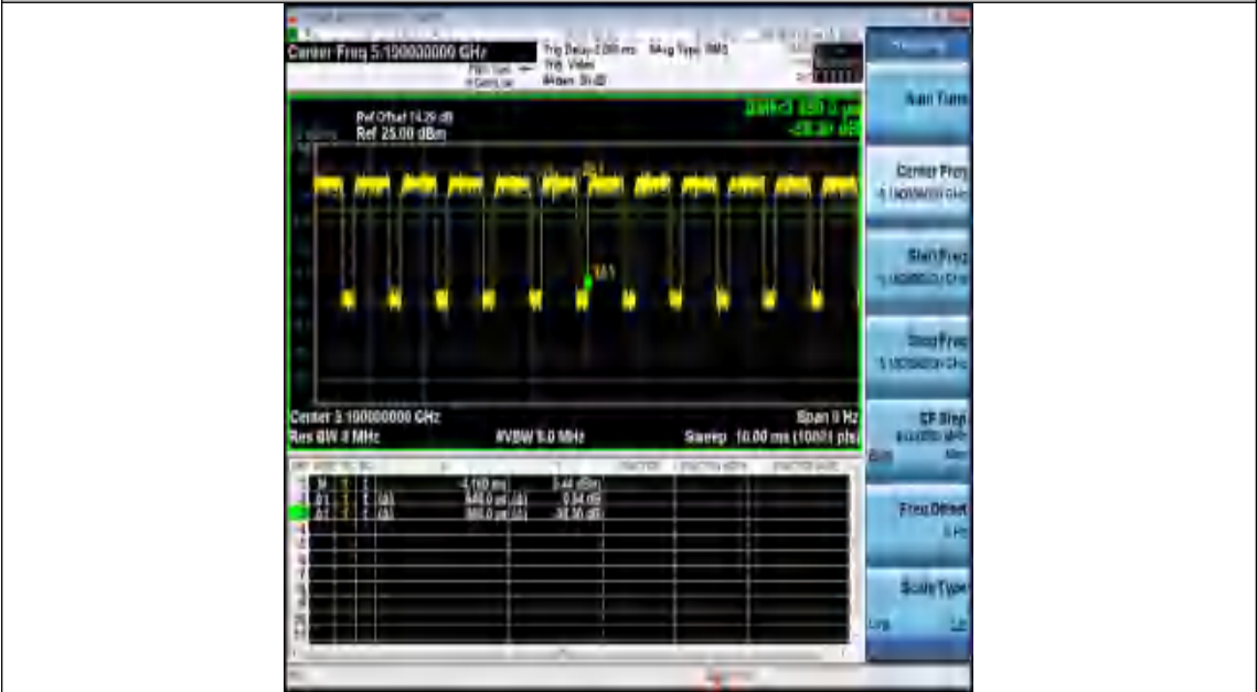
NTNV-11AX40ISO-Ant2-5190
