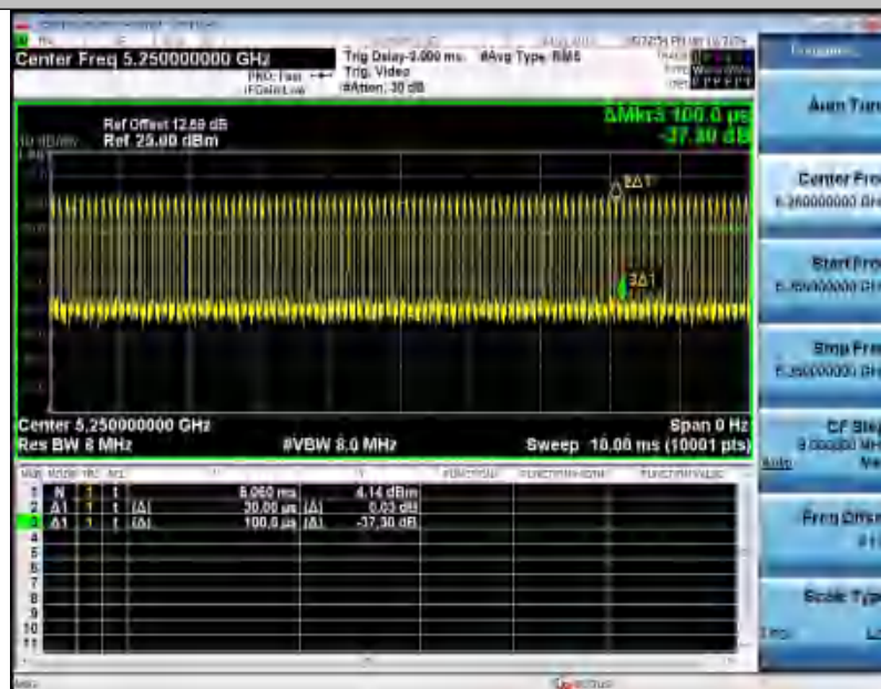
NTNV-11AX160SISO-Ant2-5250
