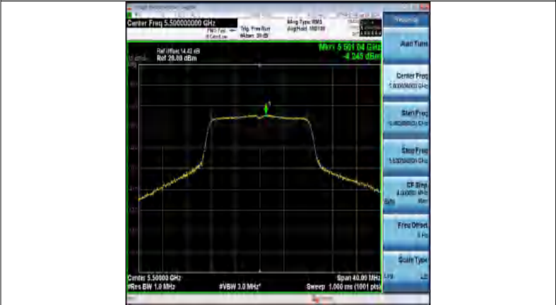
11AX20SISO-Ant1-5500-PASS
