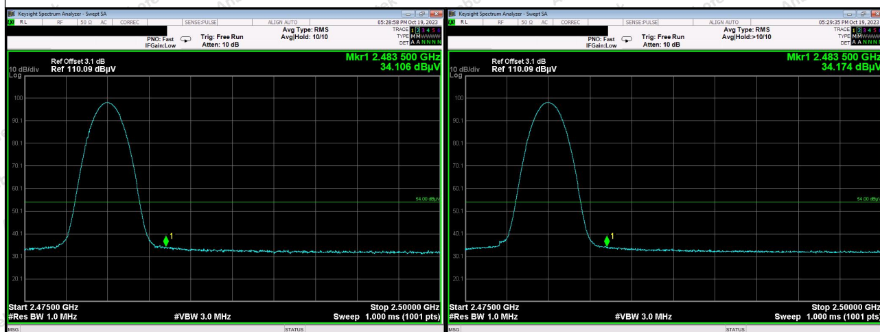
Average Value(Vertical)
