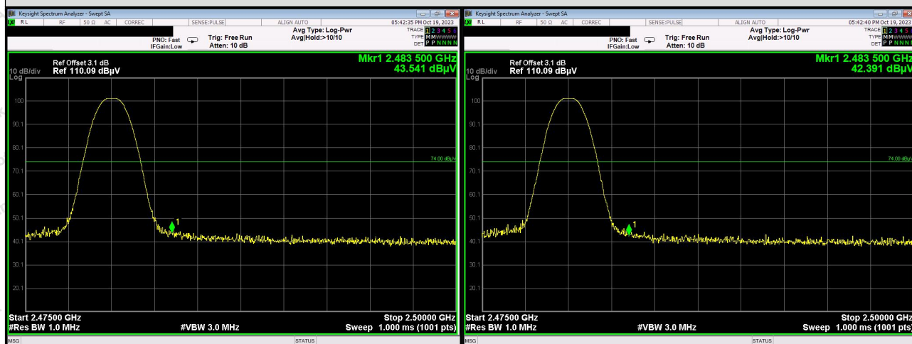
Peak Value(Vertical)
