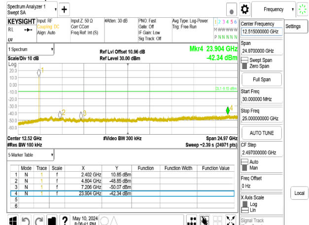
Spurious Emission_GFSK_1M_DH5_2402MHz_Chain1
