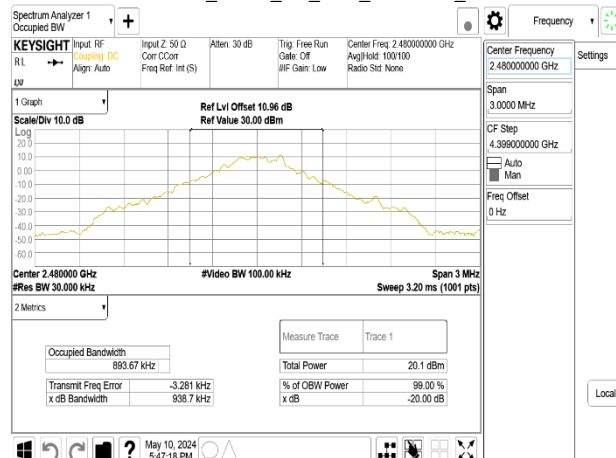
OBW 20dB_GFSK_1M_DH5_2480MHz_Chain1
