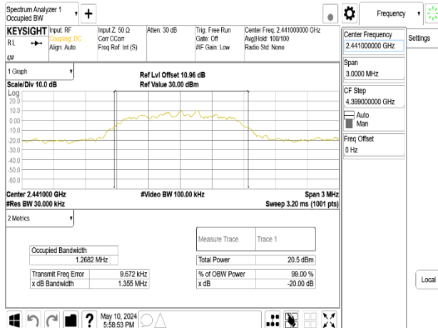
OBW 20dB_π/4QPSK_2M_DH5_2441MHz_Chain0
