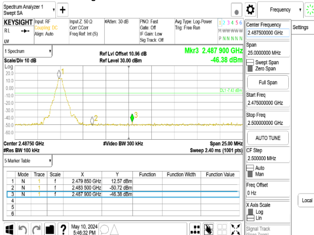
Band Edge_GFSK_1M_DH5_2480MHz_Chain0
