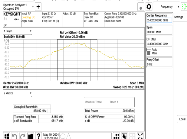
OBW 20dB_GFSK_1M_DH5_2402MHz_Chain1
