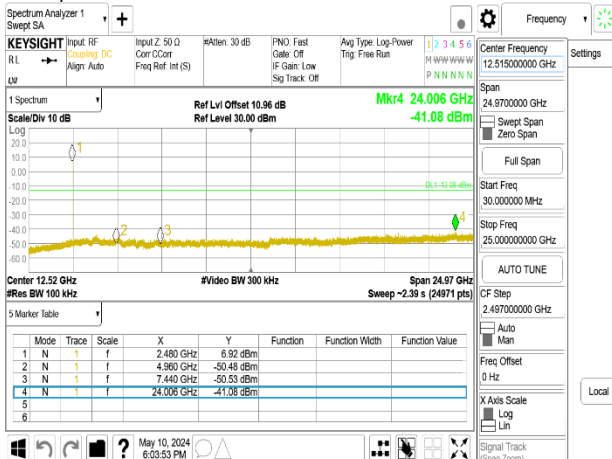
Spurious Emission_π/4DQPSK_2M_DH5_2480MHz_Chain0
