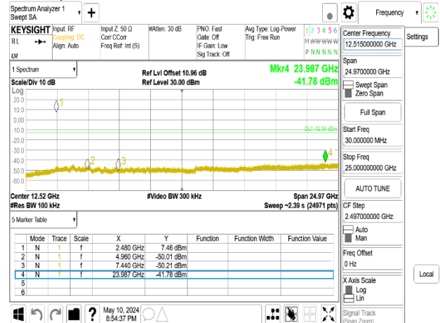
Spurious Emission_8DPSK_3M_DH5_2480MHz_Chain1
