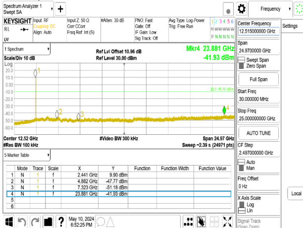
Spurious Emission_8DPSK_3M_DH5_2441MHz_Chain1
