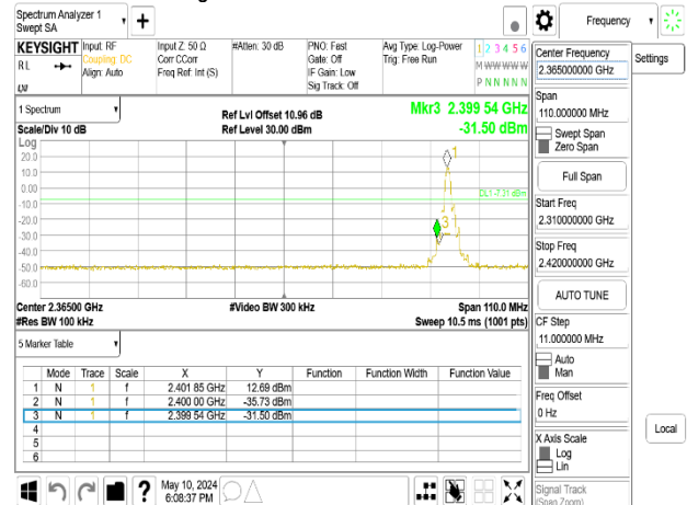
Band Edge_8DPSK_3M_DH5_2402MHz_Chain1
