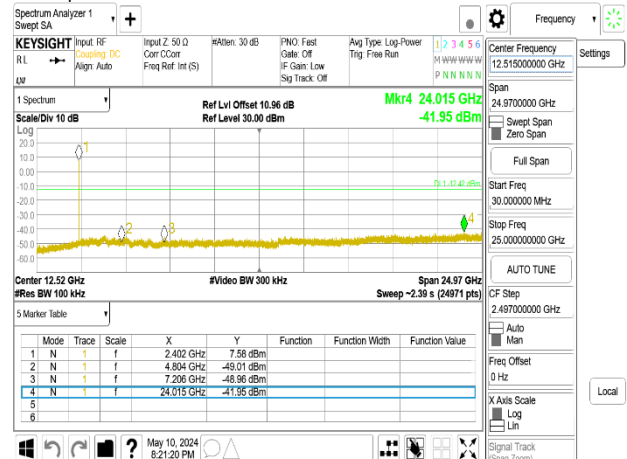
Spurious Emission_π/4DQPSK_2M_DH5_2402MHz_Chain1
