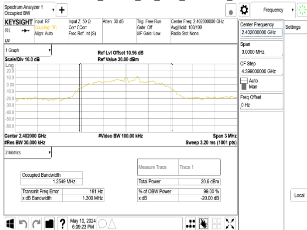
OBW 20dB_8DPSK_3M_DH5_2402MHz_Chain1
