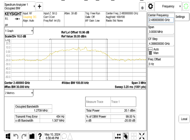
OBW 20dB_8DPSK_3M_DH5_2480MHz_Chain1
