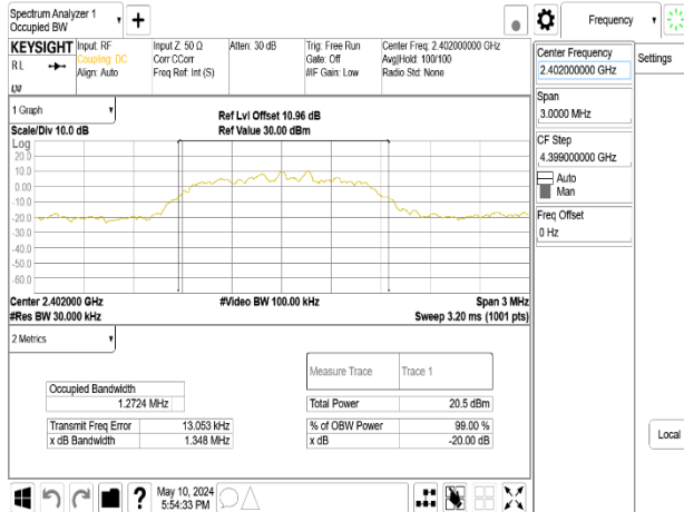
OBW 20dB_π/4QPSK_2M_DH5_2402MHz_Chain1
