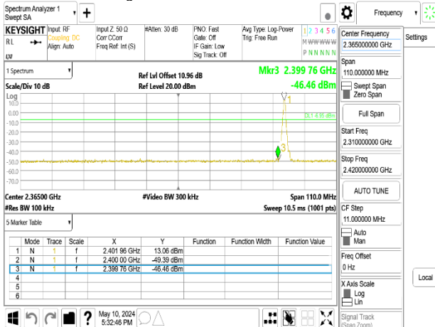
Band Edge_GFSK_1M_DH5_2402MHz_Chain1
