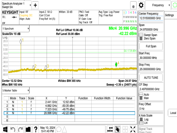
Spurious Emission_GFSK_1M_DH5_2441MHz_Chain1
