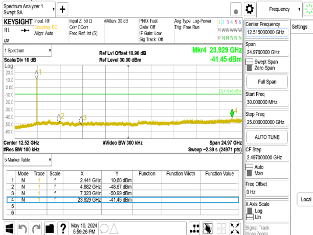
Spurious Emission_π/4DQPSK_2M_DH5_2441MHz_Chain1
