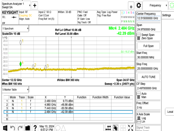
Spurious Emission_8DPSK_3M_DH5_2480MHz_Chain0
