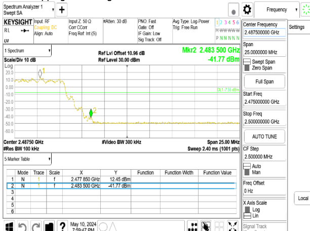
Hopping Band Edge_8DPSK_3M_DH5_2480MHz_Chain0
