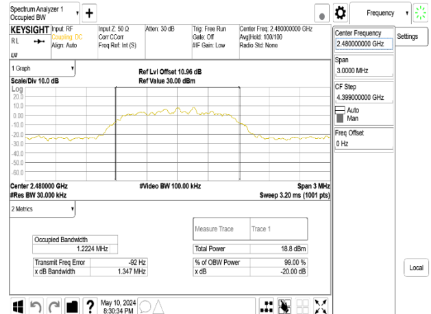
OBW 20dB_π/4QPSK_2M_DH5_2480MHz_Chain1
