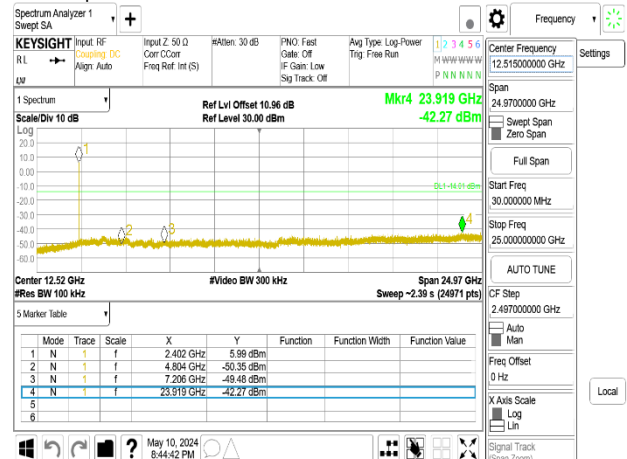
Spurious Emission_8DPSK_3M_DH5_2402MHz_Chain1
