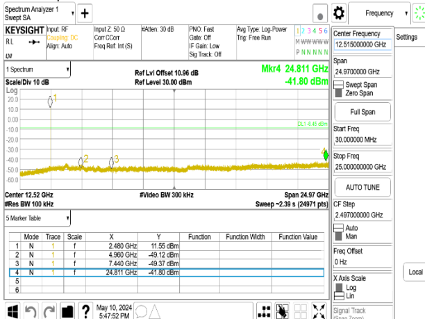
Spurious Emission_GFSK_1M_DH5_2480MHz_Chain0
