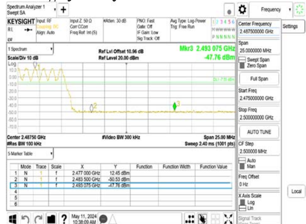
Hopping Band Edge_GFSK_1M_DH5_2480MHz_Chain1
