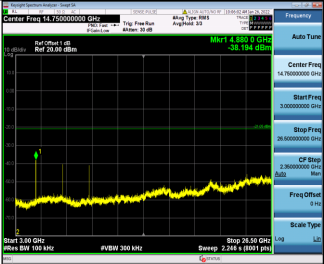
BLE_2440_3000-26500
