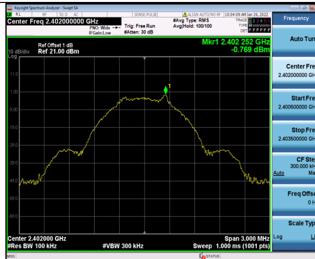
BLE_2402-Reference
