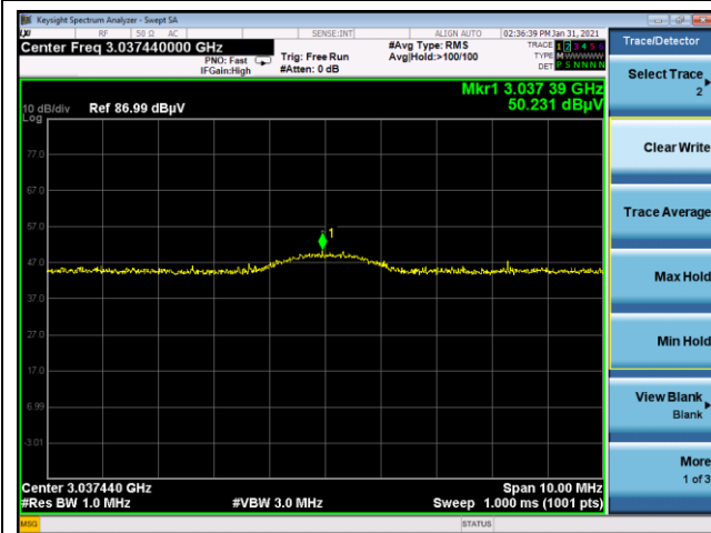
10 th harmonic
