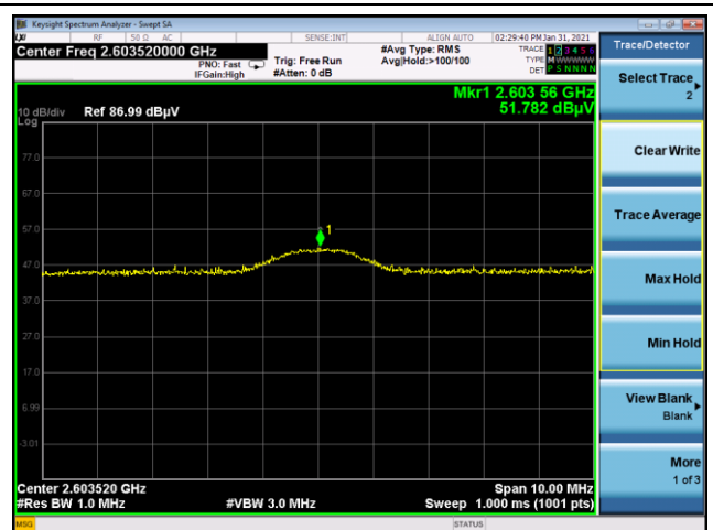
6 th harmonic
