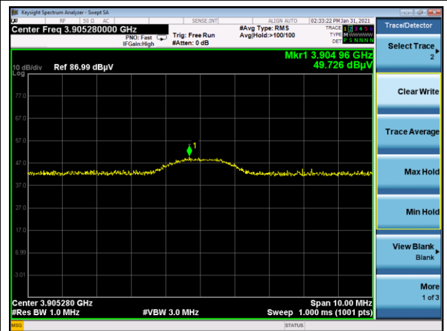
9 th harmonic
