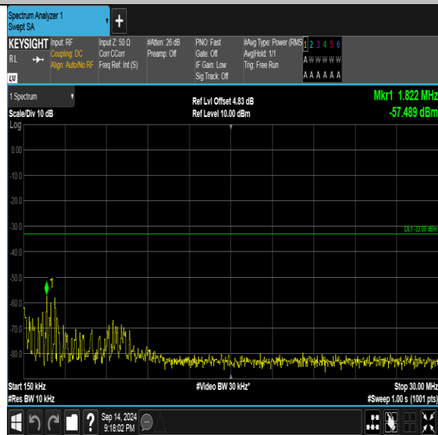
Band2-9262-2-0.15~30MHz-PASS
