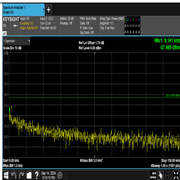
Band2-9538-2-0.009~0.15MHz-PASS
