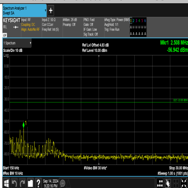
Band2-9262-3-0.15~30MHz-PASS
