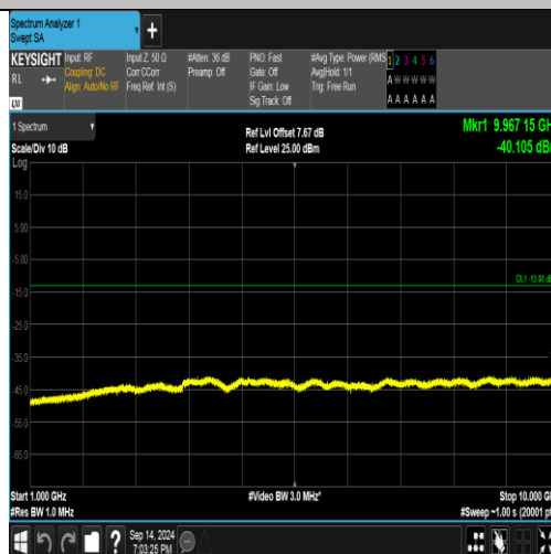
Band5-4233-1-1000~10000MHz-PASS
