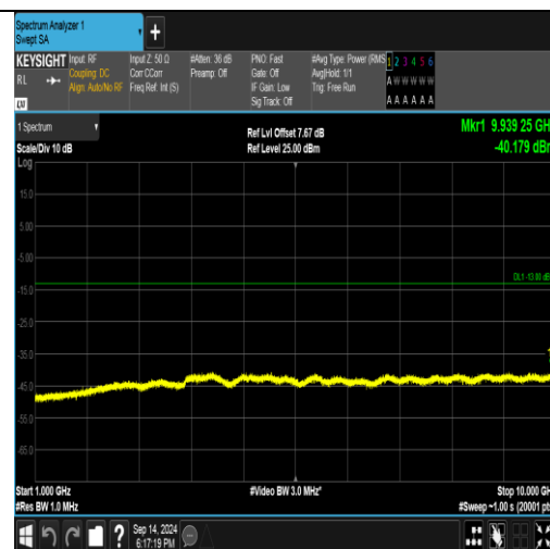
Band5-4182-1000~10000MHz-PASS
