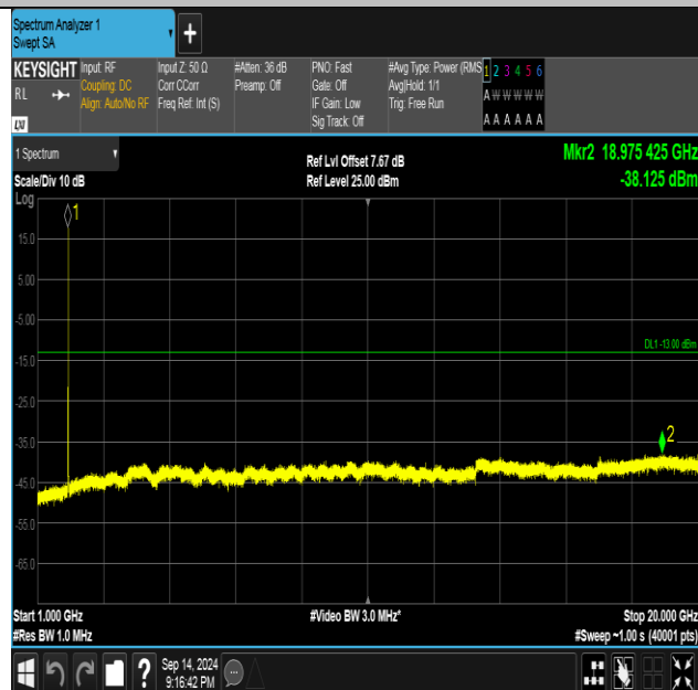
Band2-9400-1-1000~20000MHz-PASS
