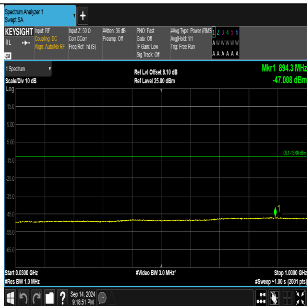
Band2-9400-2-30~1000MHz-PASS
