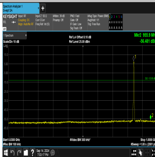
Band5-4233-1-30~1000MHz-PASS
