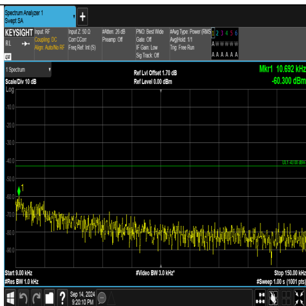
Band2-9262-3-0.009~0.15MHz-PASS
