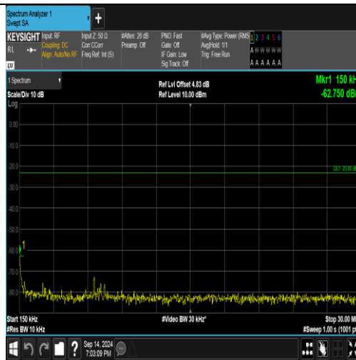
Band5-4233-1-0.15~30MHz-PASS
