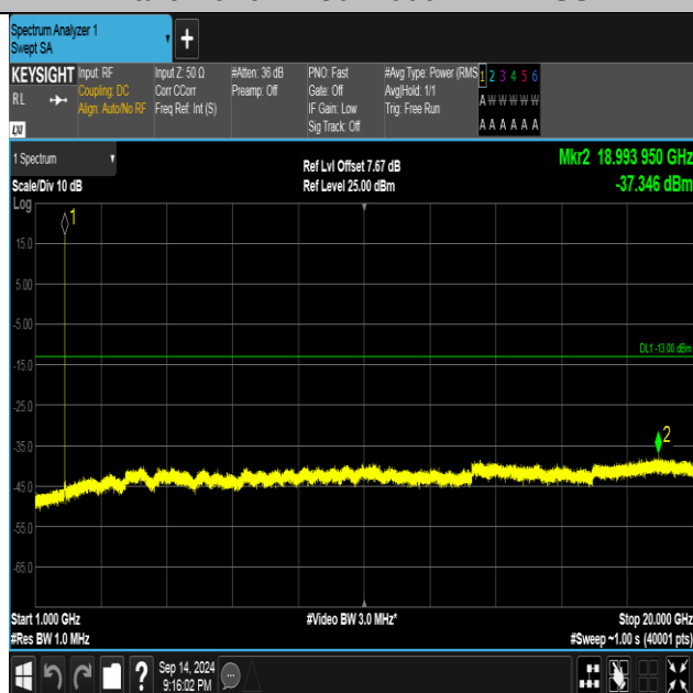
Band2-9262-1-1000~20000MHz-PASS
