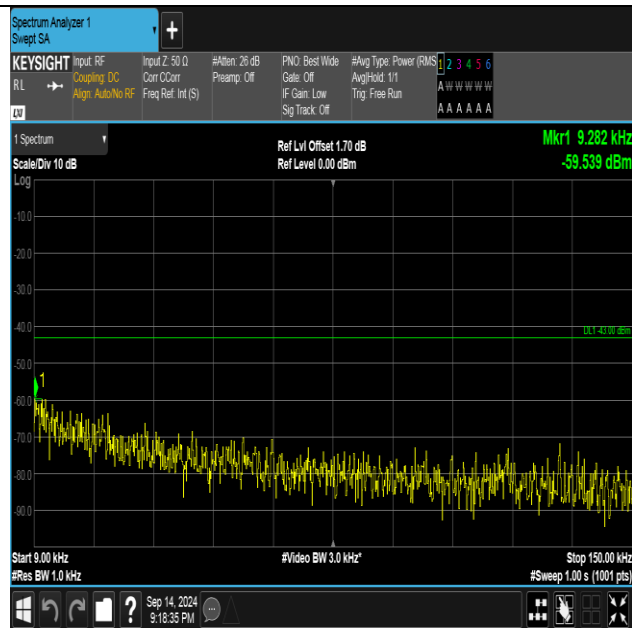
Band2-9400-2-0.009~0.15MHz-PASS
