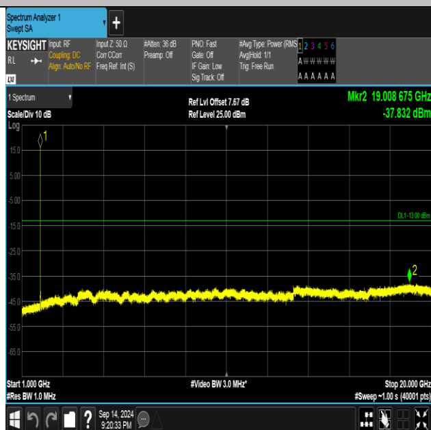
Band2-9262-3-1000~20000MHz-PASS
