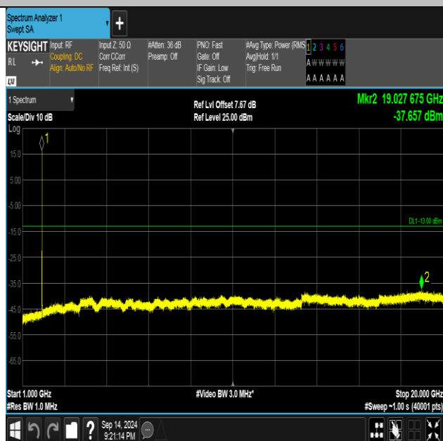
Band2-9400-3-1000~20000MHz-PASS
