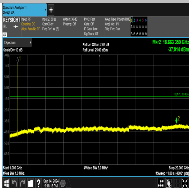
Band2-9262-2-1000~20000MHz-PASS
