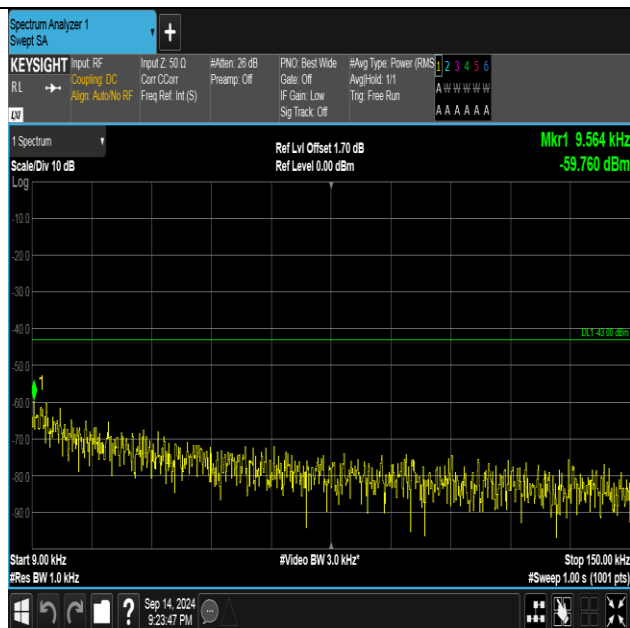
Band2-9538-4-0.009~0.15MHz-PASS
