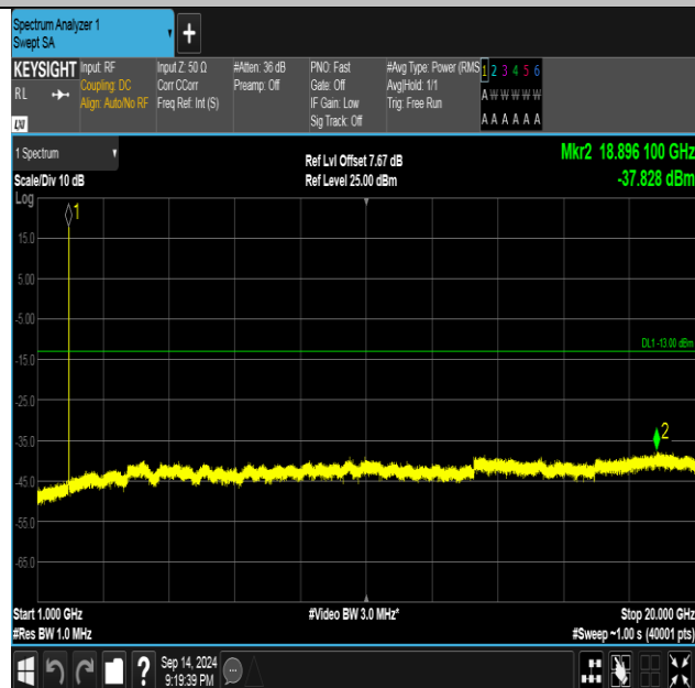
Band2-9538-2-1000~20000MHz-PASS
