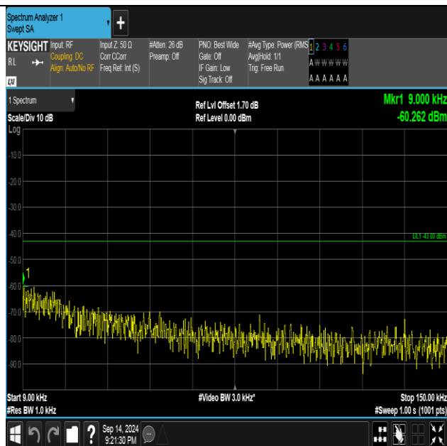
Band2-9538-3-0.009~0.15MHz-PASS
