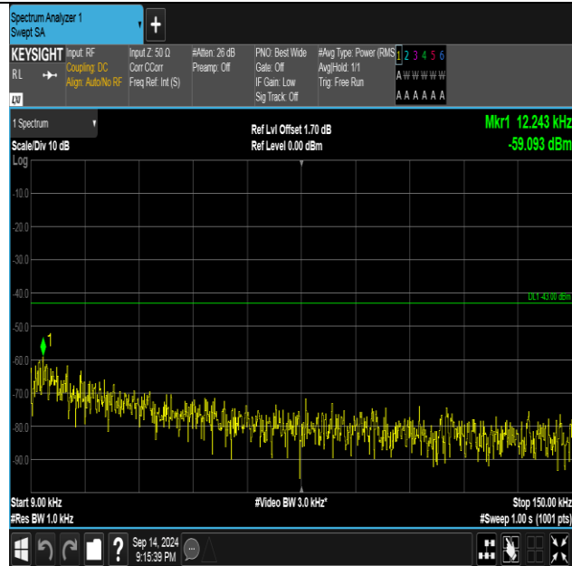
Band2-9262-1-0.009~0.15MHz-PASS
