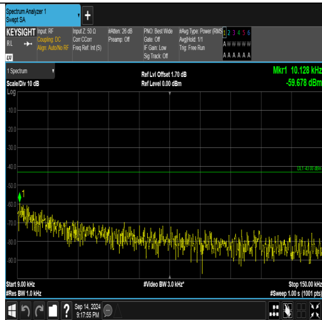
Band2-9262-2-0.009~0.15MHz-PASS
