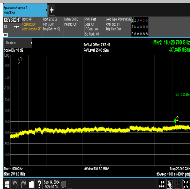
Band2-9538-4-1000~20000MHz-PASS
