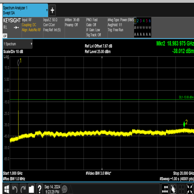
Band2-9400-4-1000~20000MHz-PASS
