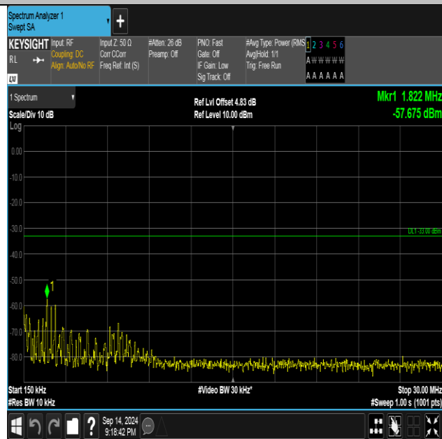
Band2-9400-2-0.15~30MHz-PASS
