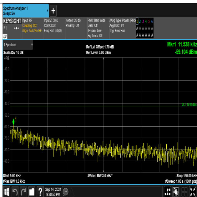
Band2-9400-3-0.009~0.15MHz-PASS
