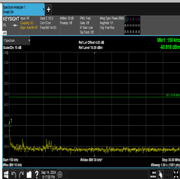
Band2-9538-1-0.15~30MHz-PASS
