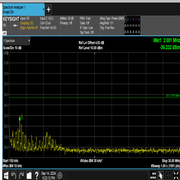
Band2-9400-4-0.15~30MHz-PASS
