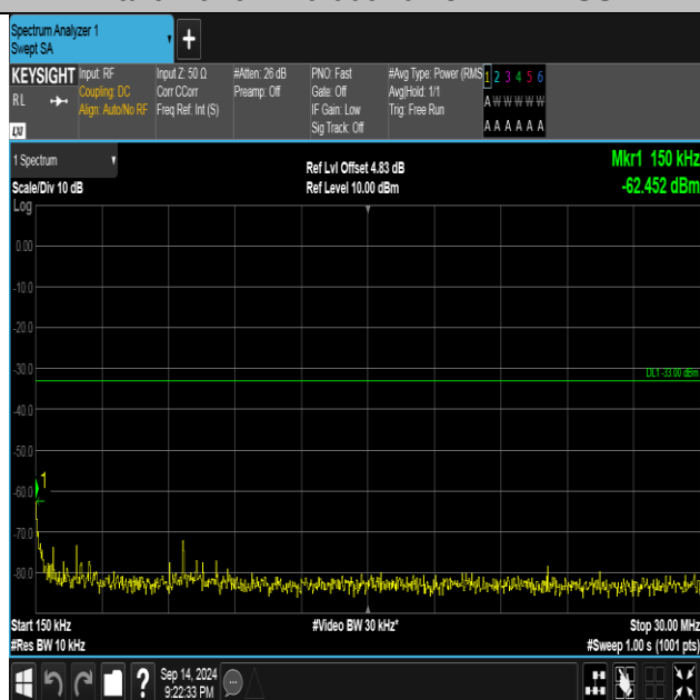
Band2-9262-4-0.15~30MHz-PASS
