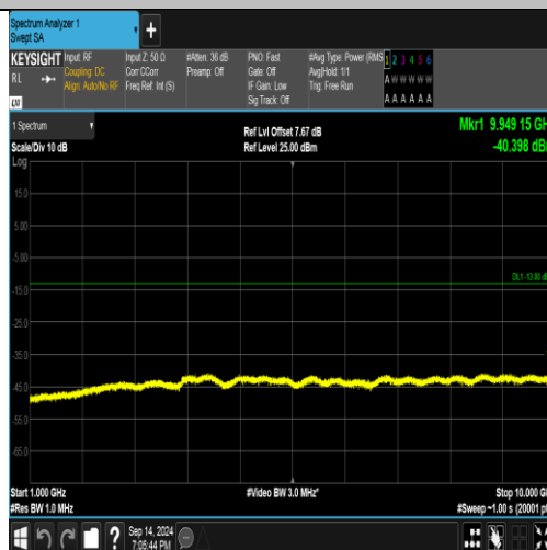
Band5-4233-2-1000~10000MHz-PASS
