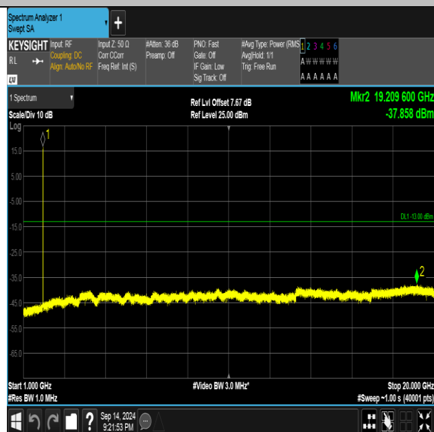
Band2-9538-3-1000~20000MHz-PASS
