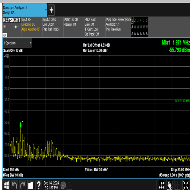
Band2-9538-3-0.15~30MHz-PASS
