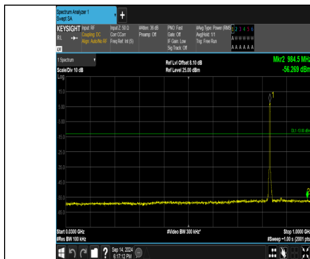
Band5-4182-30~1000MHz-PASS
