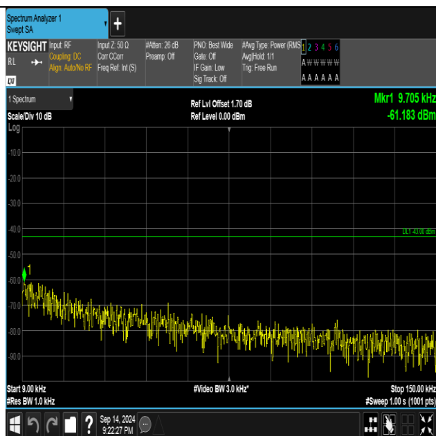
Band2-9262-4-0.009~0.15MHz-PASS
