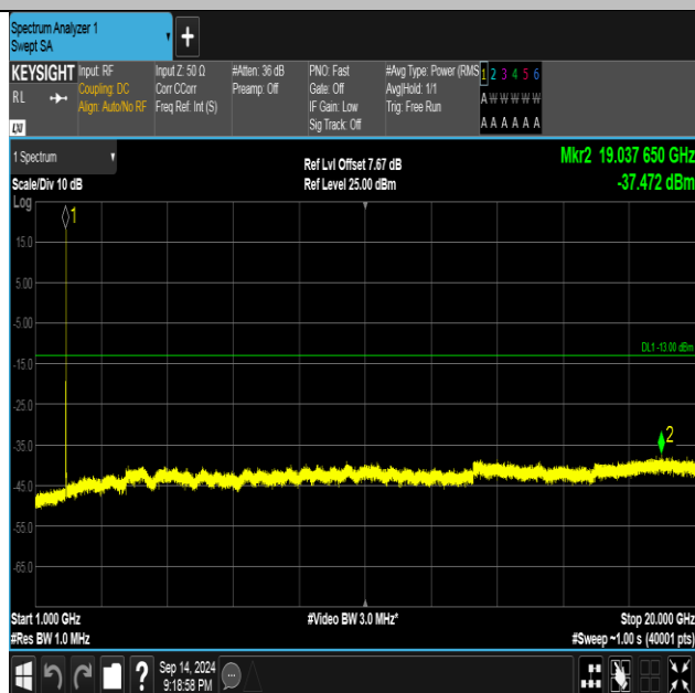
Band2-9400-2-1000~20000MHz-PASS
