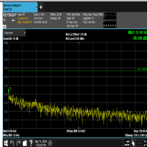
Band5-4233-1-0.009~0.15MHz-PASS
