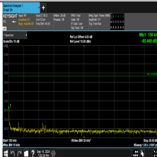
Band5-4182-1-0.15~30MHz-PASS
