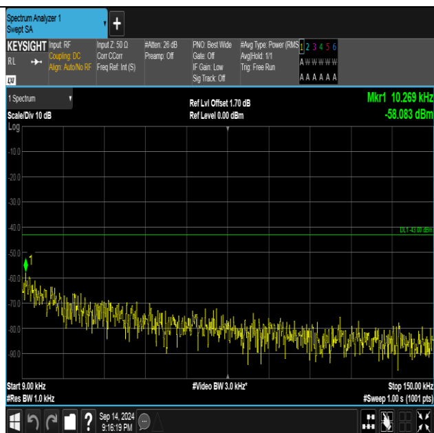
Band2-9400-1-0.009~0.15MHz-PASS
