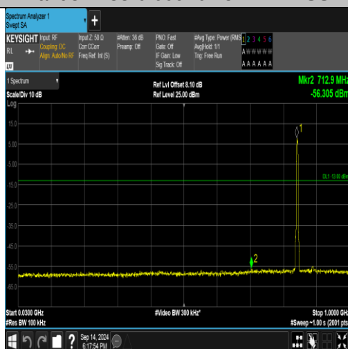
Band5-4233-30~1000MHz-PASS
