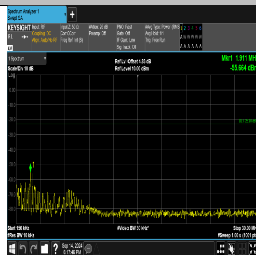
Band5-4233-0.15~30MHz-PASS
