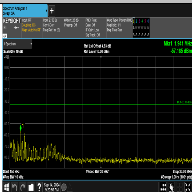
Band2-9400-3-0.15~30MHz-PASS
