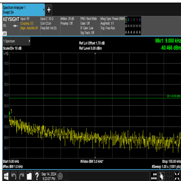
Band2-9400-4-0.009~0.15MHz-PASS
