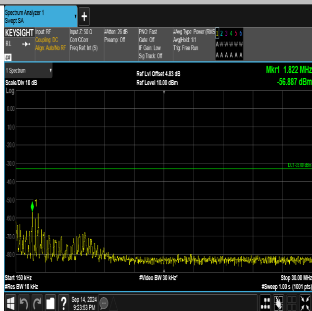
Band2-9538-4-0.15~30MHz-PASS
