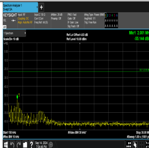
Band5-4182-2-0.15~30MHz-PASS
