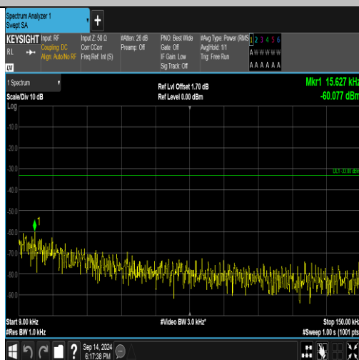
Band5-4233-0.009~0.15MHz-PASS
