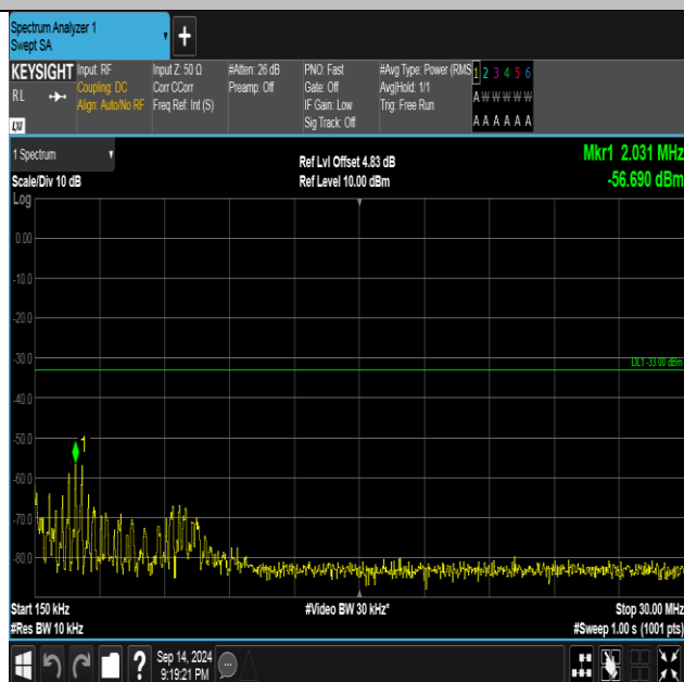
Band2-9538-2-0.15~30MHz-PASS
