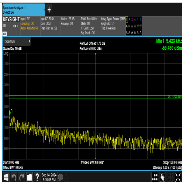
Band2-9538-1-0.009~0.15MHz-PASS
