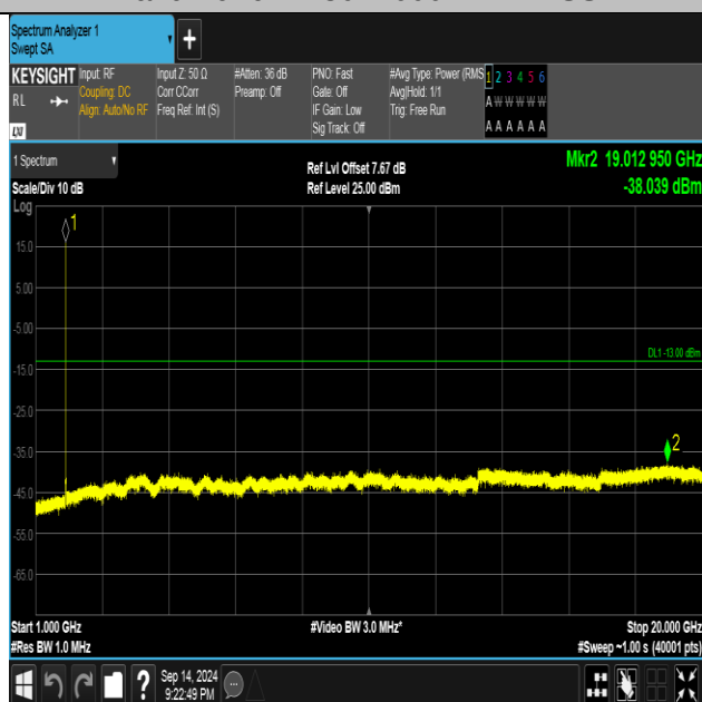
Band2-9262-4-1000~20000MHz-PASS
