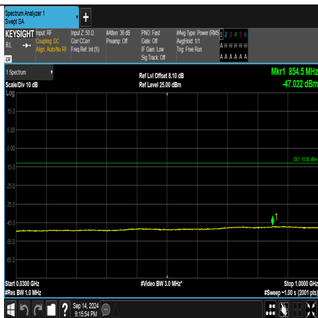
Band2-9262-1-30~1000MHz-PASS
