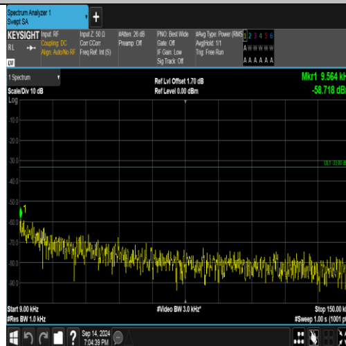
Band5-4182-2-0.009~0.15MHz-PASS
