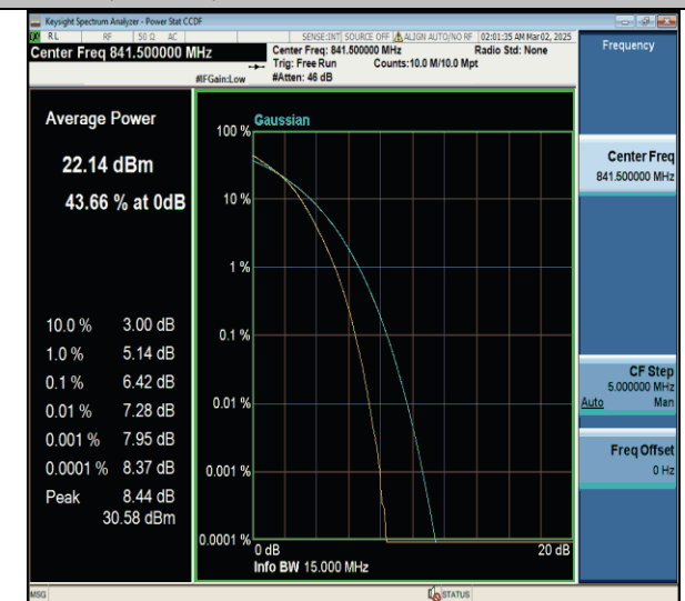
Band26(824-849)-15MHz-16QAM-26965-75RB#0-PASS
