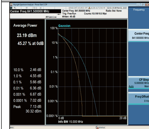
Band26(824-849)-15MHz-QPSK-26965-75RB#0-PASS
