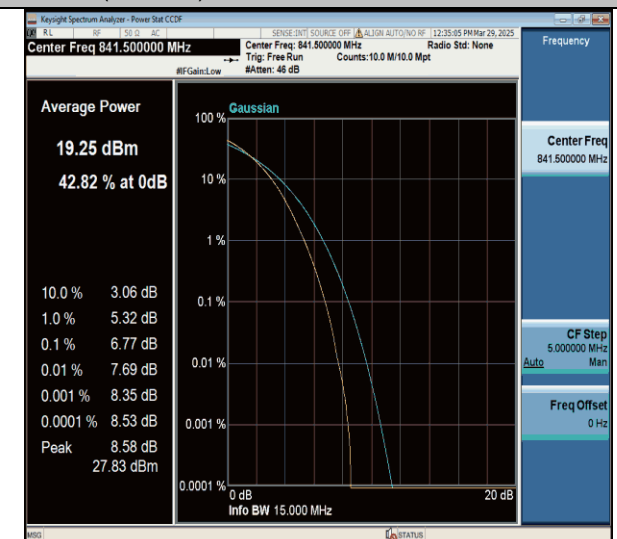
Band26(824-849)-15MHz-256QAM-26965-75RB#0-PASS
