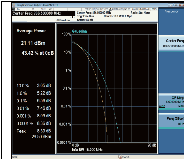
Band26(824-849)-15MHz-64QAM-26915-75RB#0-PASS
