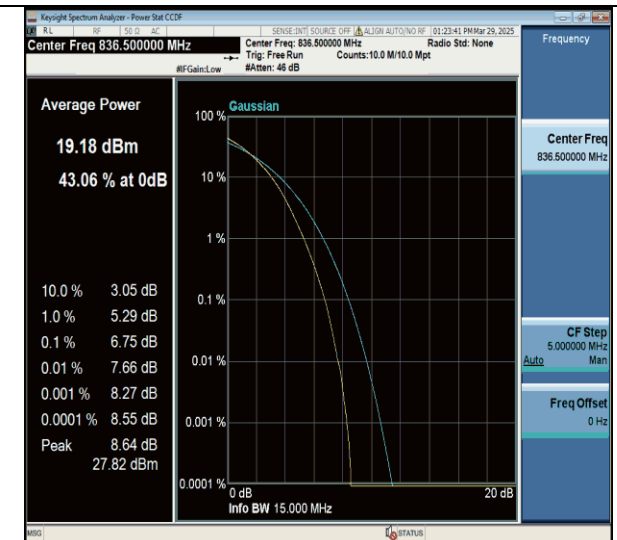
Band26(824-849)-15MHz-256QAM-26915-75RB#0-PASS
