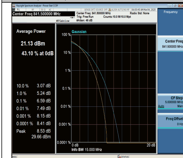
Band26(824-849)-15MHz-64QAM-26965-75RB#0-PASS
