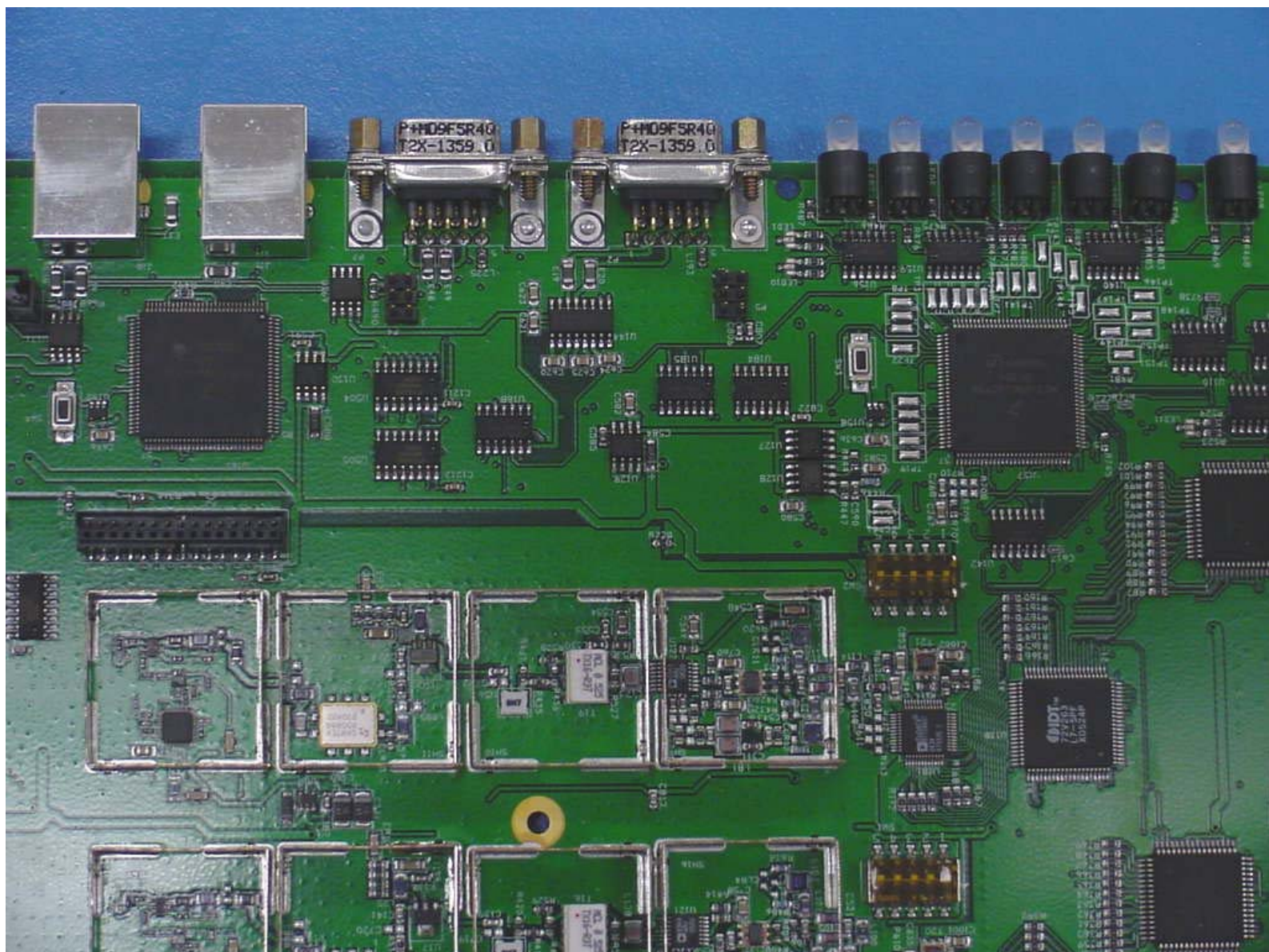
Digivance LRCS 1900 MHz Host Board Top View 7
