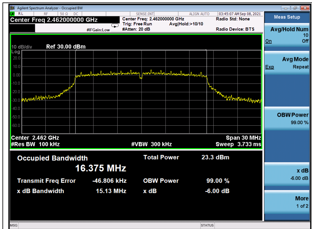
(Channel 11, 802.11g)
