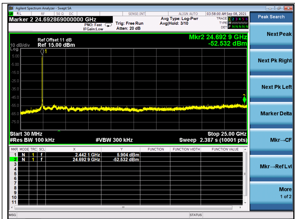
(30MHz to 25GHz, Channel 6, 802.11g)
