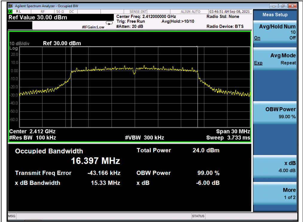
(Channel 1, 802.11g)
