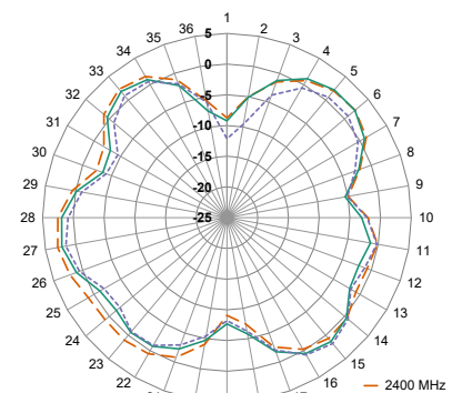
XY-Plane Gain
