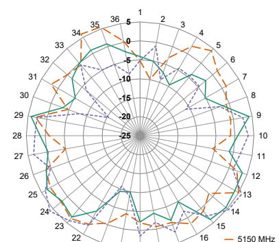
XY-Plane Gain
